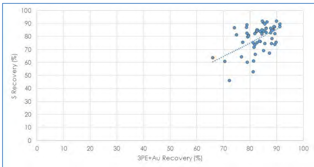
Figure 13.26 Variability Testwork Sulfur Recovery as a Function of 3PE+Au Recovery
