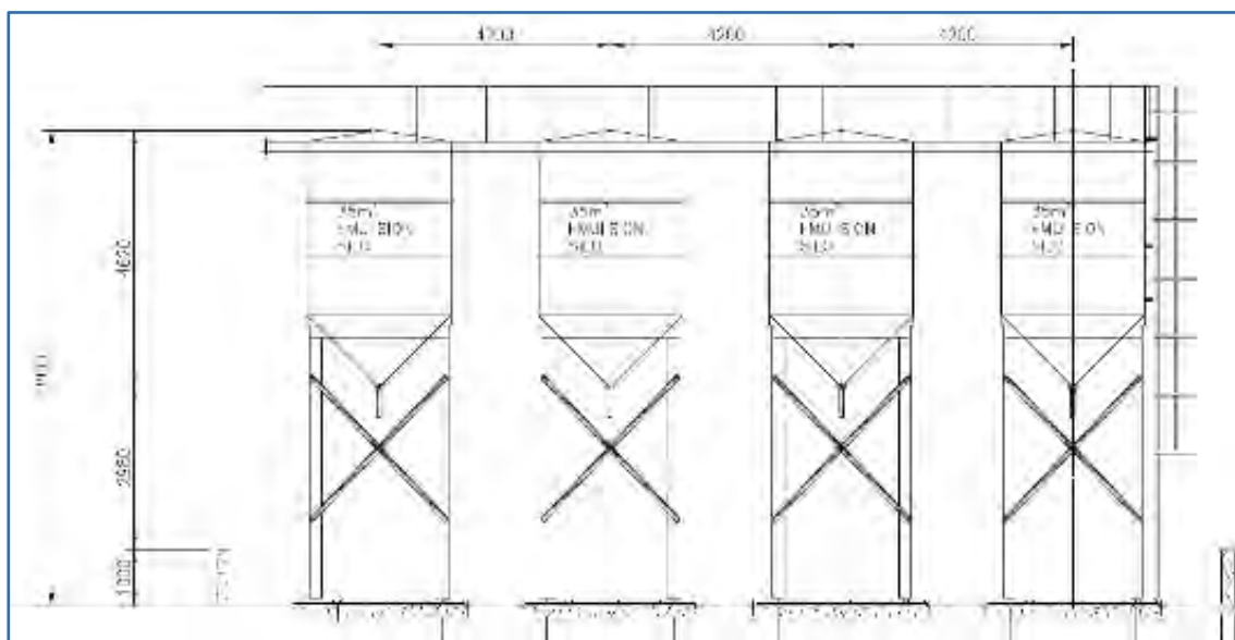
Figure 18.25 Emulsion Storage Tanks – Section View
