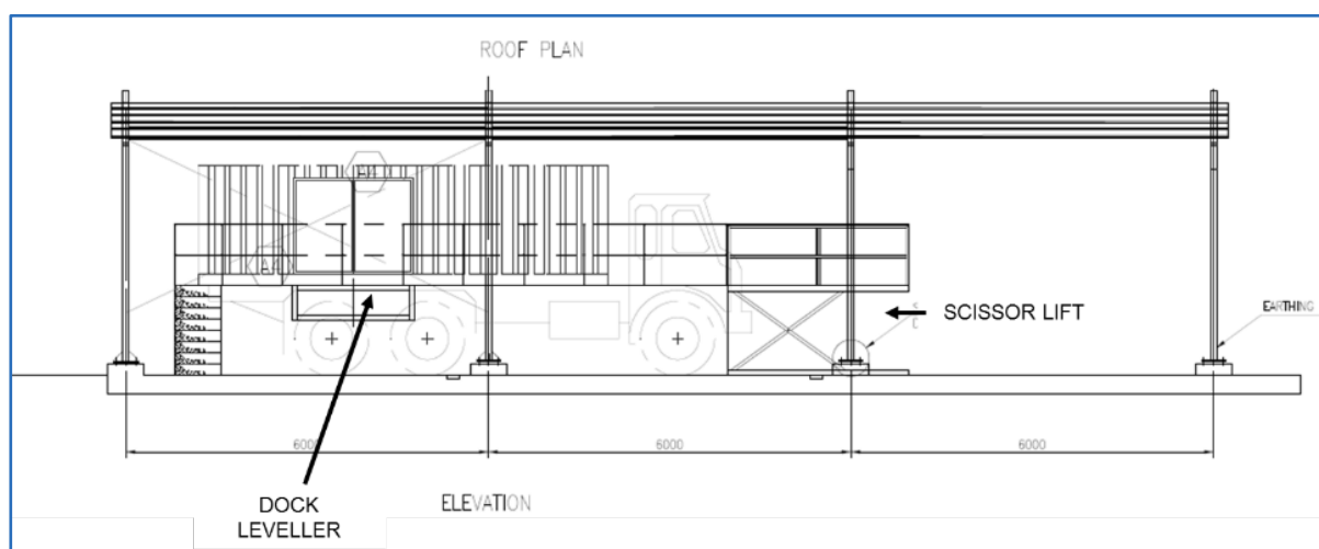
Figure 18.28 Explosives Offloading Facility – Side View
