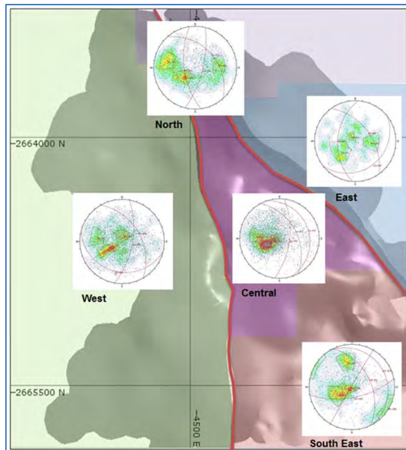
Figure 16.5 Stereographic Projections per Structural Domain
