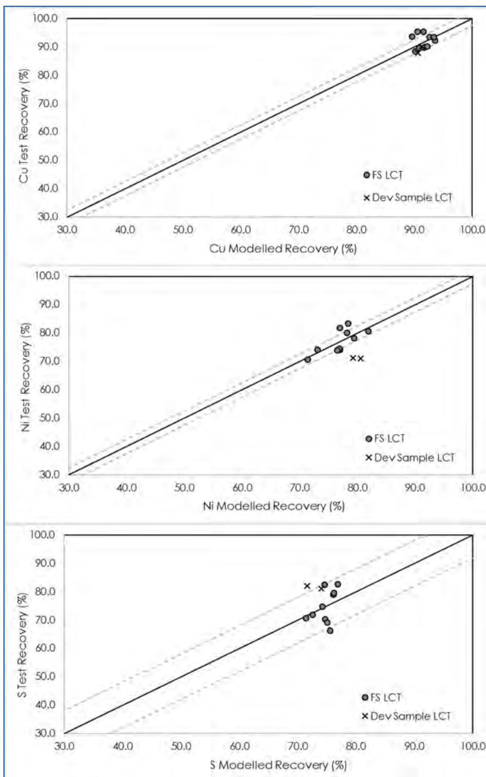
Figure 13.37 Copper, Nickel and Sulfur Recovery Model Verification
