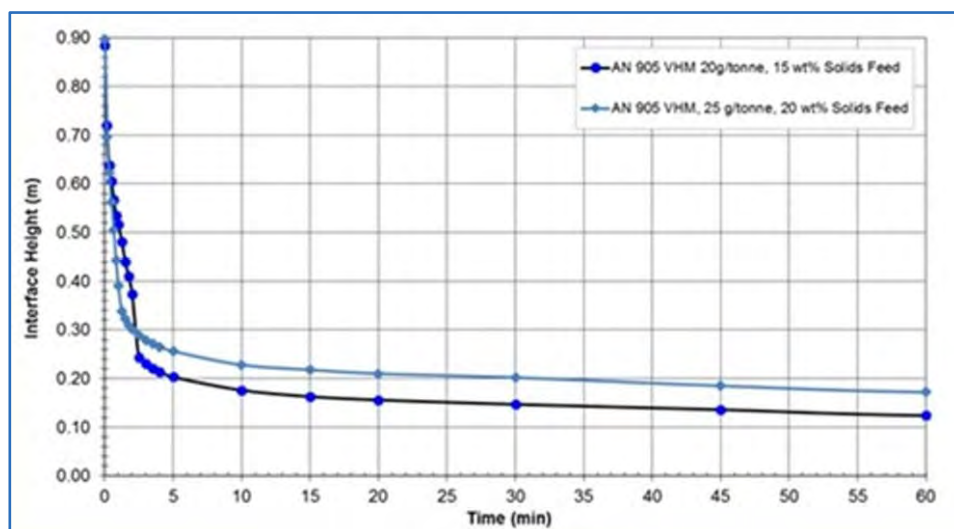
Figure 13.31 Settling Curve, 15–20% Solids Feed, 20–25 g/t
