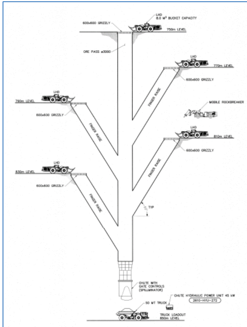
Figure 16.42 Sublevel Loading and Transfer Arrangement
