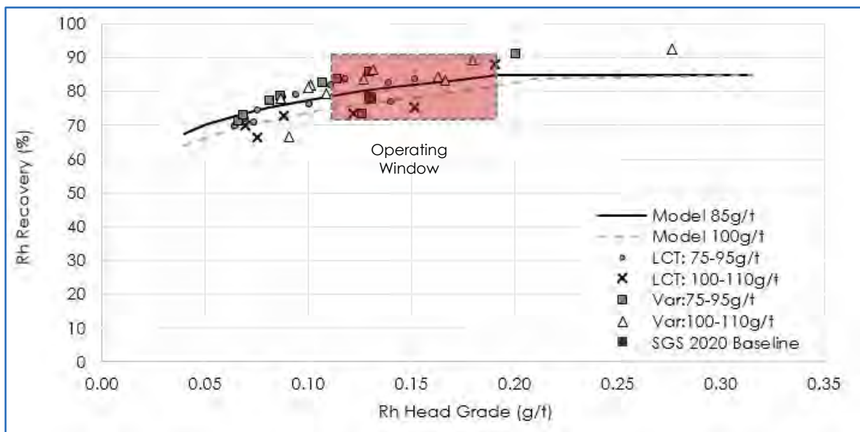
Figure 13.41 Rhodium Recovery as a Function of Feed Grade and Targeted Concentrate Grade
