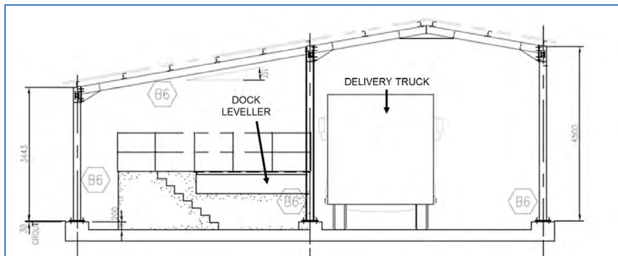
Figure 18.27 Explosives Offloading Facility – Front View
