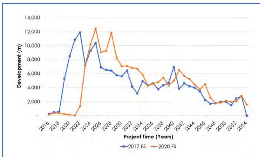
Figure 16.37 Waste Development
