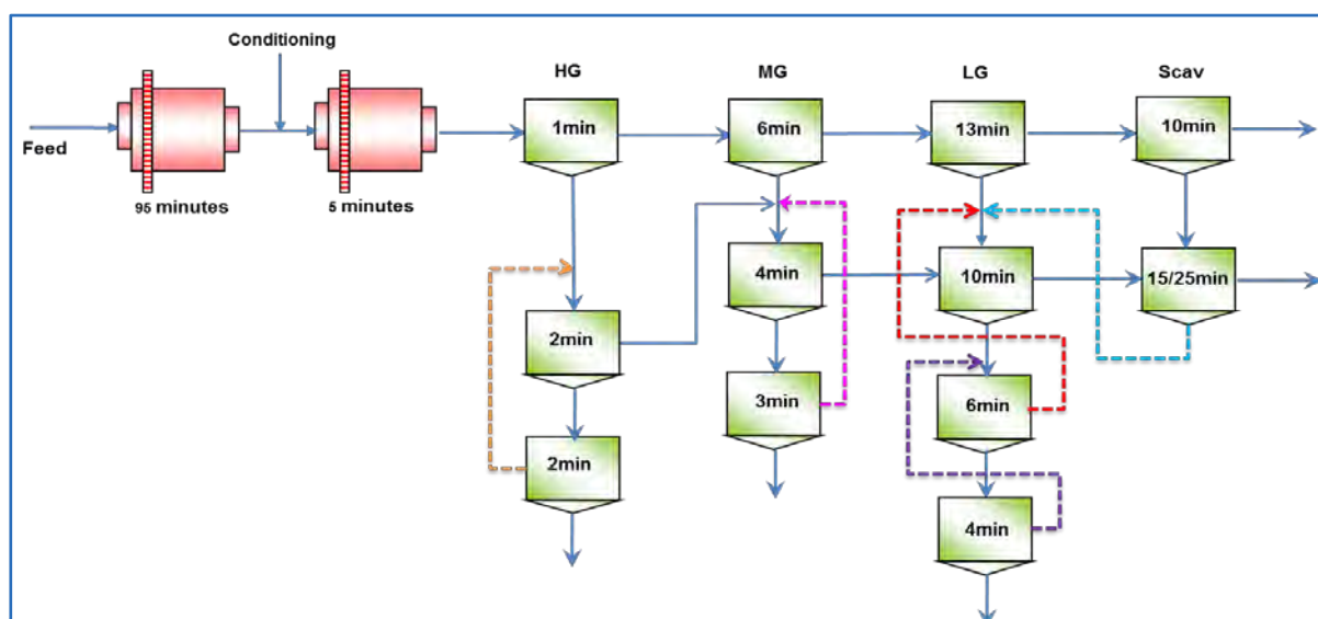
Figure 13.27 Development Testing Locked Cycle Test Flow Sheet 1 (Flow Sheet 1)
