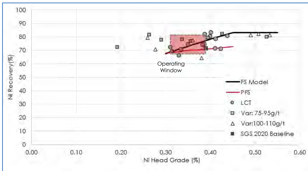
Figure 13.44 Nickel Recovery as a Function of Feed Grade
