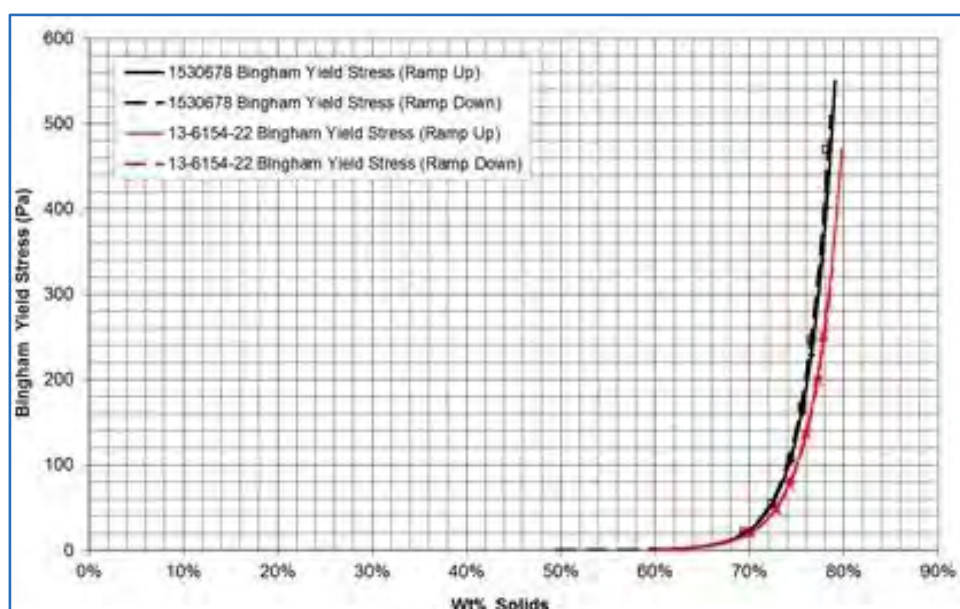
Figure 16.19 Bingham Yield Stress Comparison
