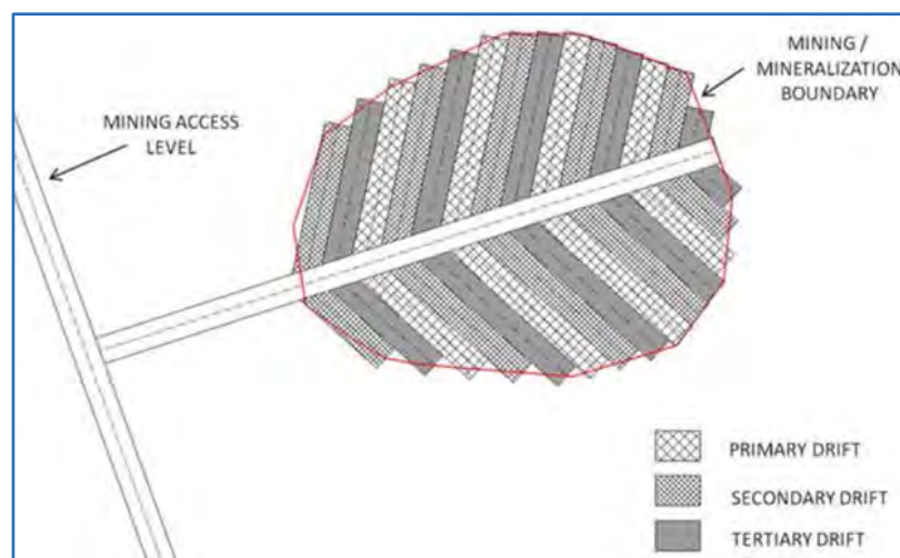
Figure 16.14 Typical Drift-and-Fill Mining Level Layout
