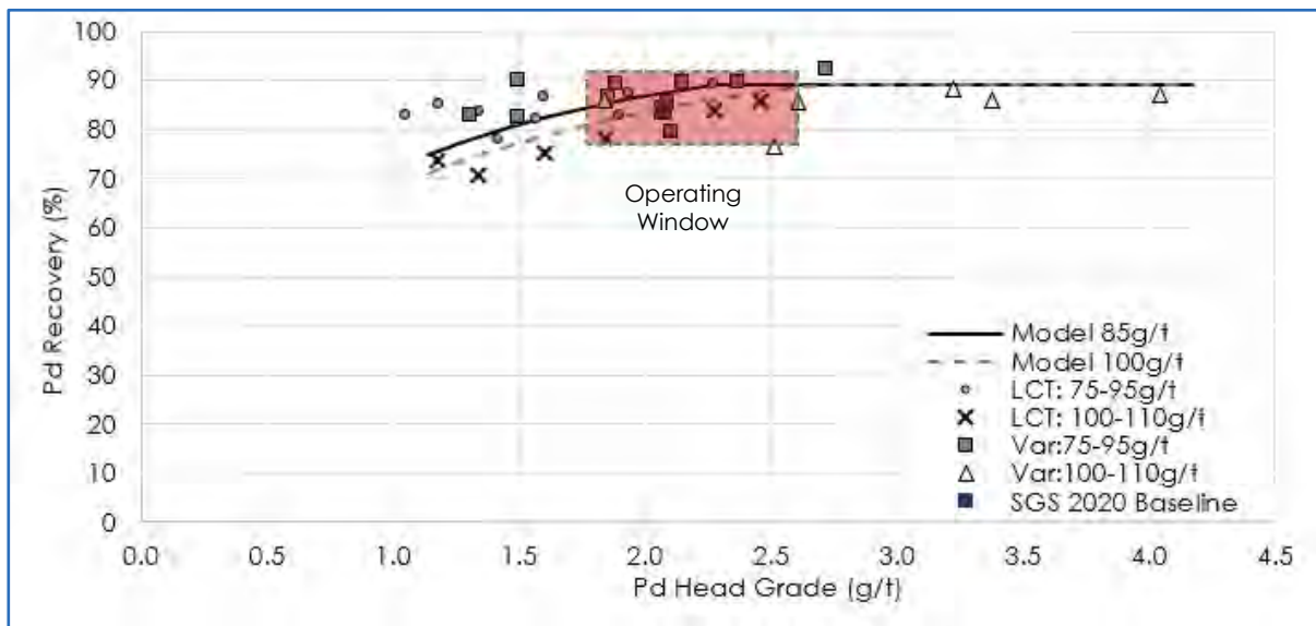
Figure 13.40 Palladium Recovery as a Function of Feed Grade and Targeted Concentrate Grade
