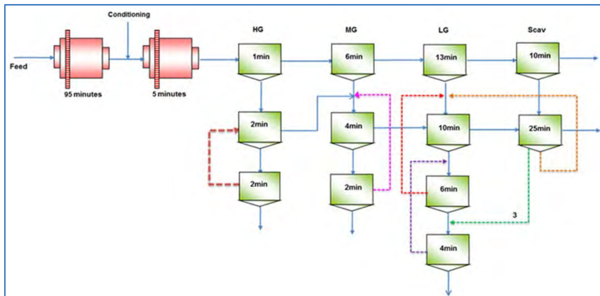
Figure 17.2 Optimised Flotation Flow Sheet as Derived from Testwork
