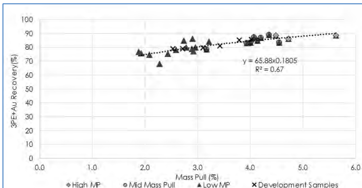
Figure 13.34 3PE+Au Recovery as A Function of Mass Pull
