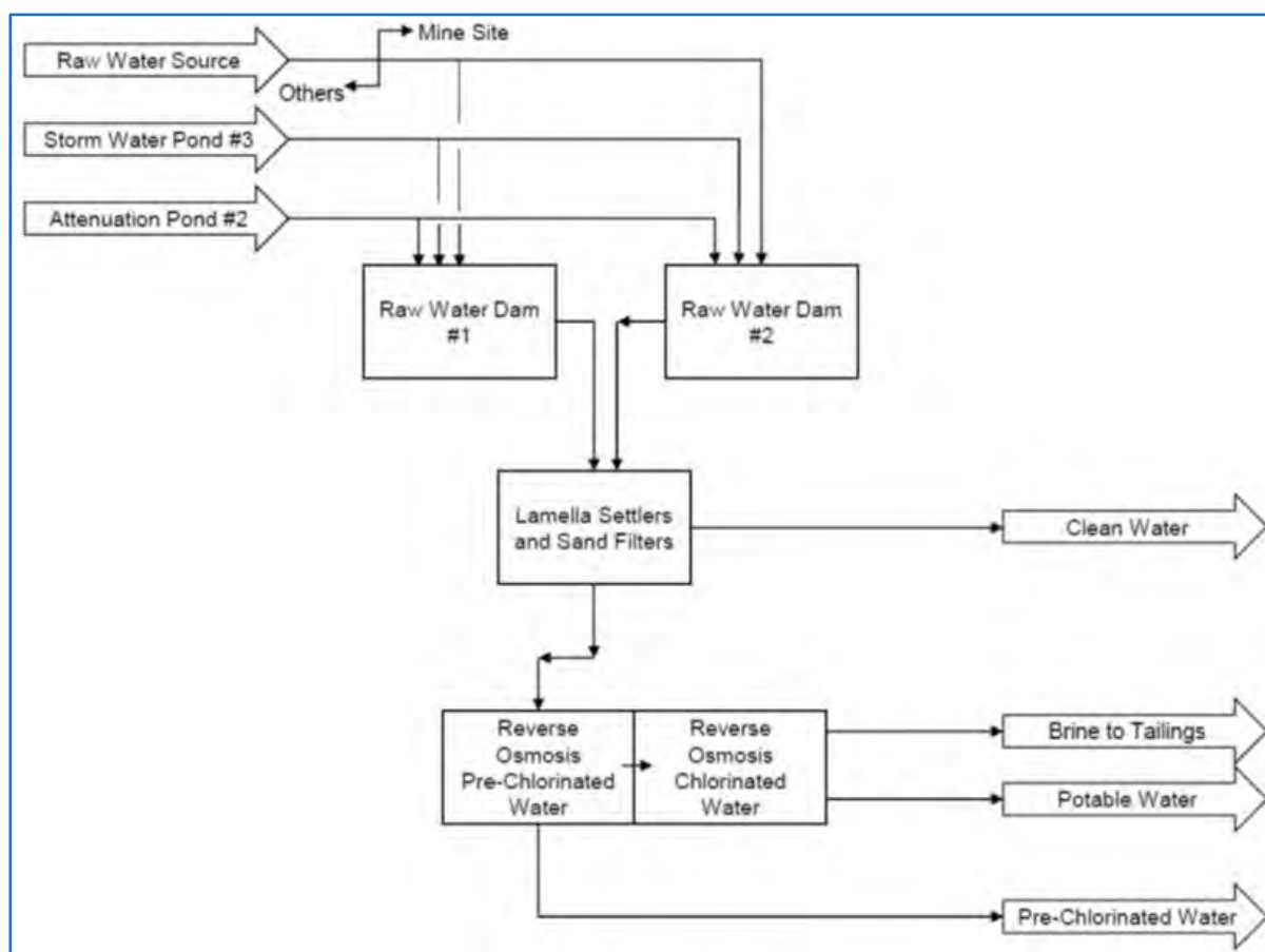
Figure 18.18 Schematic Showing Water Treatment Works
