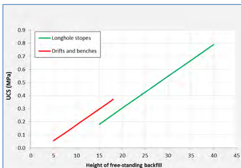
Figure 16.6 Proposed Backfill Strength Requirements
