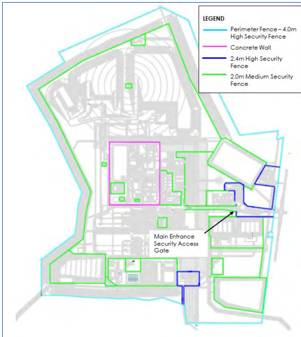
Figure 18.34 Mine Area Perimeter and Internal Fence Lines
