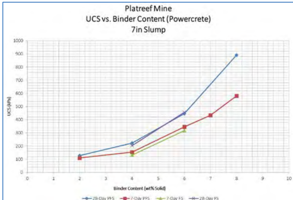
Figure 16.21 UCS vs. Binder Content – 7" (178 mm) Slump
