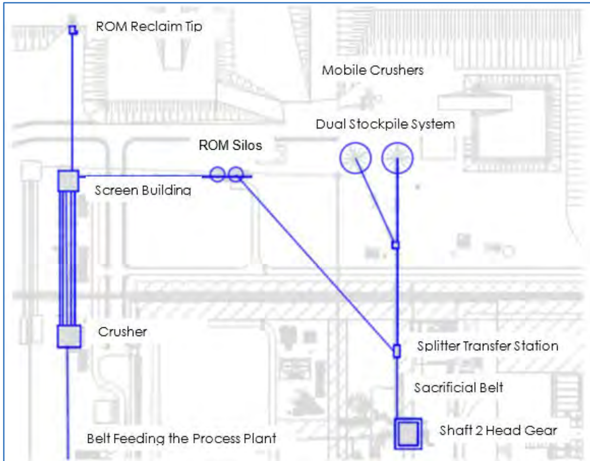
Figure 18.22 Surface Rock Handling
