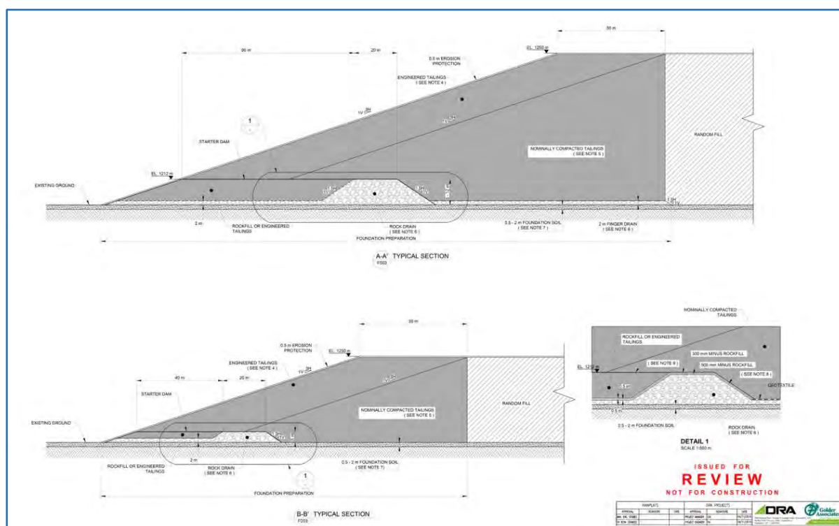
Figure 18.8 Dry-Stacking TSF
