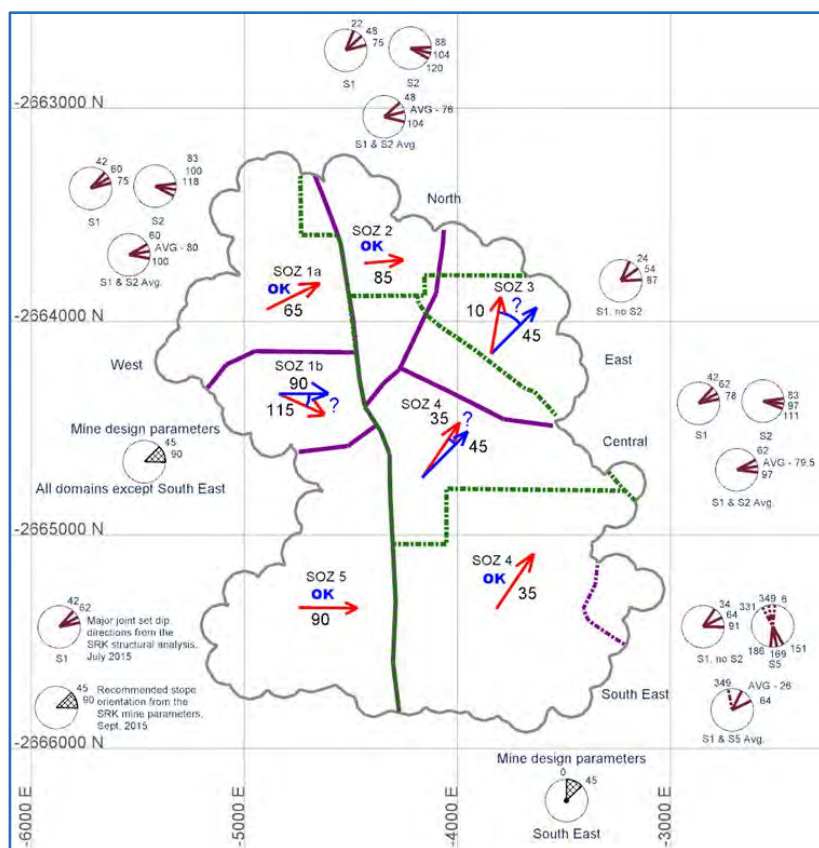
Figure 16.13 Possible Transverse Stope Orientation Conflicts
