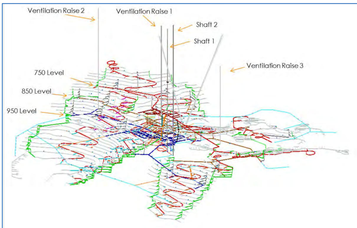
Figure 1.4 Mine Access Layout
