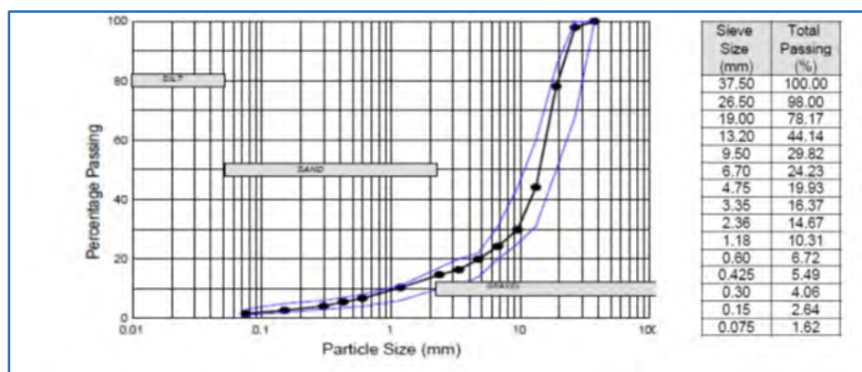
Figure 16.18 Waste Rock Sample Gradation for Tests
