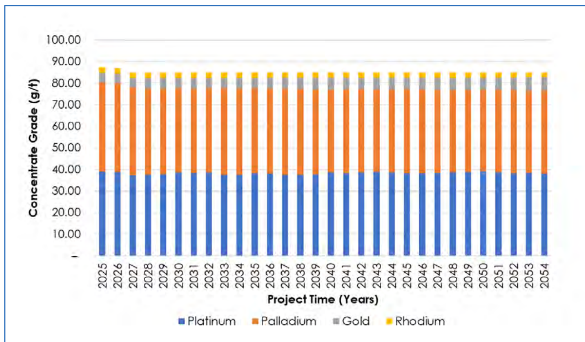
Figure 13.47 Modelled Life-of-Mine Concentrate Grade Profile
