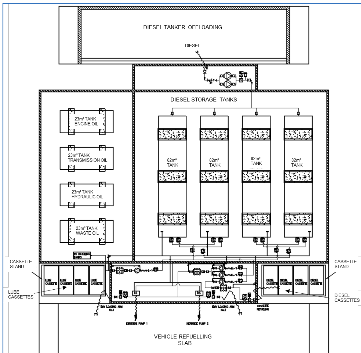
Figure 18.30 Surface Fuel and Lube Receiving, Storage and Dispensing Depot – Diesel Receiving and Dispensing
