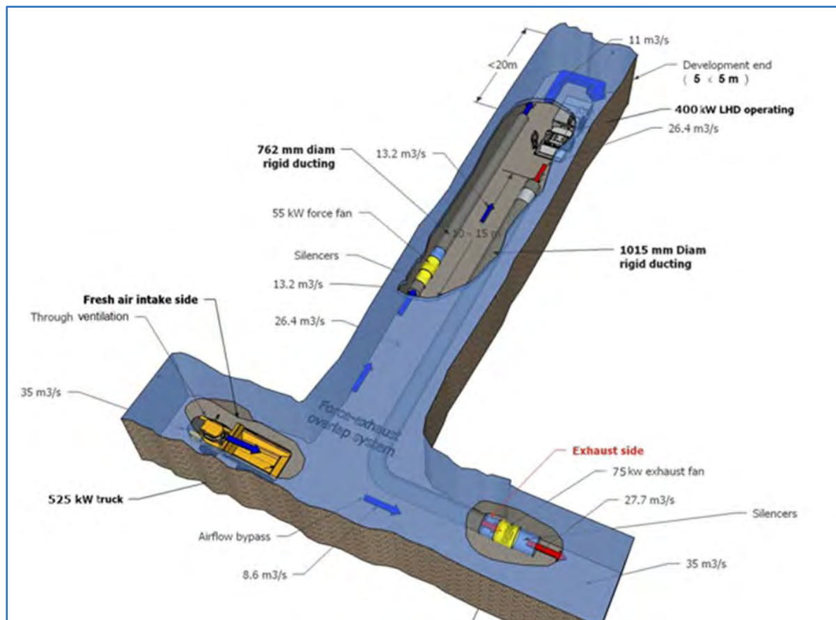
Figure 16.47 General Ventilation Arrangement and Layout
