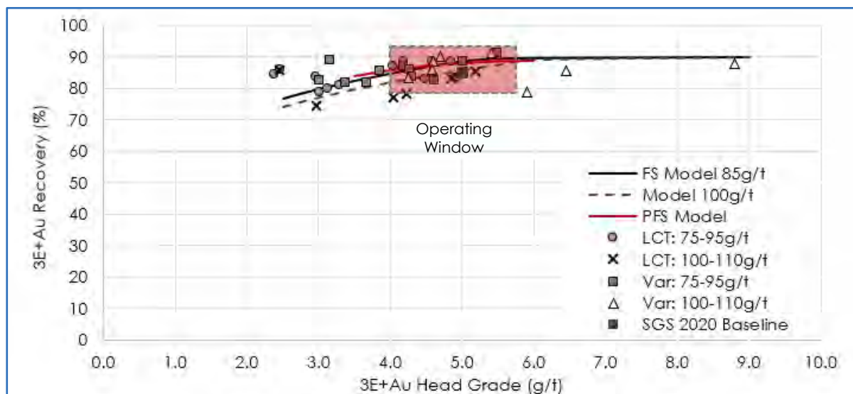
Figure 13.38 3PE+Au Recovery as a Function of Feed Grade and Targeted Concentrate Grade
