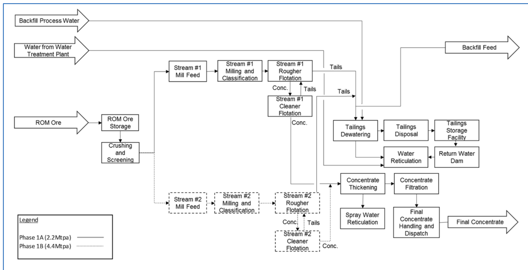
Figure 17.1 Concentrator Flow Sheet
