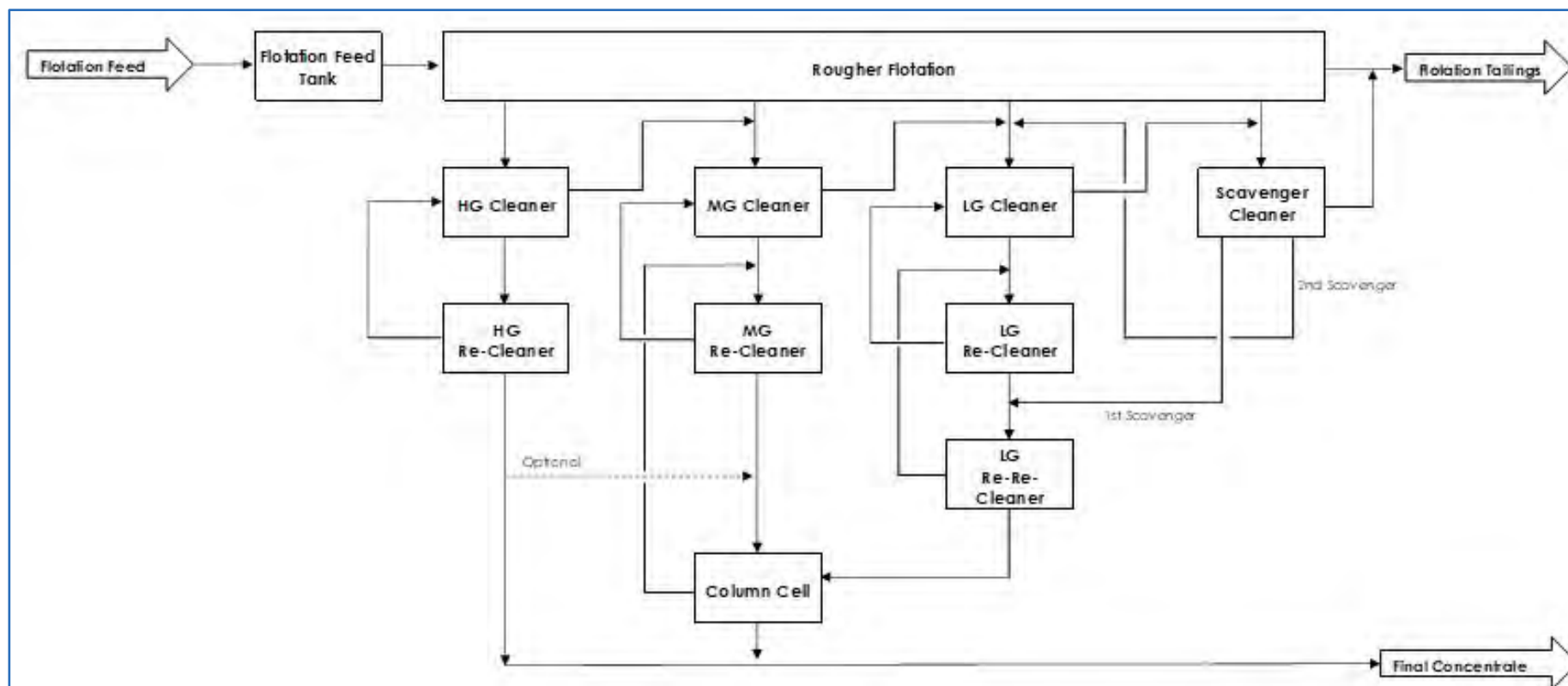
Figure 17.3 Flotation Circuit High Level Flow Sheet
