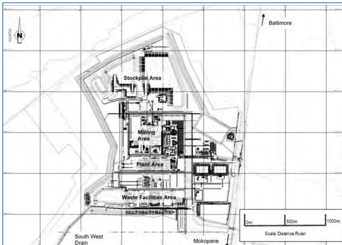
Figure 18.7 Mine Plot Plan
