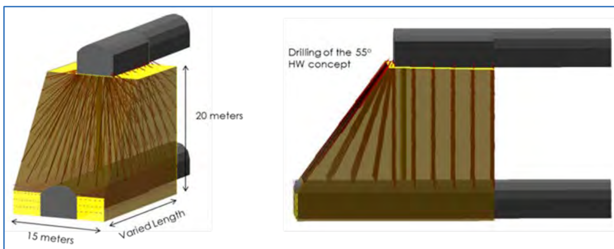
Figure 16.7 Typical Transverse Drill Design
