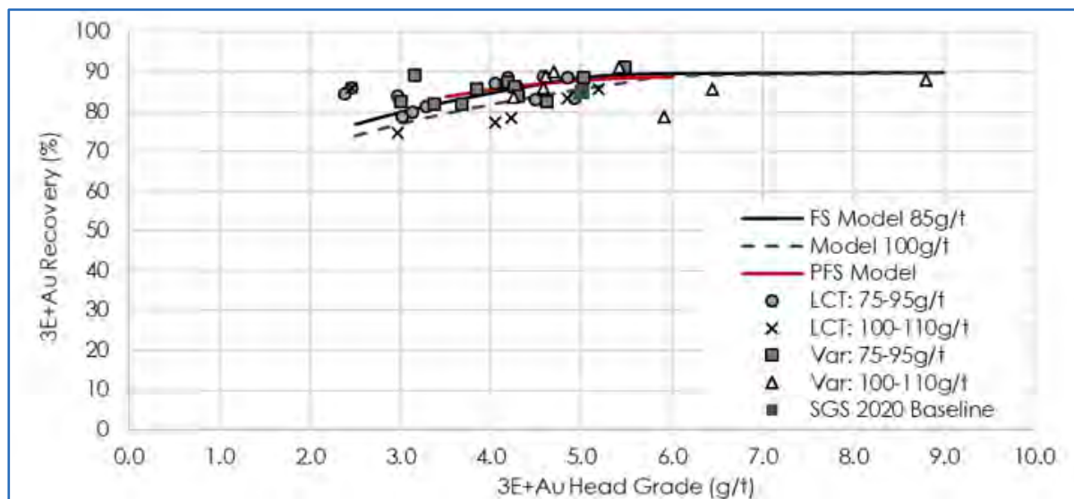
Figure 13.1 3PE+Au Recovery as a Function of Concentrate Grade
