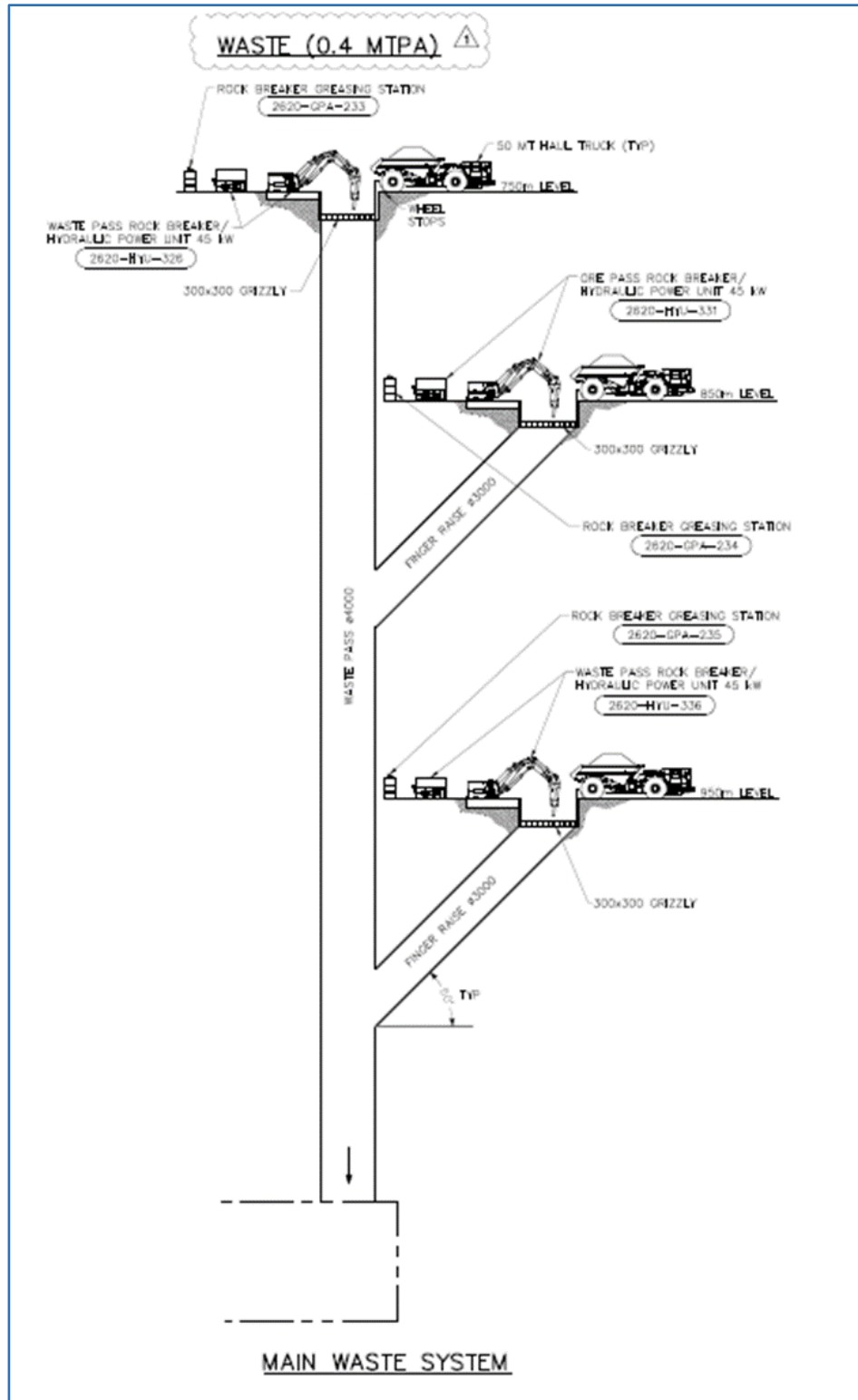
Figure 16.46 Waste Pass System
