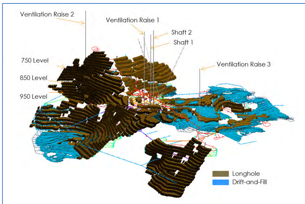
Figure 1.5 Elevated View of Mining Areas by Method
