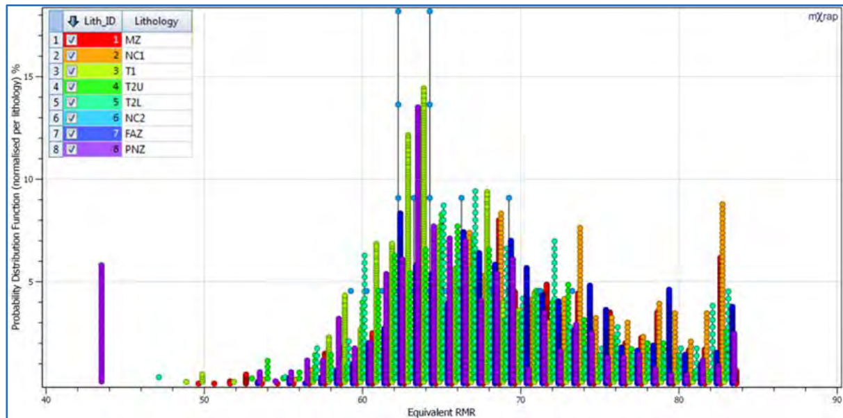
Figure 16.3 Pdfs of RMR Values (Determined From Q') for All Stratigraphic Units
