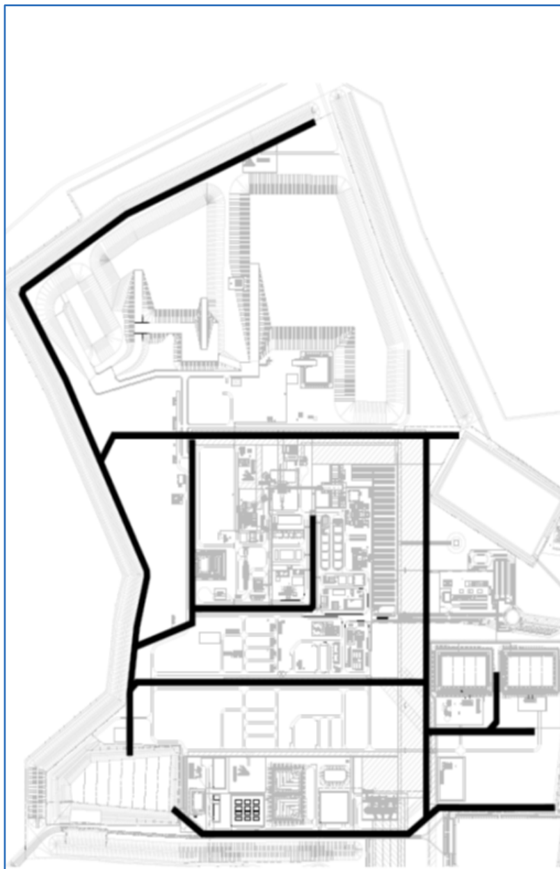
Figure 18.15 Stormwater Run Off Drains
