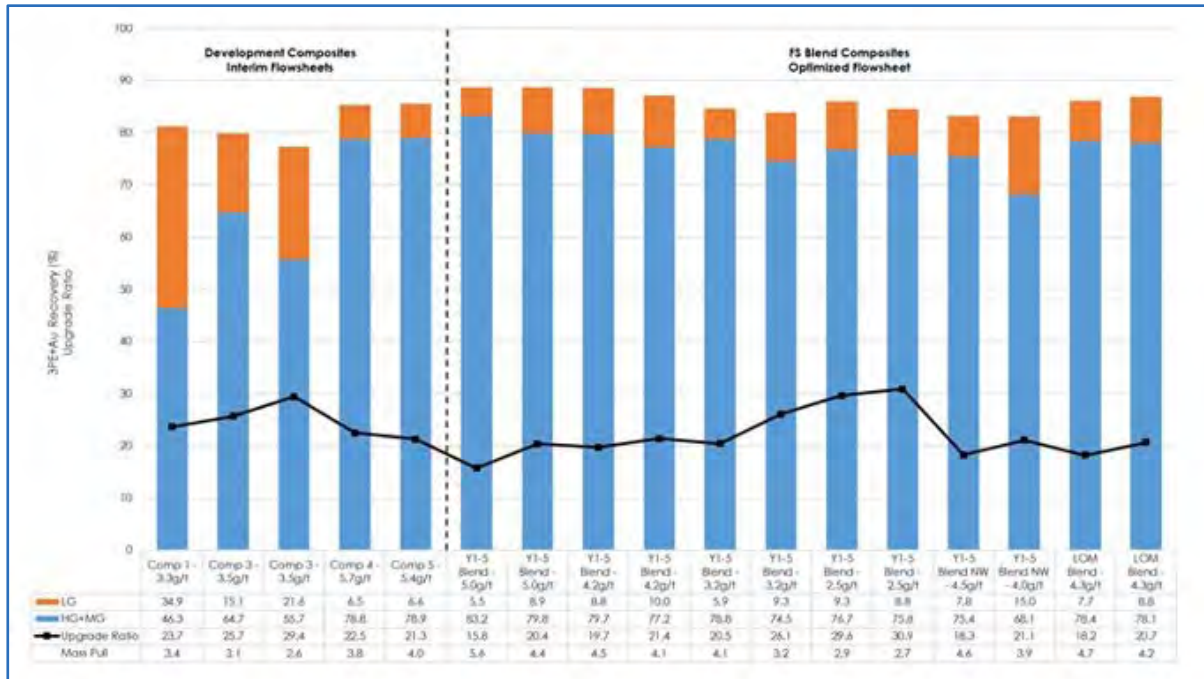
Figure 13.30 Summary of Locked Cycle Test Results
