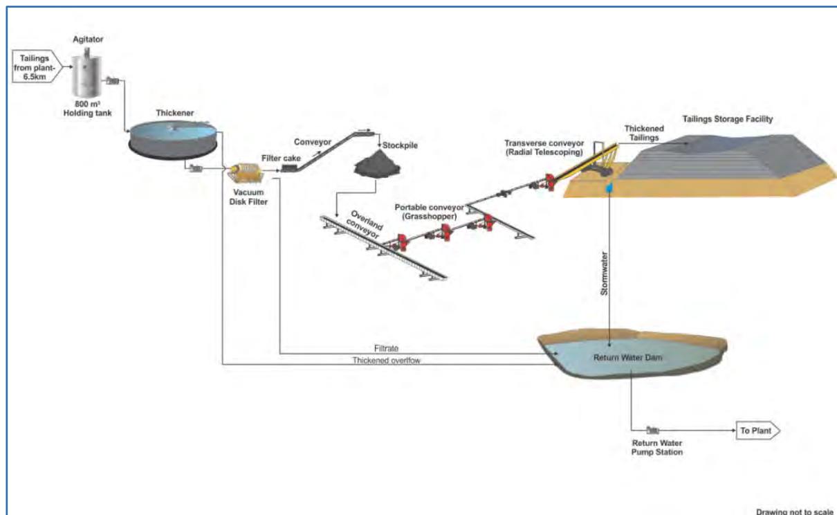
Figure 18.9 Dry-Stacking Tails System
