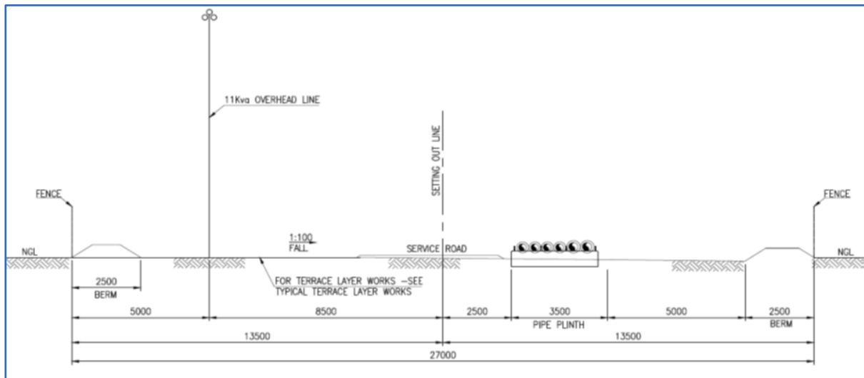
Figure 18.20 Tailings Servitude Section
