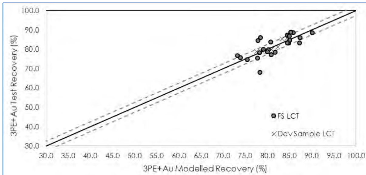
Figure 13.35 Combine PGE (3PE+Au) Recovery Model Verification
