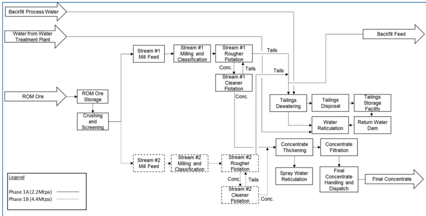
Figure 1.7 Concentrator Flow Sheet
