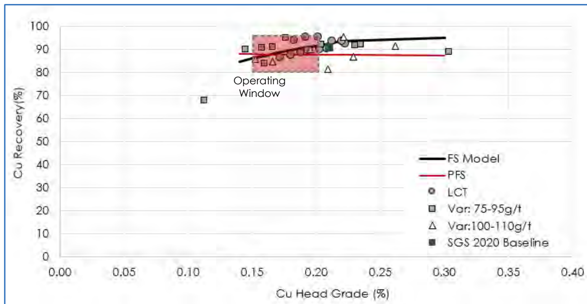
Figure 13.43 Copper Recovery as a Function of Feed Grade
