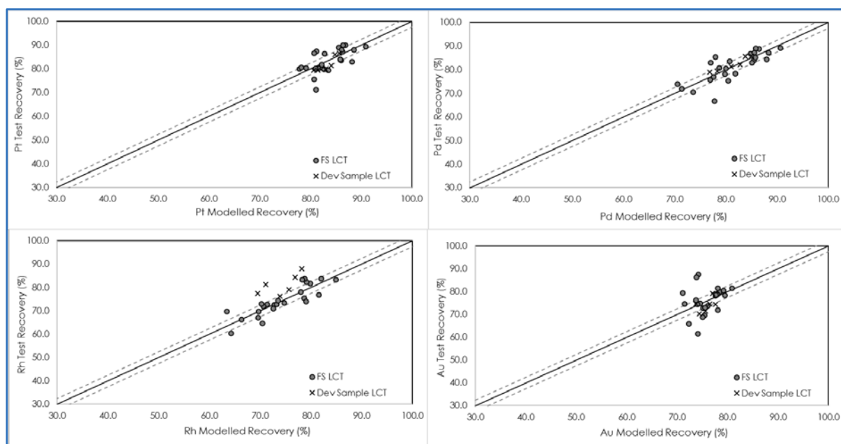
Figure 13.36 Individual, Pt, Pd, Rh and Au Recovery Model Verification
