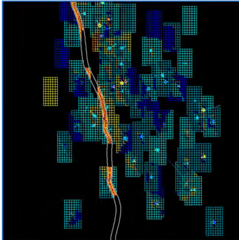
Figure 16.4 Geotechnical Block Model
