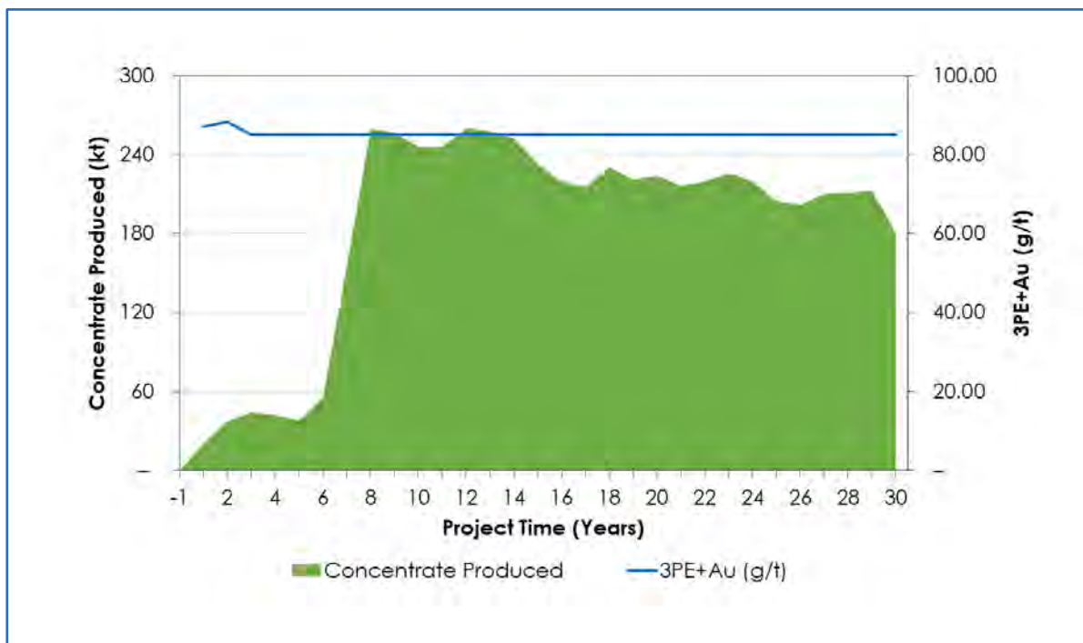
Figure 24.8 Platreef 2020 PEA Estimated Concentrate Produced and 3PE+Au Grade
