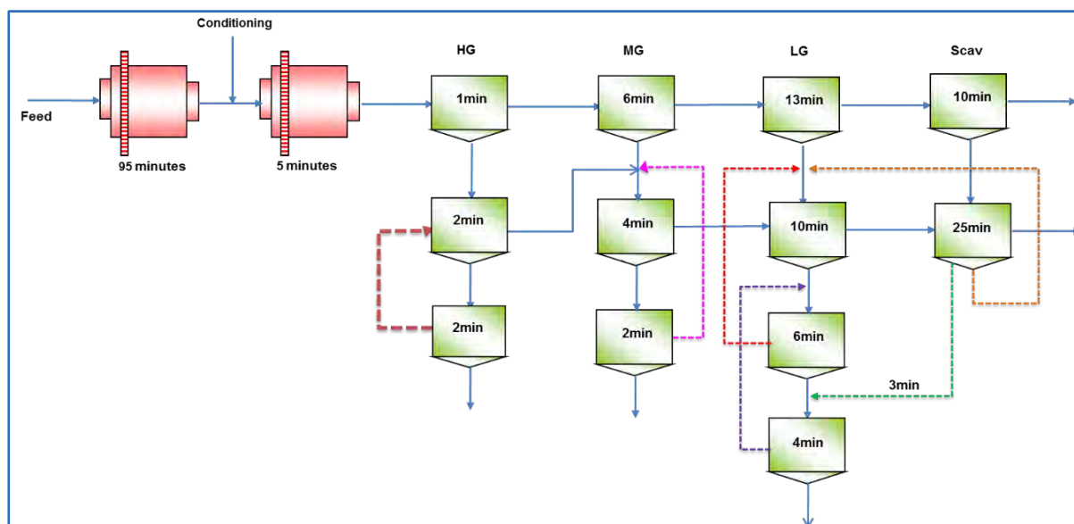
Figure 13.29 Optimised Platreef 2017 FS Locked Cycle Test Flow Sheet (Flow Sheet 3)
