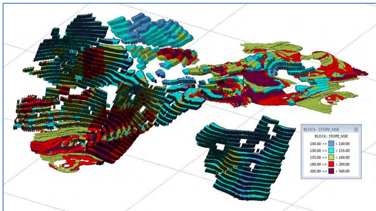
Figure 16.28 NSR Values by Stope
