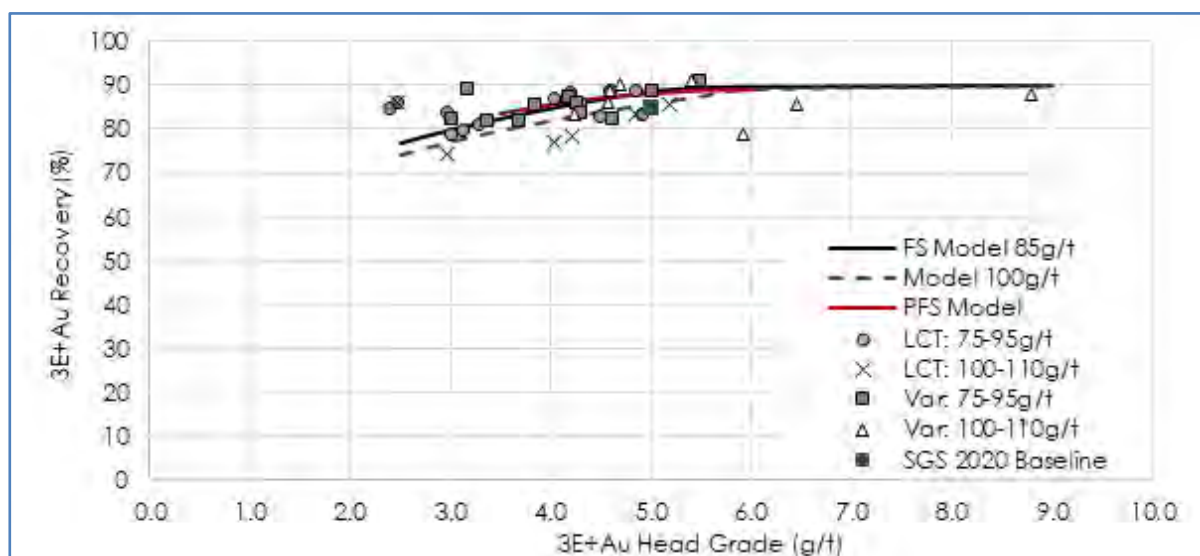
Figure 1.6 3PE+Au Recovery as a Function of Concentrate Grade
