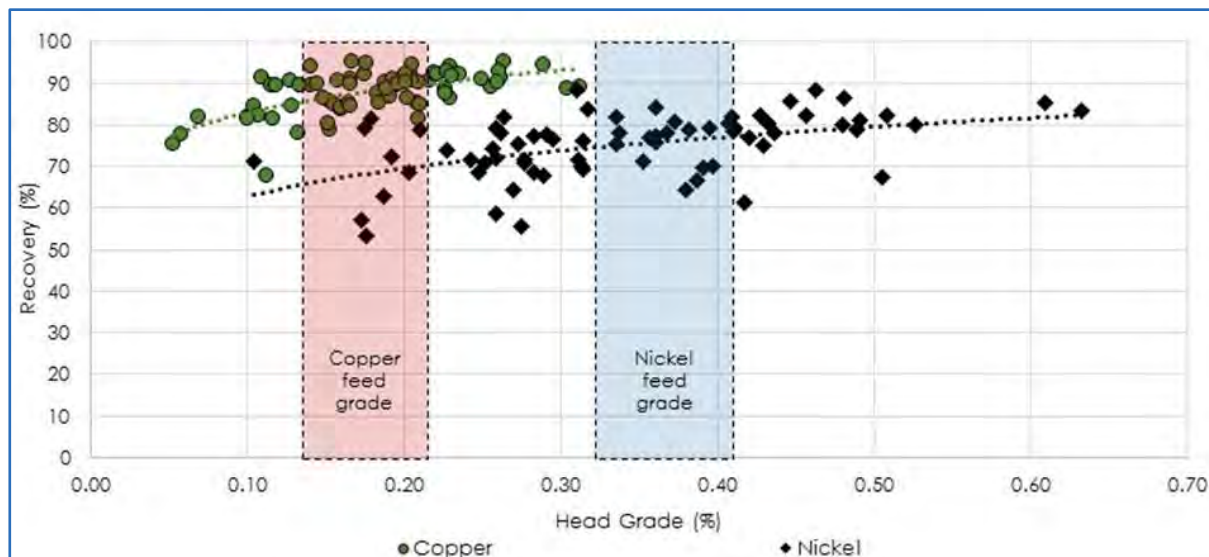
Figure 13.25 Variability Testwork Recovery as a Function of Head Grade
