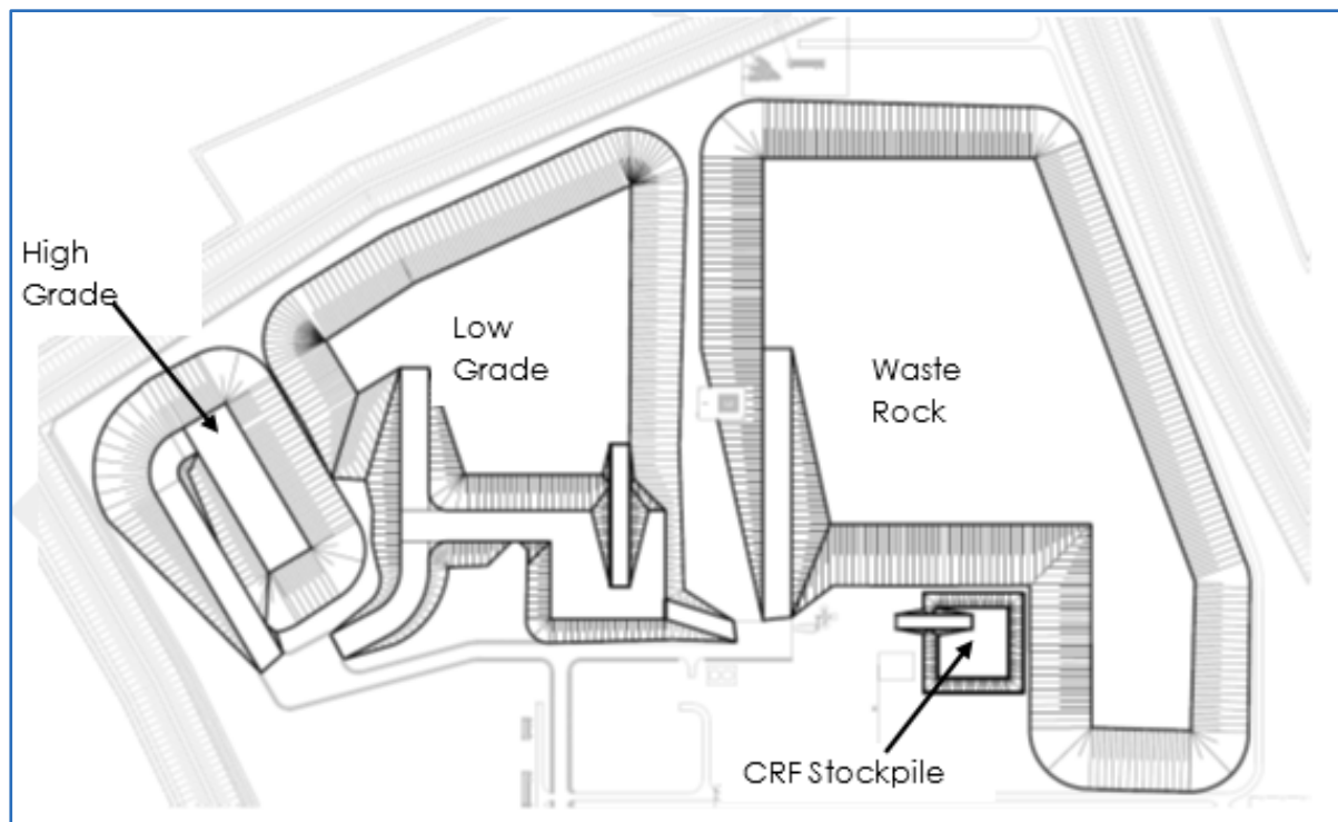
Figure 18.17 Material Storage Stockpiles
