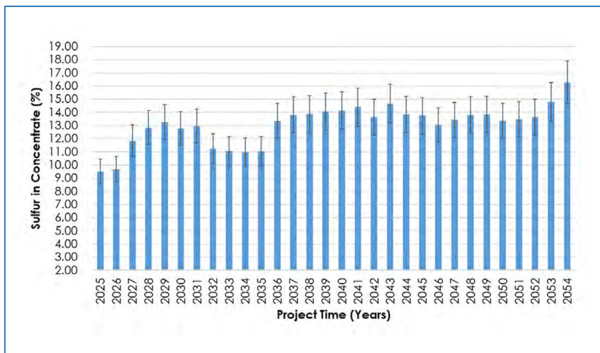
Figure 13.48 Modelled Life-of-Mine Sulfur in Concentrate
