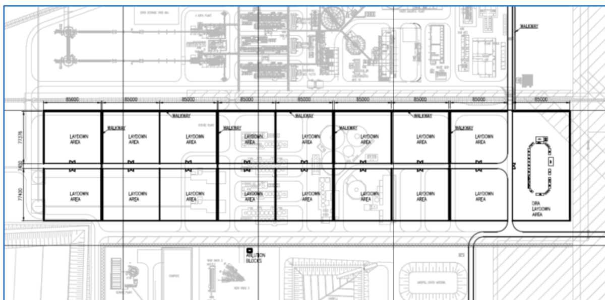
Figure 18.38 Construction Laydown Area
