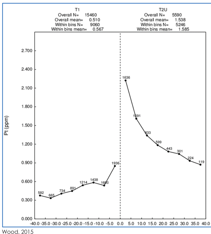
Figure 14.7 Contact Profile for Platinum Between T1 and T2U
