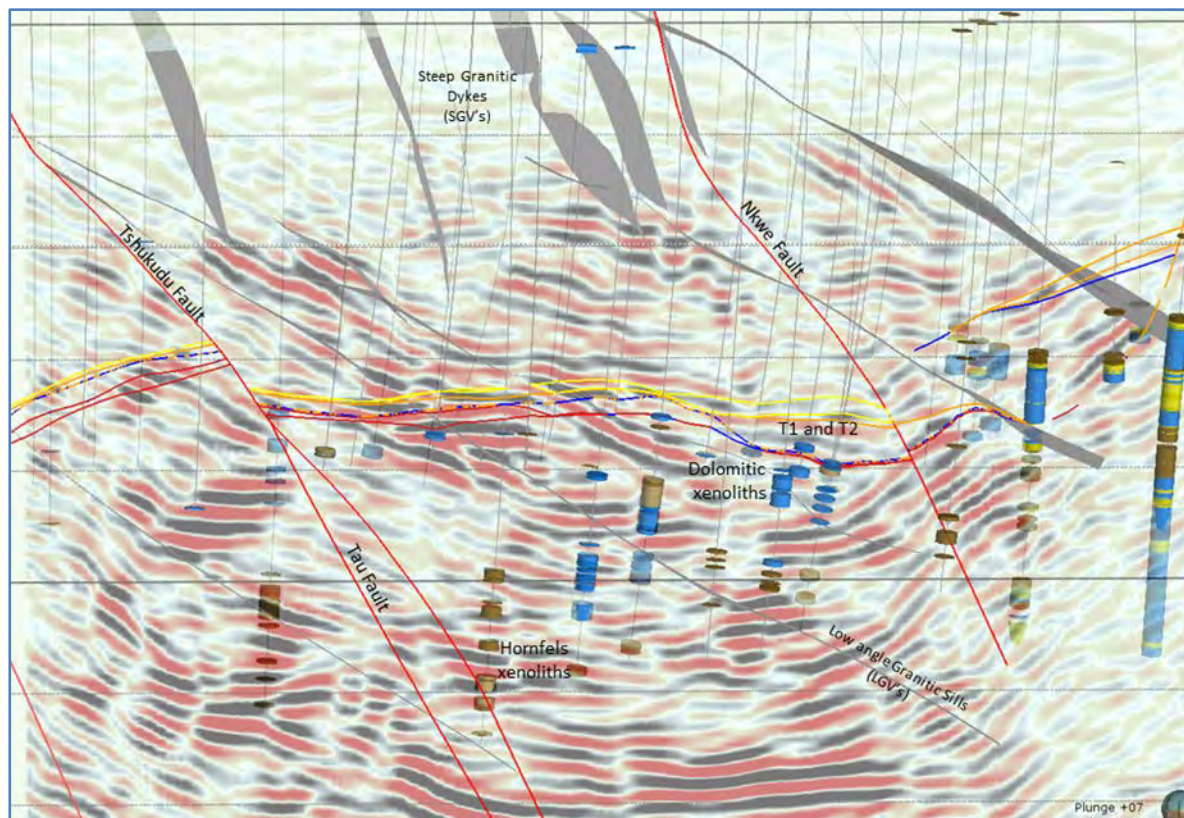
Figure 9.5 Dip Section 10.0 from Velsis Depth Converted Data
