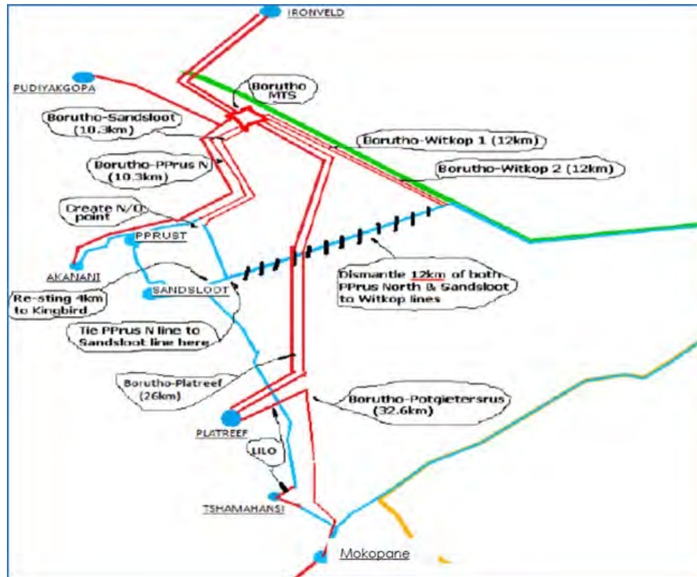
Figure 18.11 Eskom Supply Network
