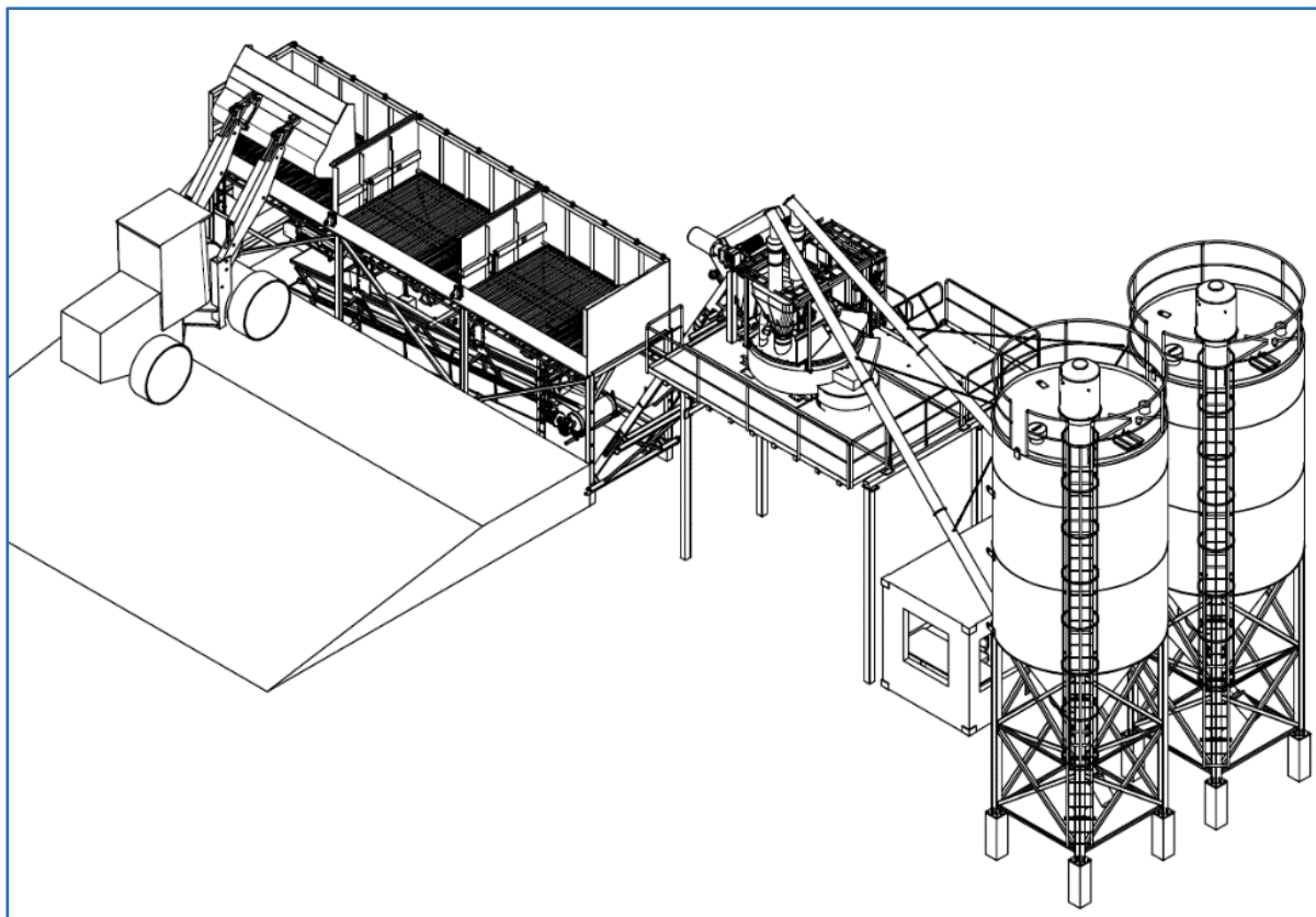
Figure 18.31 Surface Shotcrete and Concrete Batch Plant
