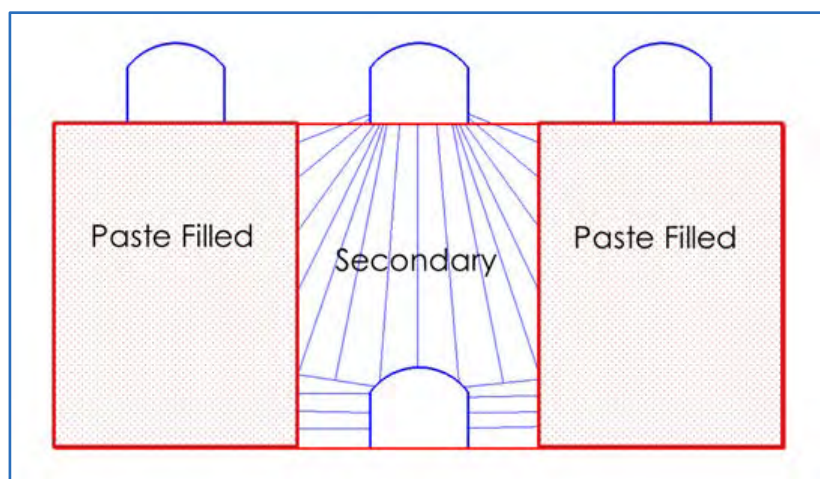
Figure 16.15 Typical Drill Pattern for Longhole Stopping
