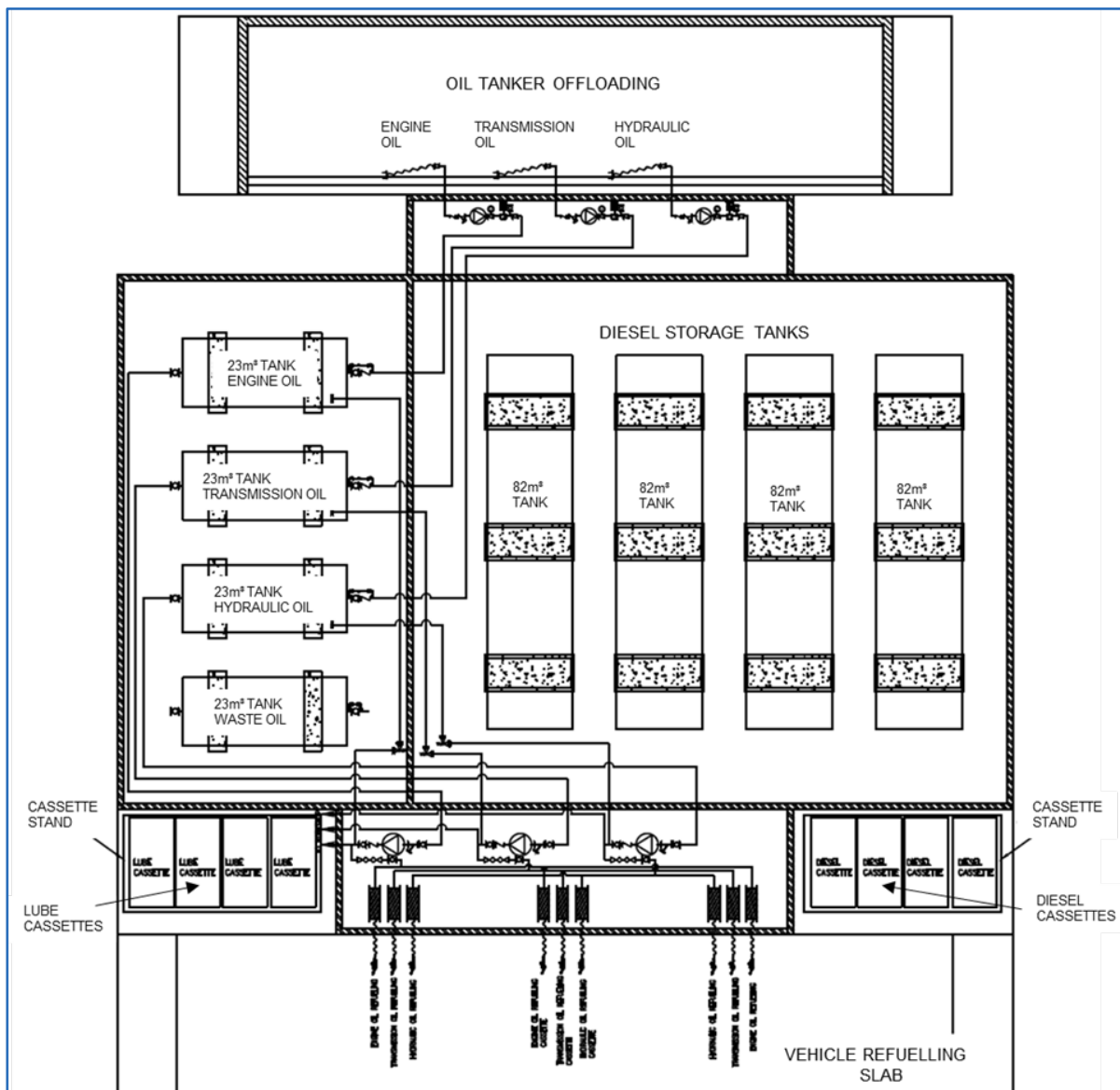
Figure 18.29 Surface Fuel and Lube Receiving, Storage and Dispensing Depot – Lubes Receiving and Dispensing
