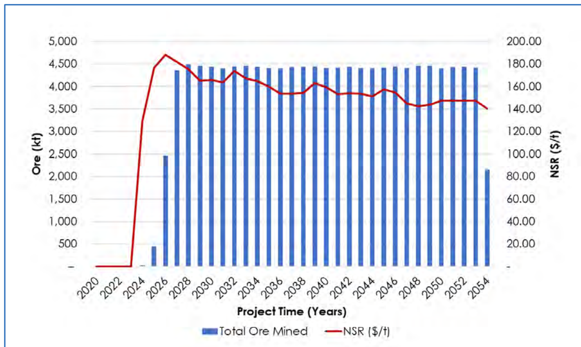
Figure 16.30 Annual Production with NSR
