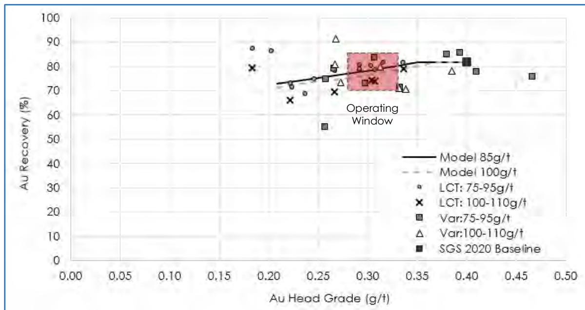
Figure 13.42 Gold Recovery as a Function of Feed Grade and Targeted Concentrate Grade
