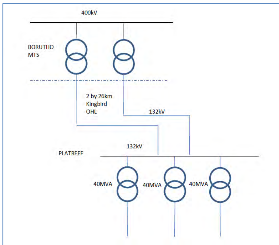
Figure 18.12 Bulk Power Scope of Work
