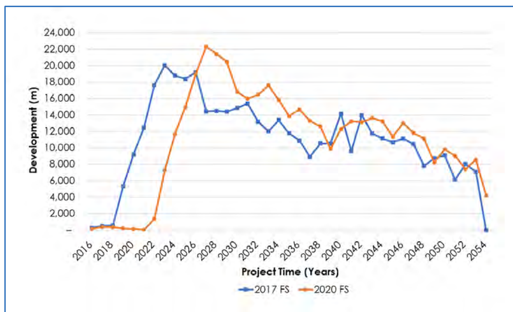
Figure 16.40 Total Development
