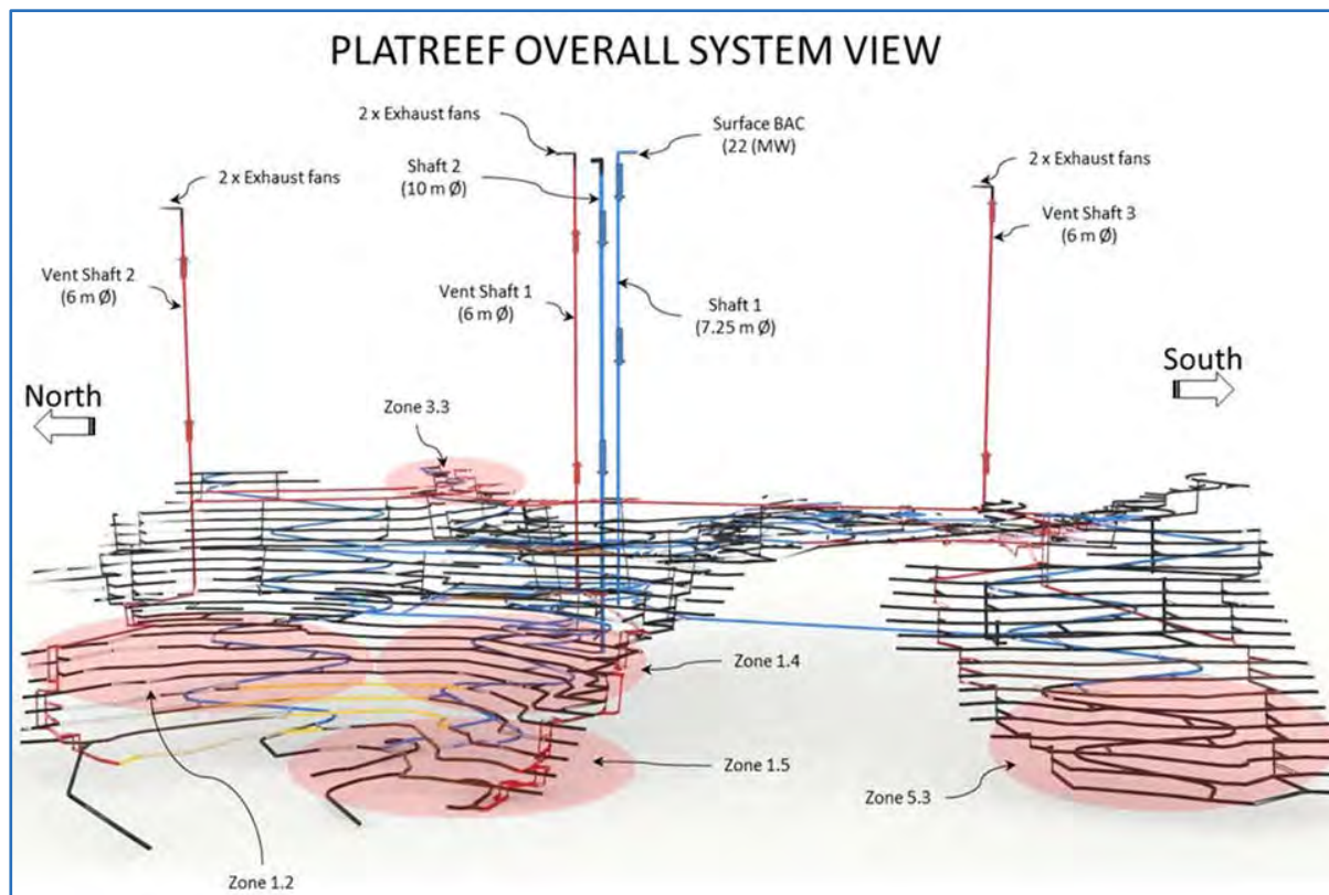
Figure 16.48 General Underground Mine Ventilation Arrangement
