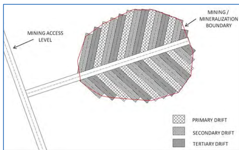
Figure 16.25 Typical Drift-and-Fill Level Layout
