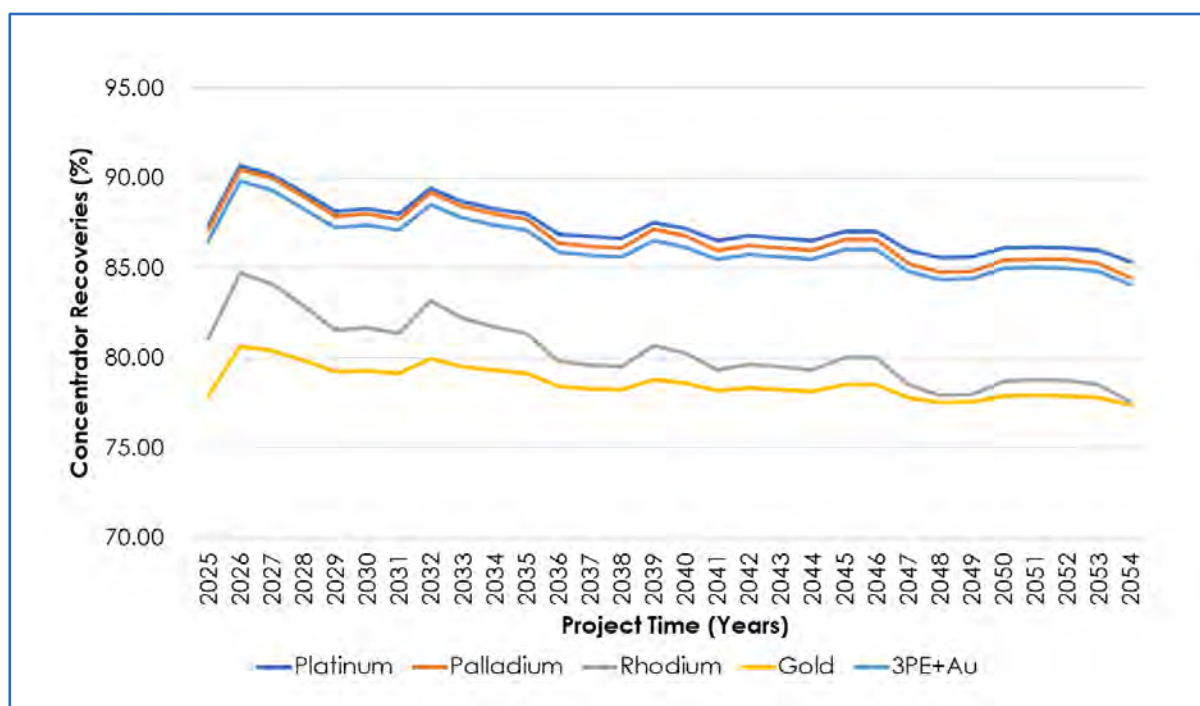
Figure 13.45 Modelled Steady State Life-of-Mine 3PE+Au Recovery Profile
