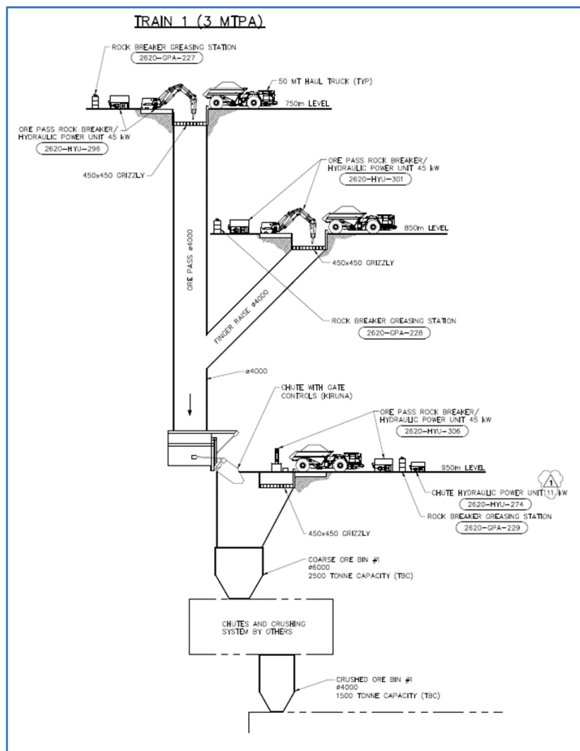
Figure 16.44 Main Ore Pass Arrangement and Truck Chutes
