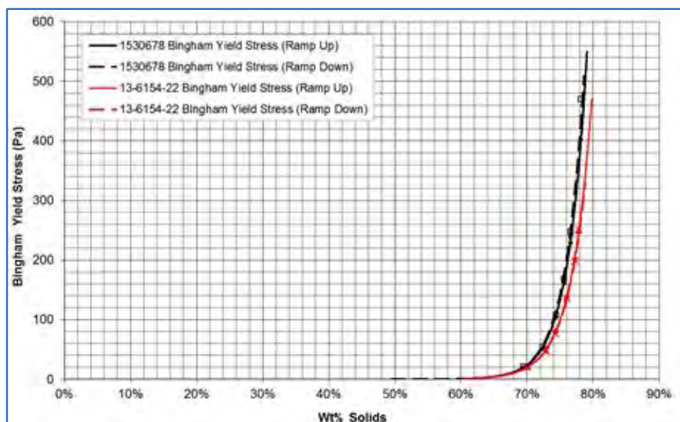
Figure 16.20 Bingham Viscosity Comparison
