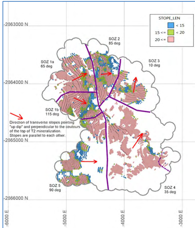
Figure 16.10 Longhole MSO Stopes – $130/T NSR Cut-off
