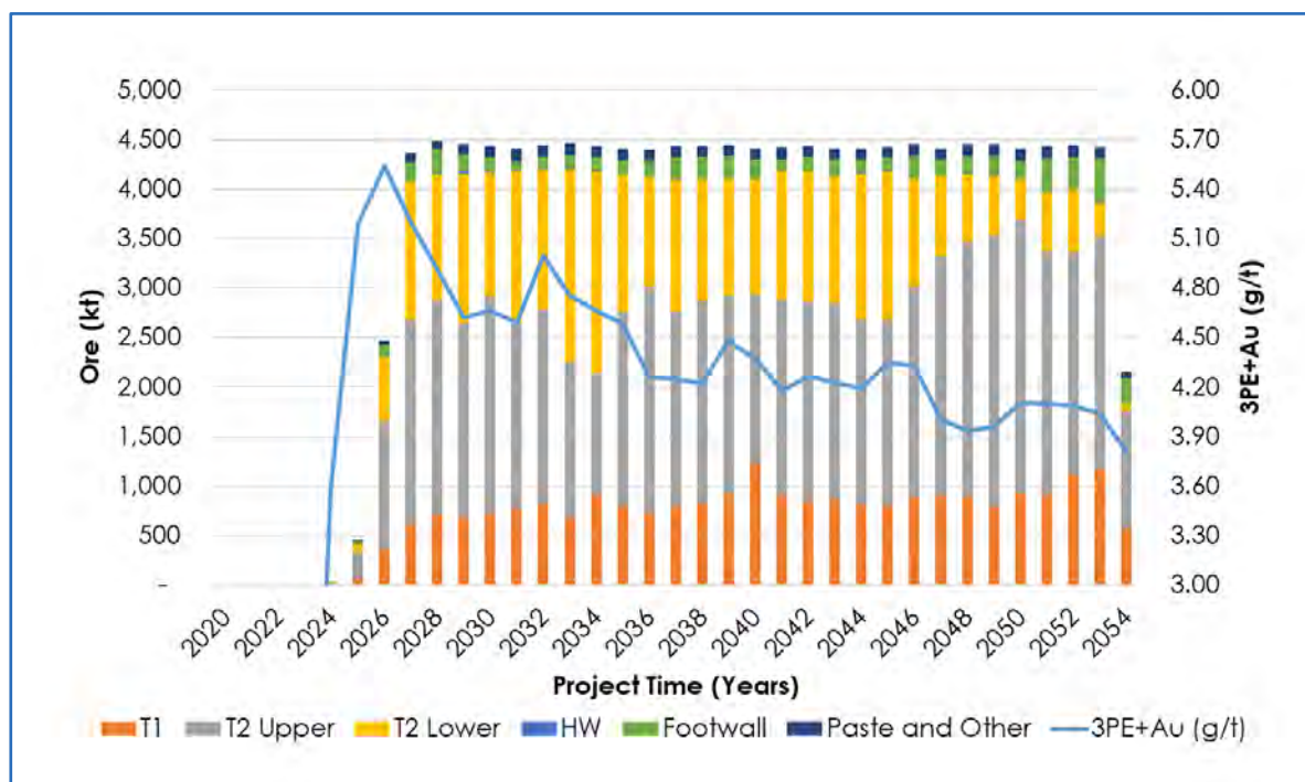
Figure 16.35 Annual Production by Rock Type with 3PE+Au
