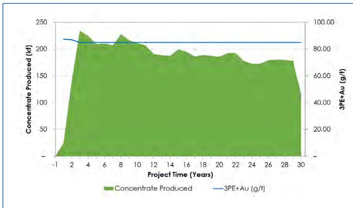
Figure 1.13 Platreef 2020 FS Estimated Concentrate Produced and 3PE+Au Grade
