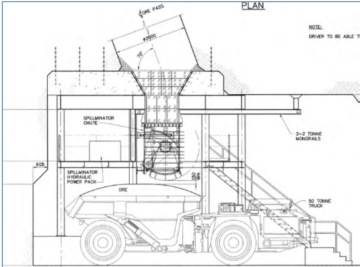
Figure 16.43 Typical Truck Loading Arrangement
