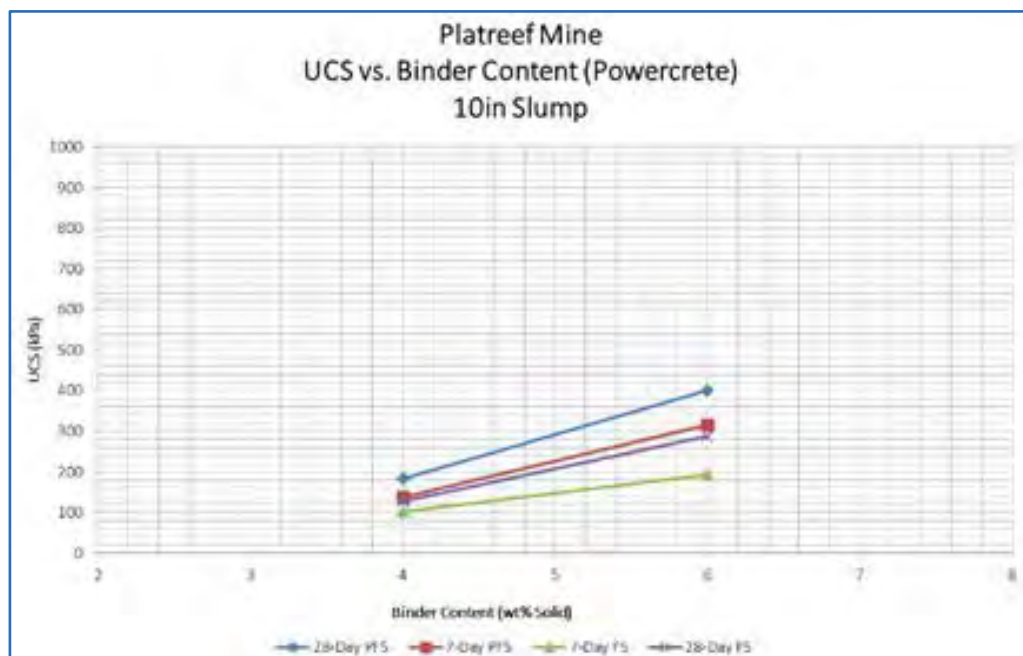
Figure 16.22 UCS vs. Binder Content – 10" (254 mm) Slump
