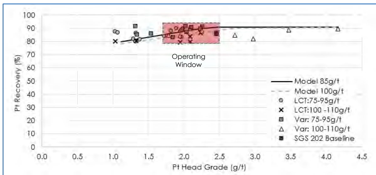
Figure 13.39 Platinum Recovery as a Function of Feed Grade and Targeted Concentrate Grade
