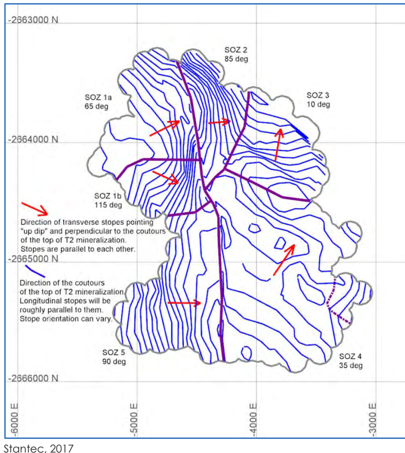
Figure 16.9 Longhole Stope Orientation Zones
