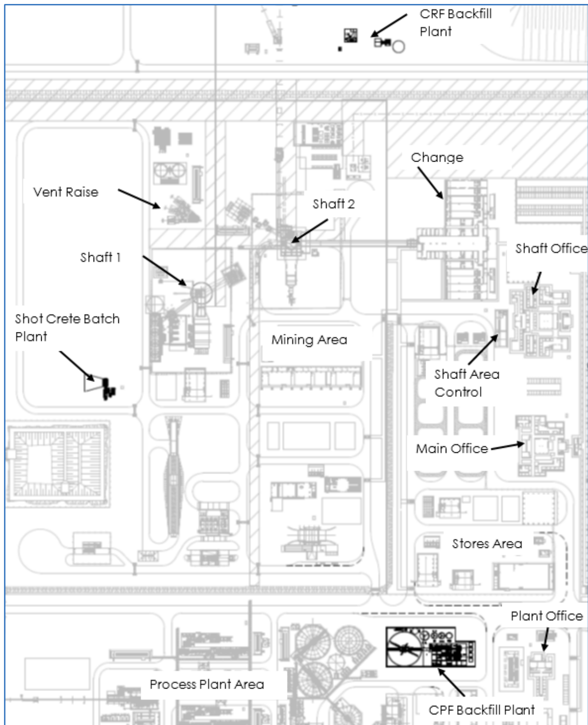
Figure 18.33 Shaft Area Services with Backfill Plants
