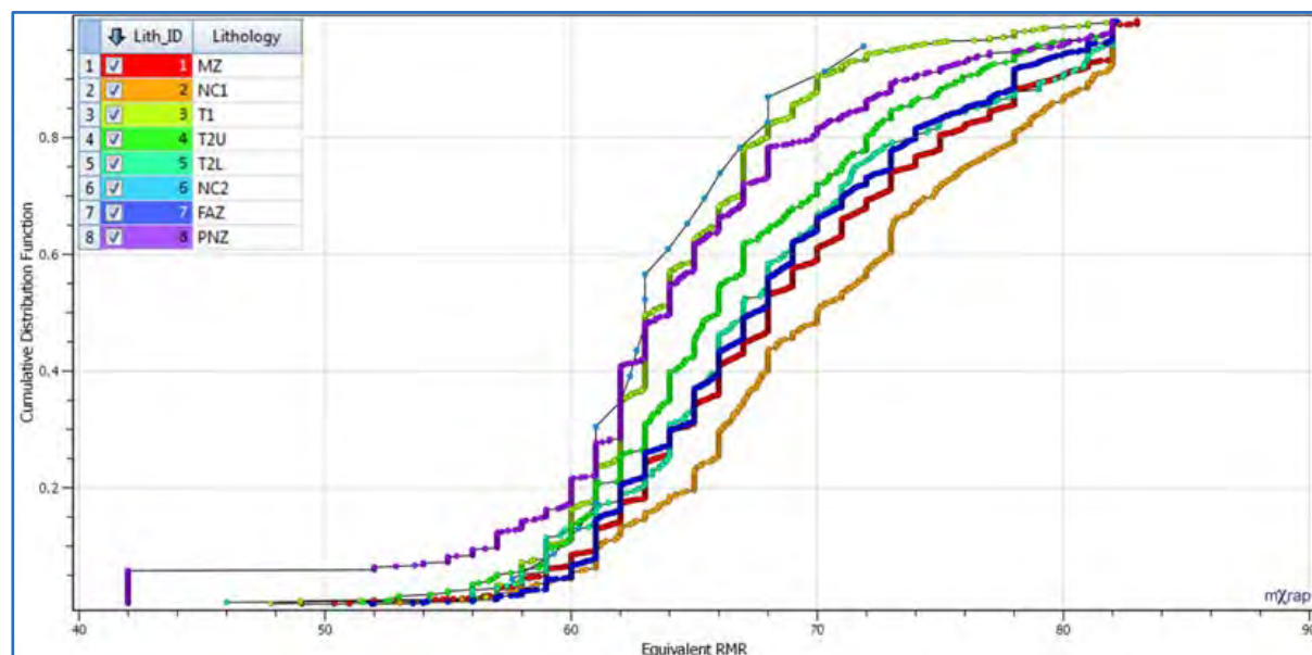
Figure 16.2 Cumulative Distribution Curve of RMR Values (Converted From Q') for All Stratigraphic Units
