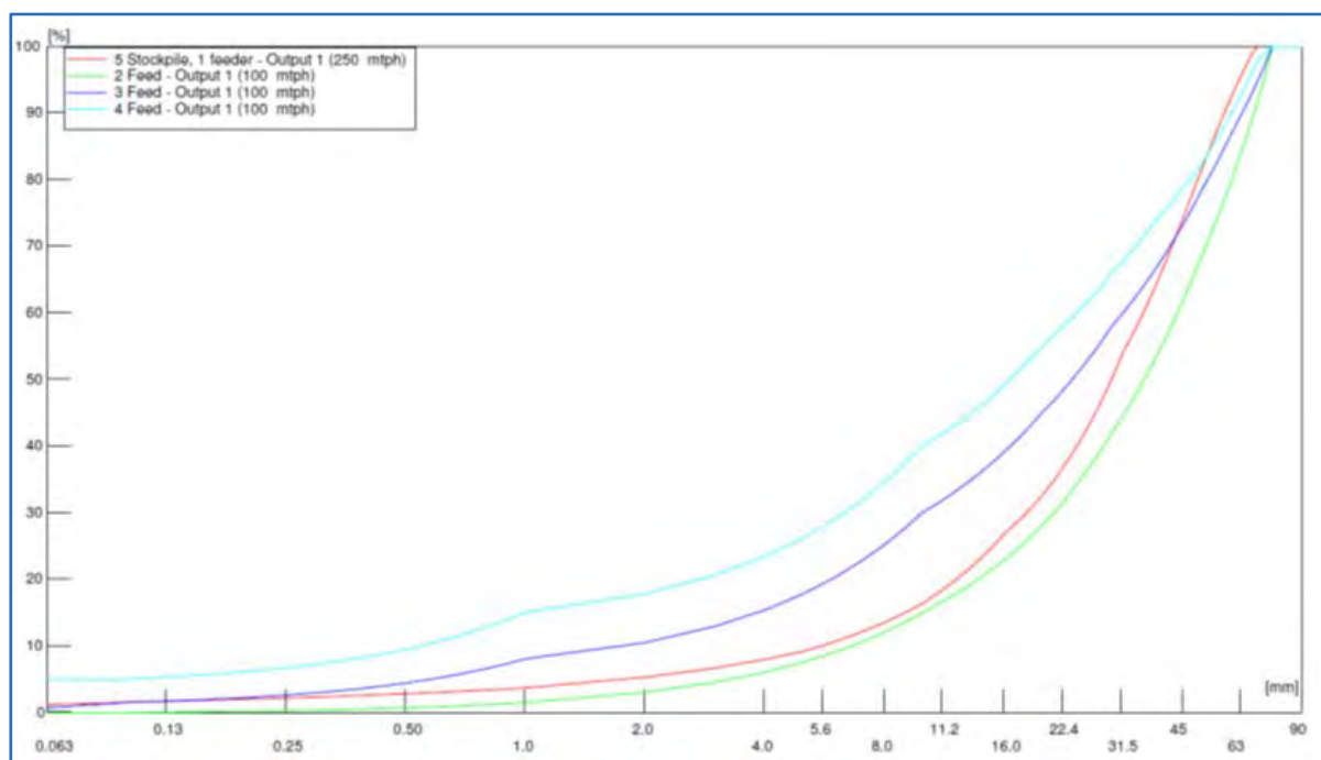
Figure 18.23 Grading Analysis of Waste Rock Material
