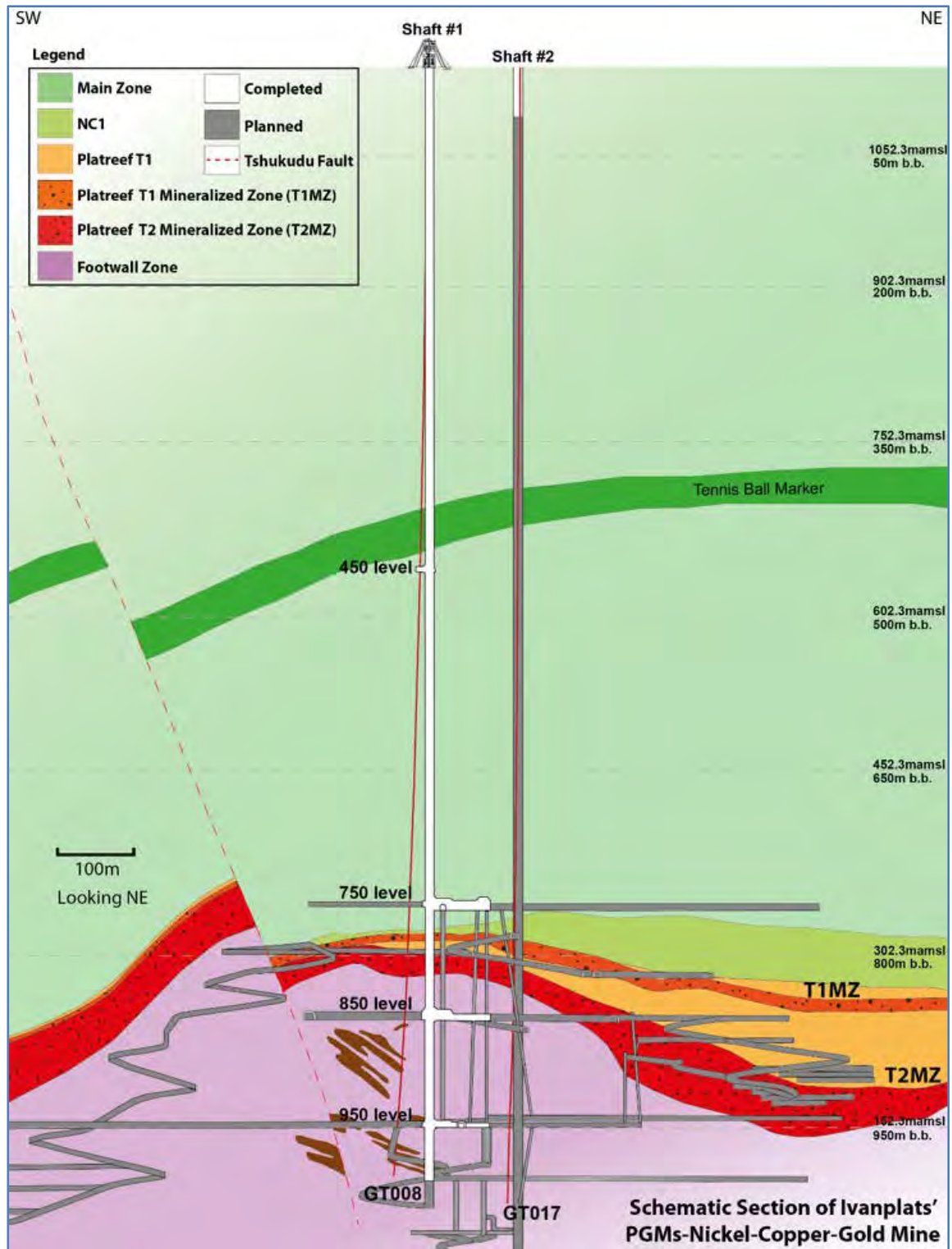
Figure 16.17 Schematic Section of the Platreef Mine
