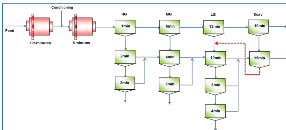
Figure 13.28 Development Testing Locked Cycle Test Flow Sheet 2 (Flow Sheet 2)
