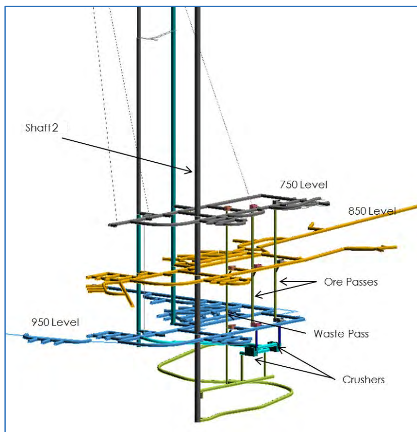
Figure 16.41 Ore Handling System (Isometric View)
