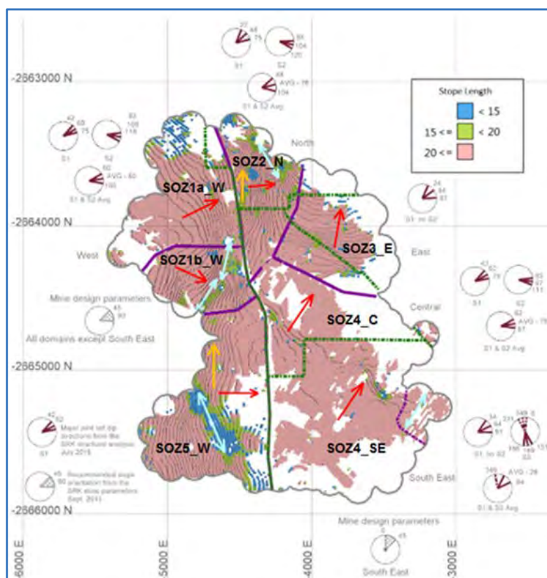
Figure 16.1 Proposed Stope Orientations by Stantec
