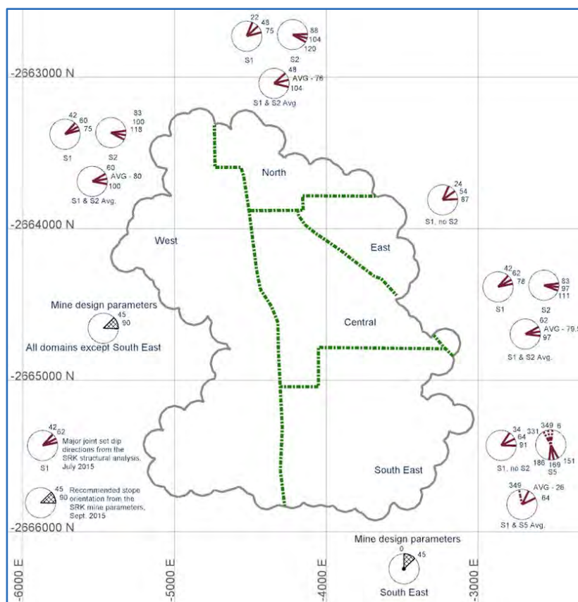
Figure 16.12 SRK Structural Domains and Preferred Stope Orientations
