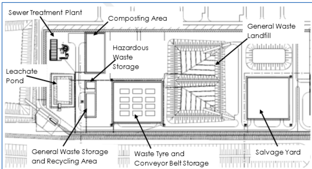
Figure 18.37 Waste Facilities Area
