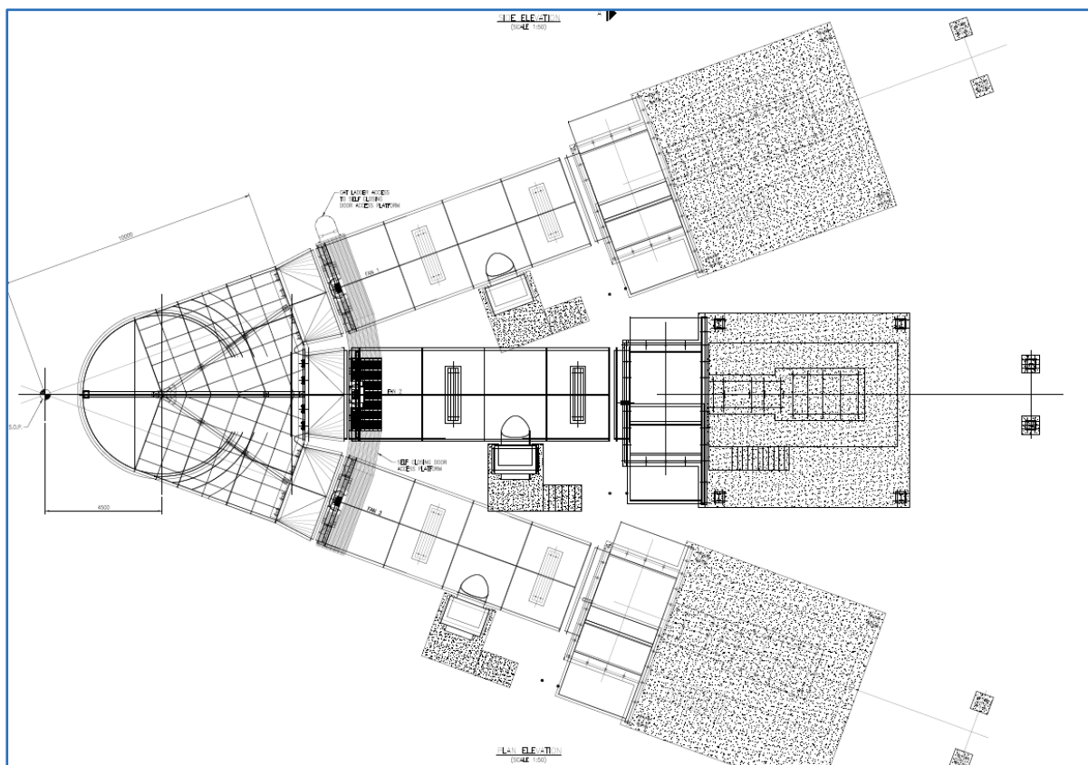
Figure 18.32 Main Ventilation Fans Layout
