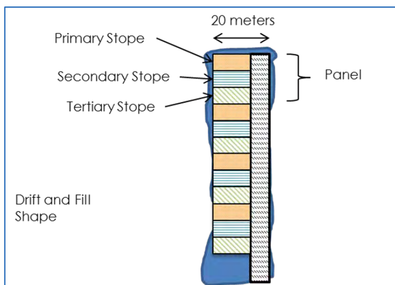
Figure 16.24 Typical Drift-and-Fill Transverse Layout
