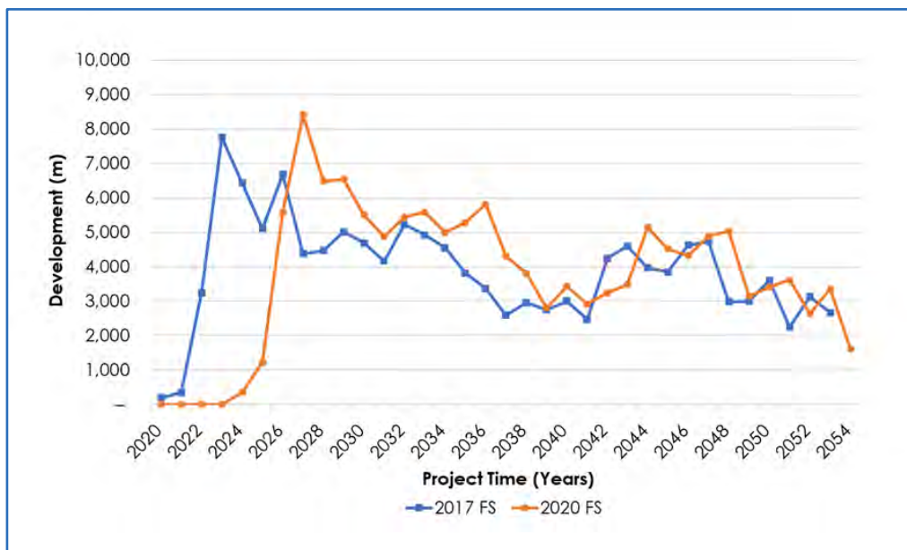
Figure 16.39 Ore Development
