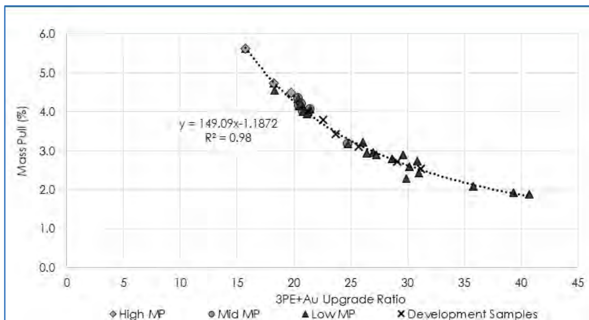
Figure 13.33 Locked Cycle Test Mass Pull as a Function of PGE Upgrade Ratio
