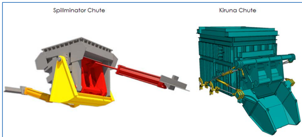
Figure 16.45 Chute Comparison
