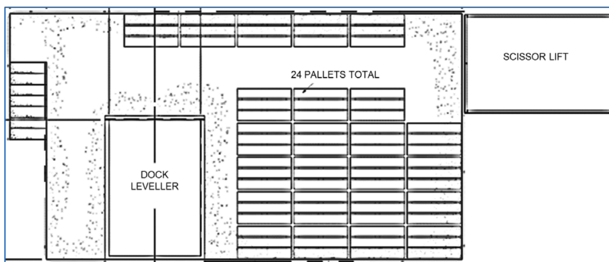
Figure 18.26 Explosives Offloading Facility – Plan View
