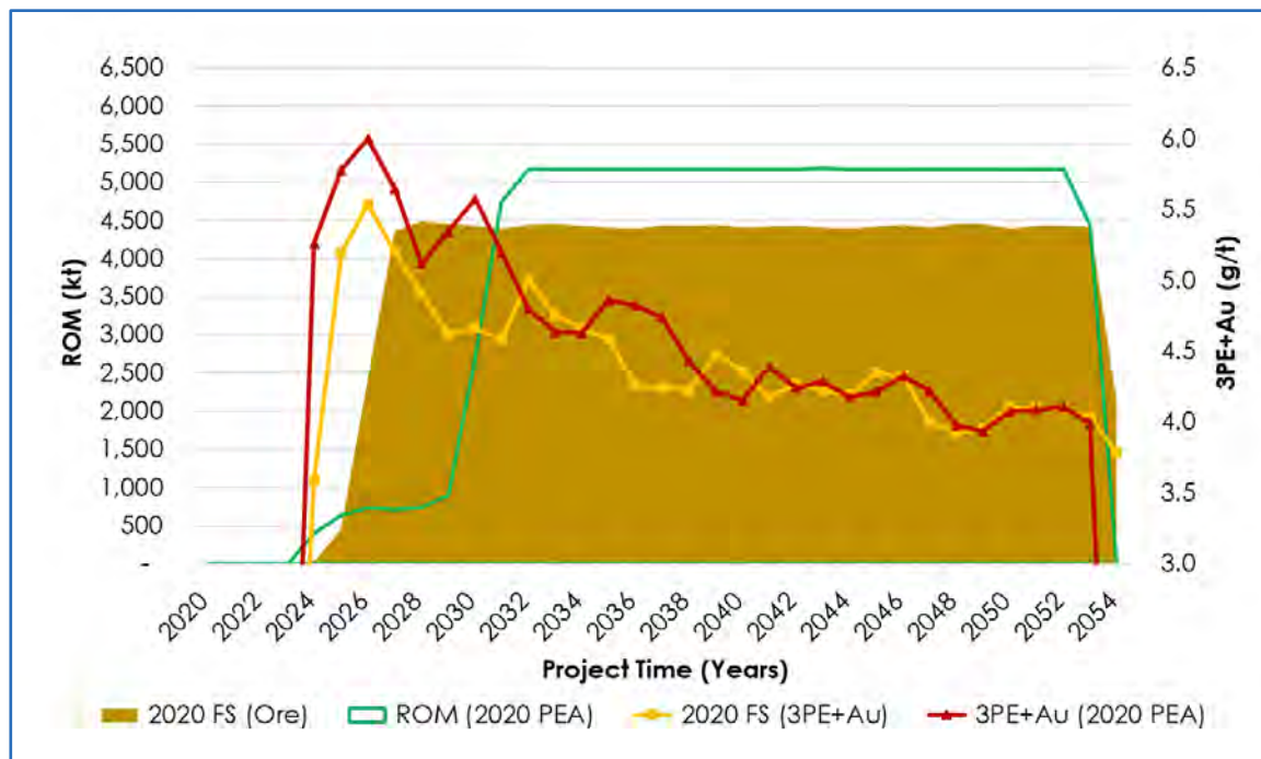
Figure 24.3 Platreef 2020 PEA Run-of-Mine Production
