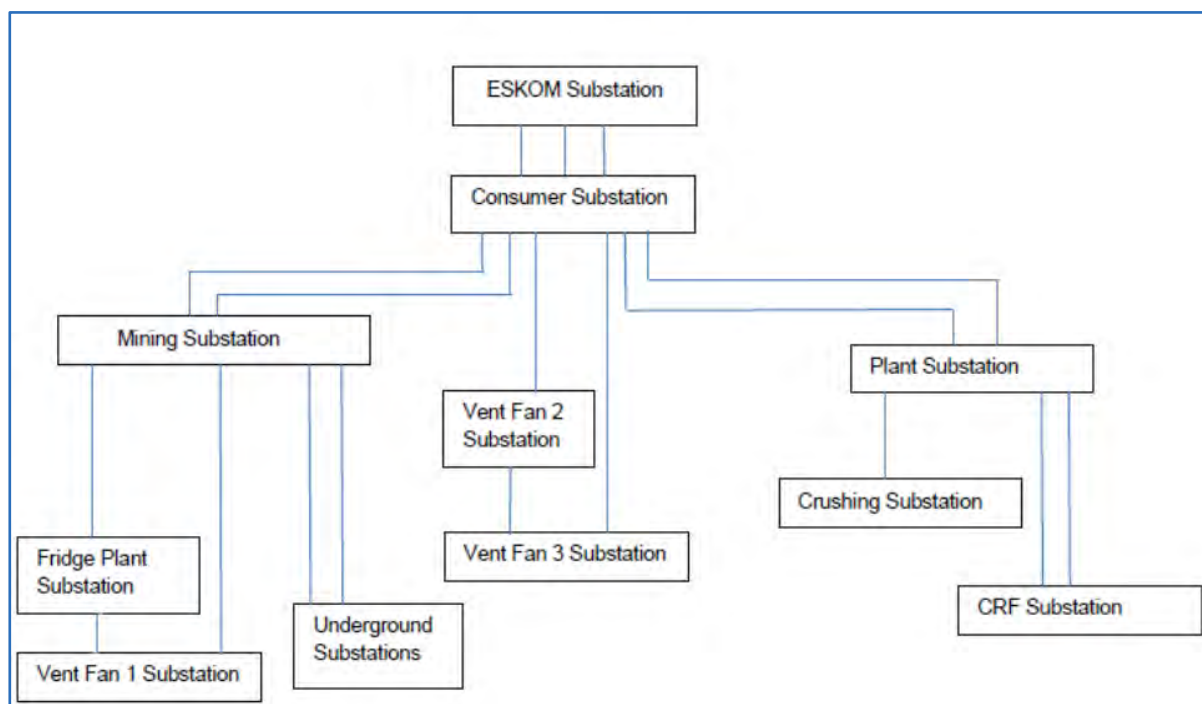
Figure 18.21 MV Distribution
