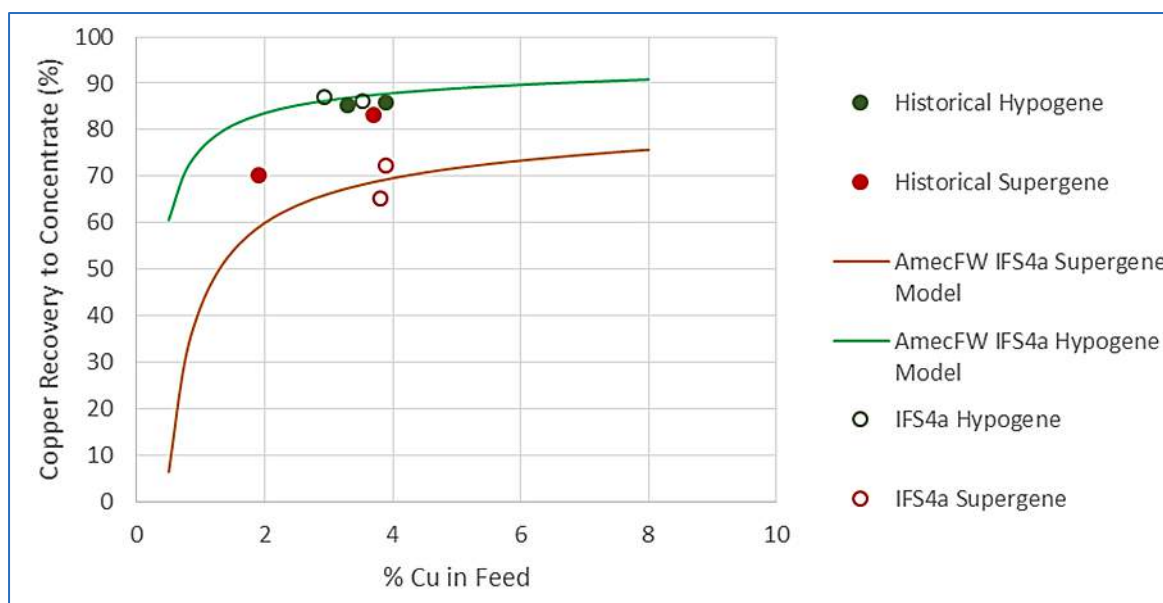
Figure 13.14 Updated Recovery Models based on PFS Testing
