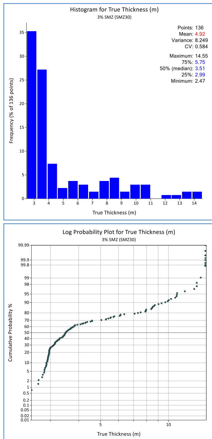
Figure 14.16 Kakula: Full Width SMZ Composite True Thickness (m) for 3.0% TCu Grade Shell (SMZ30). Histogram and Probability Plot
