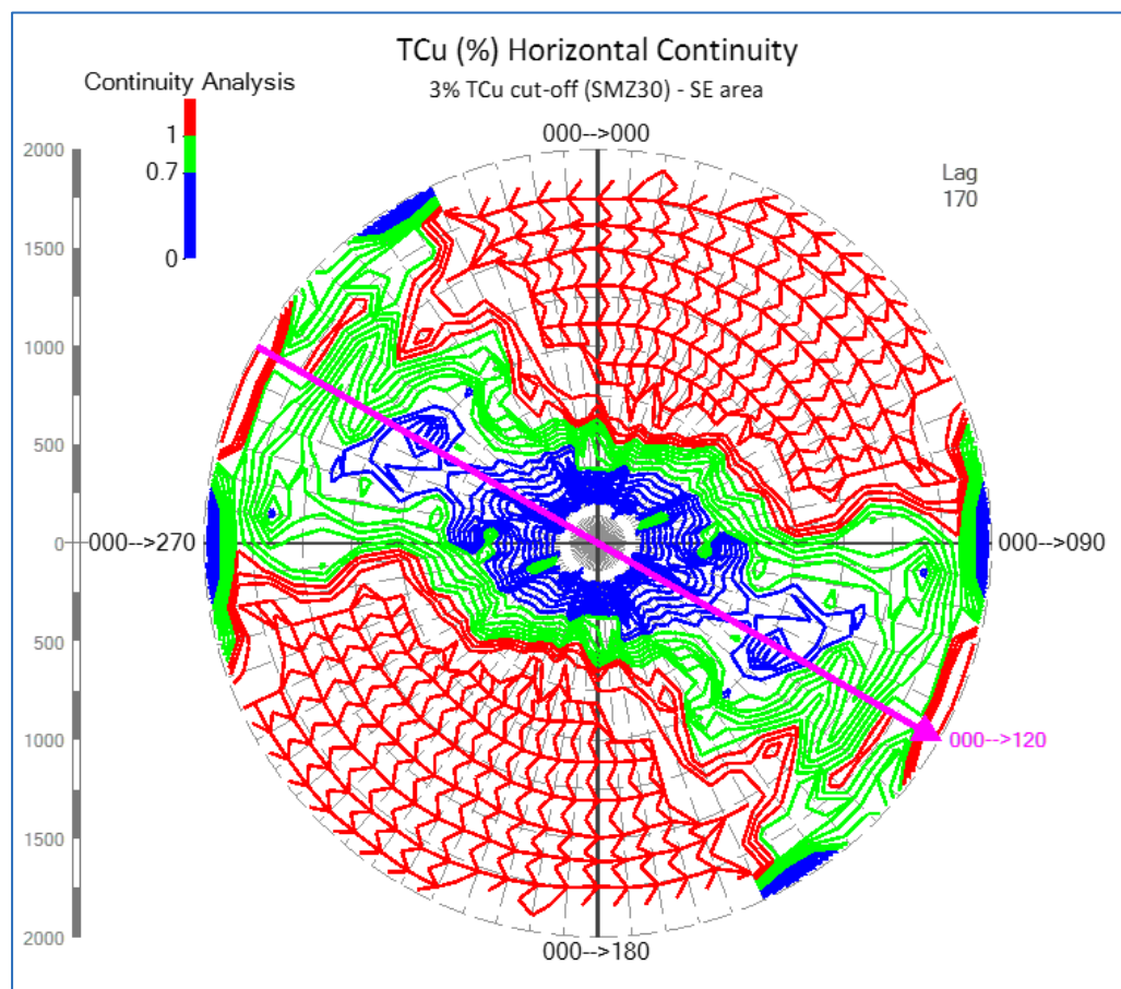
Figure 7.42 Variogram Fan for the Normal Score Variogram of TCu (%) Within the 3% Grade Shell at Kakula
