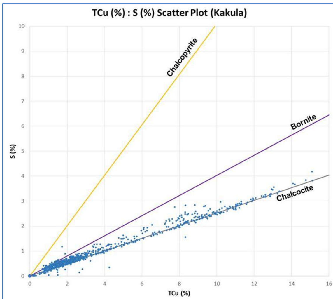
Figure 7.35 Scatter Plot Illustrating Clear Sulphide Species Within the 3% Grade Shell (SMZ30) at Kakula. Theoretical TCu: S Ratios for Chalcopyrite (orange), Bornite (purple) and Chalcocite (grey) Based Upon Molar Mass Ratios
