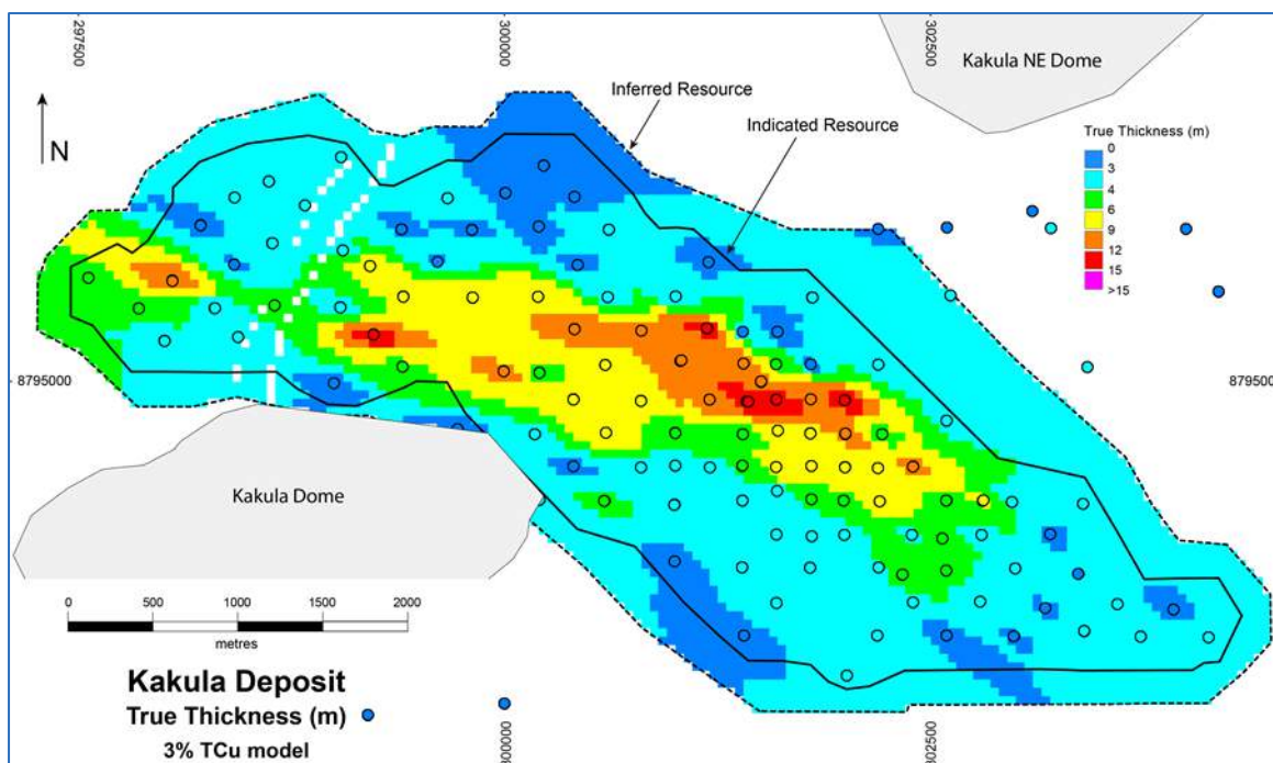
Figure 14.26 Kakula: Estimated True Thickness (m) for the 3.0% TCu Grade Shell (SMZ30)
