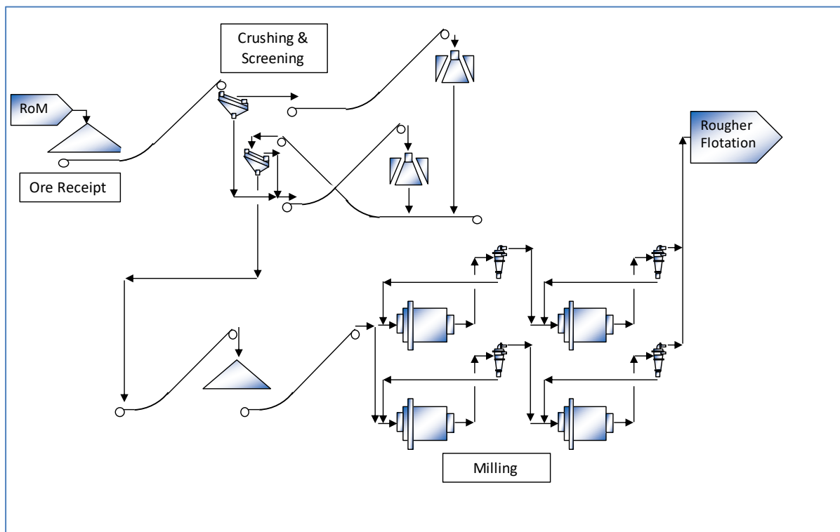
Figure 24.33 Kakula Crushing and Milling
