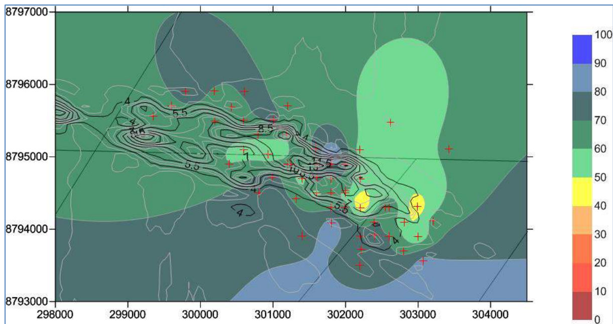
Figure 16.9 RMR B89 Contour Map for the Hanging (based on IRS from field estimates)
