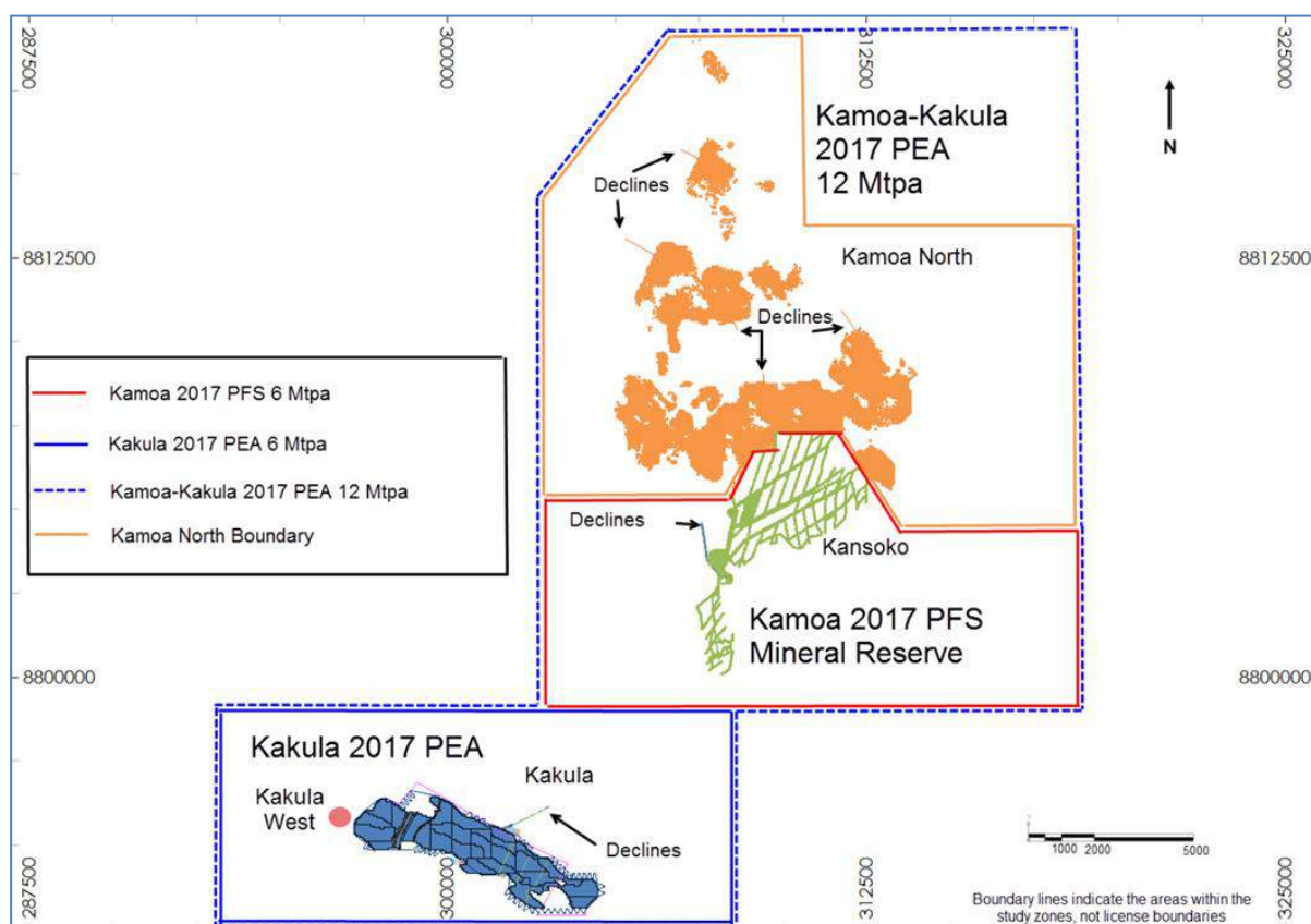
Figure 1.1 Kamoa 2017 PFS and Kamoa-Kakula 2017 PEA Mining Locations
