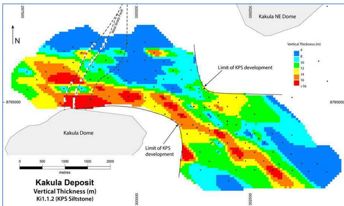
Figure 7.19 Vertical Thickness of the Ki1.1.2 (KPS) at the Kakula Deposit
