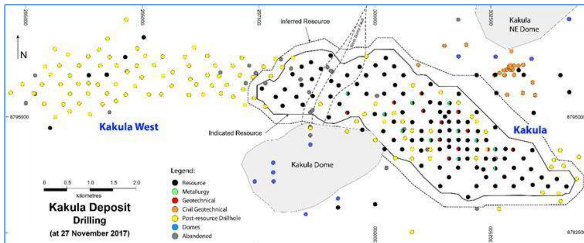
Figure 10.2 Drill Location Plan, Kakula
