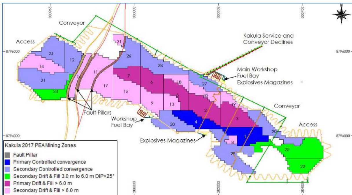
Figure 1.17 Kakula 2017 PEA Development and Mining Zones
