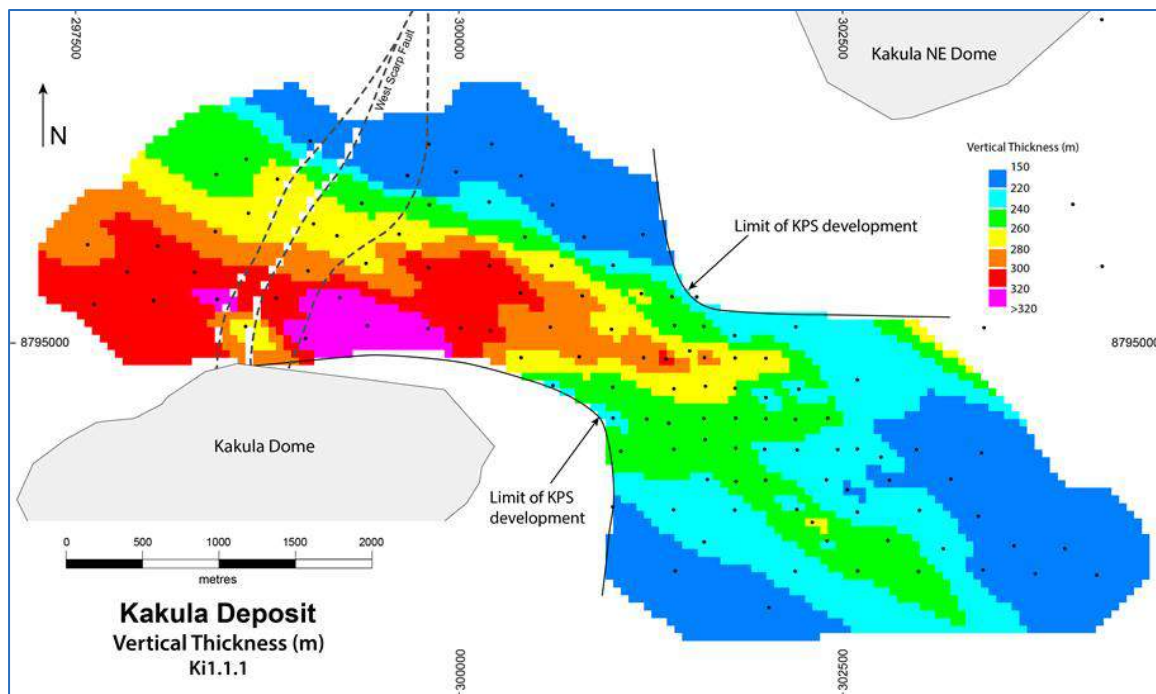
Figure 7.18 Vertical Thickness of the Ki1.1.1 at the Kakula Deposit
