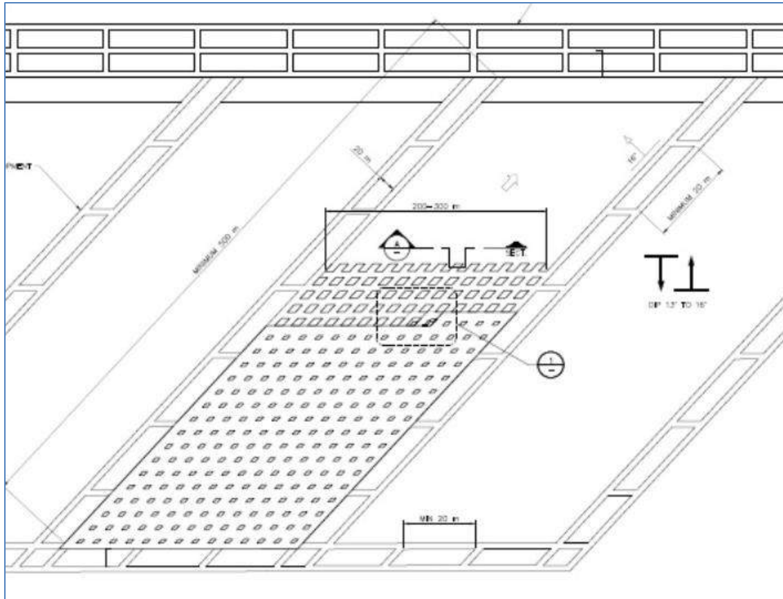
Figure 16.12 Typical Controlled Convergence Room-and-Pillar Mining Panel
