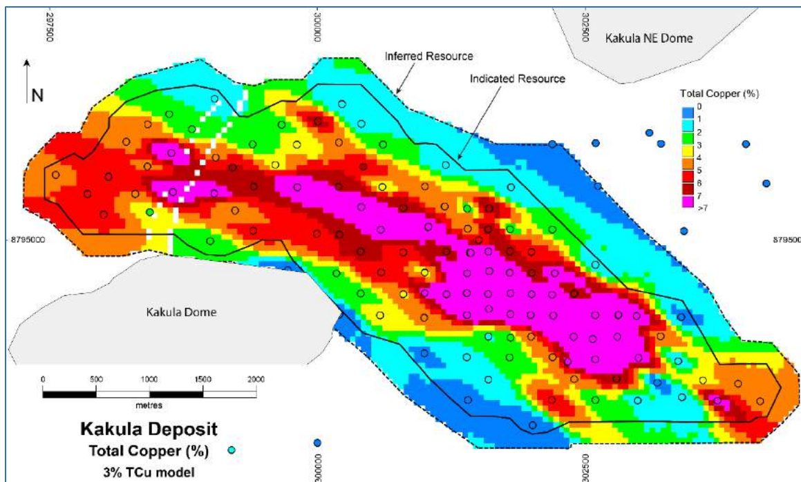
Figure 14.25 Kakula: Estimated TCu (%) for the 3.0% TCu Grade Shell (SMZ30)
