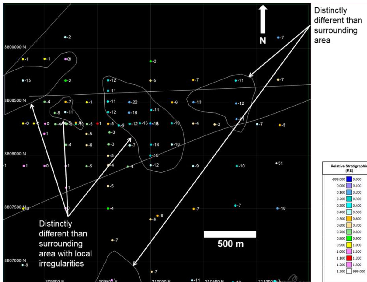
Figure 7.45 Stratigraphic Position of SMZ10 with Respect to the Base of the KPS
