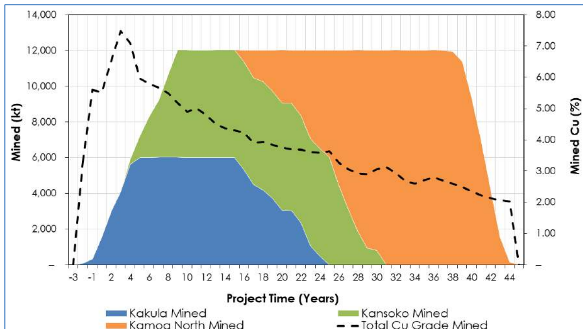
Figure 24.21 Kamoā-Kakula 12 Mtpa PEA Mine Production
