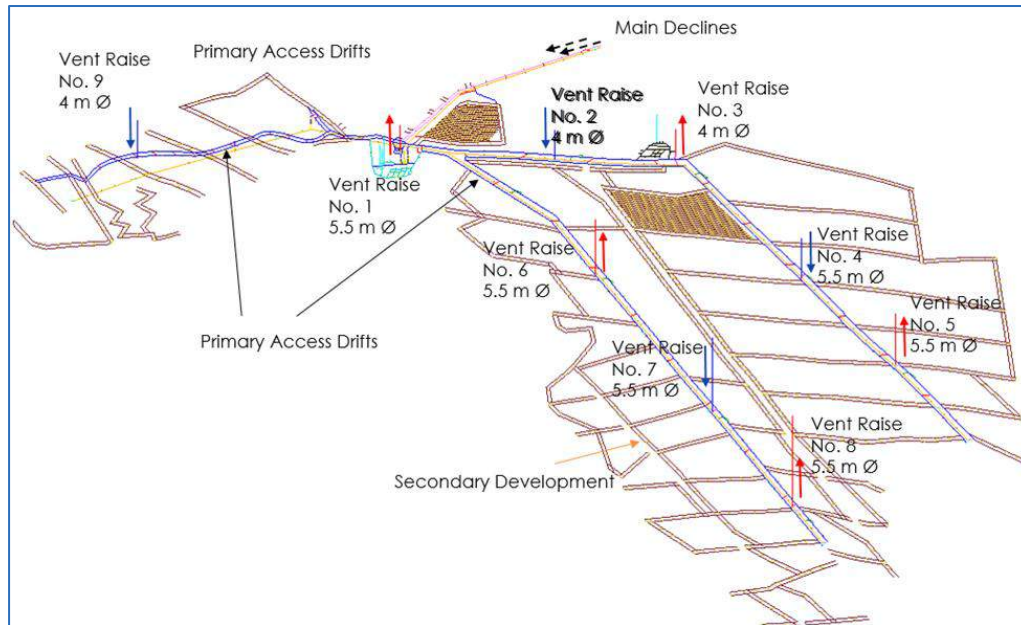
Figure 1.3 Mine Access and Ventilation
