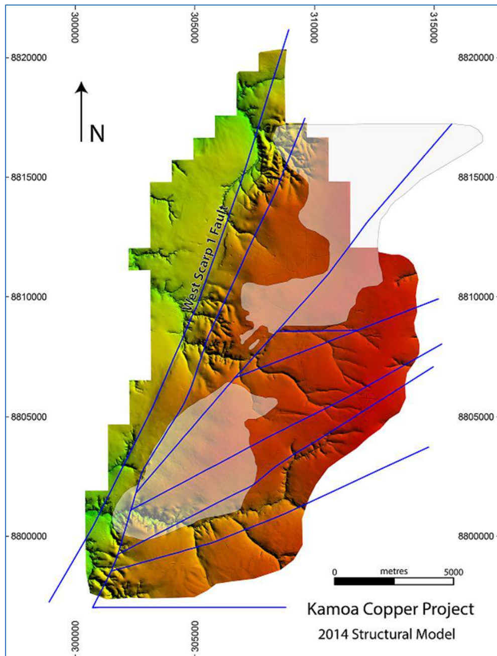
Figure 7.22 Structural Influences on Topography
