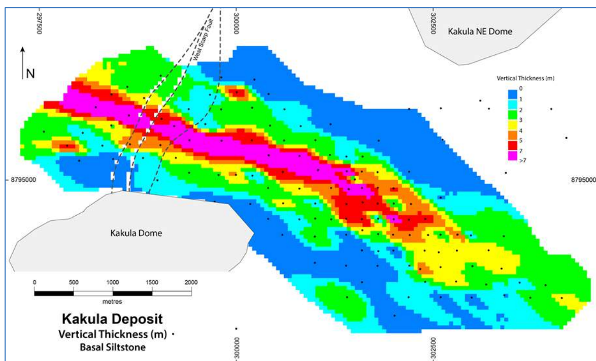
Figure 7.17 Vertical Thickness of the Basal Siltstone within the Ki1.1.1 at the Kakula Deposit
