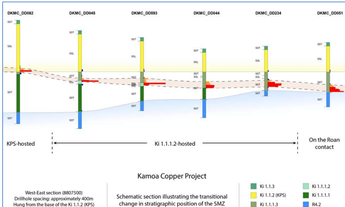
Figure 7.36 Stratigraphic Section Showing Continuity of Mineralisation Near Base of Ki 1.1.1.3 at the Kamoa Deposit
