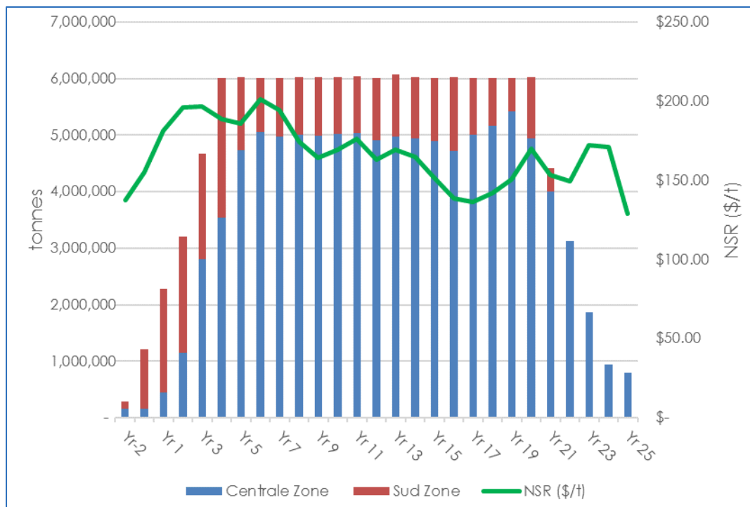
Figure 16.29 LOM Schedule and Grades
