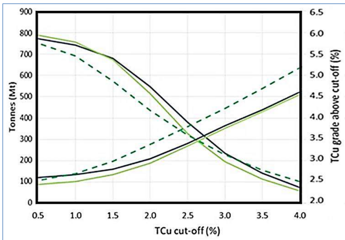
Figure 14.27 Comparative Grade-Tonnage Curves for the Kamoā 2D and 3D Models Constrained Within the Upper SMZ (Domains 110, 300, and 310) and Wireframe Defining the 1.0% TCu 2D Model (SMZ10)
