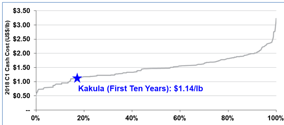
Figure 1.11 2018 C1 Copper Cash Costs
