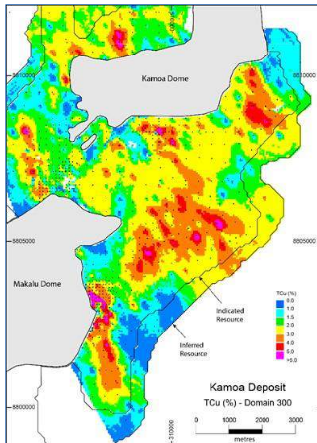
Figure 7.44 2017 Mineral Resource Model for TCu Grade
