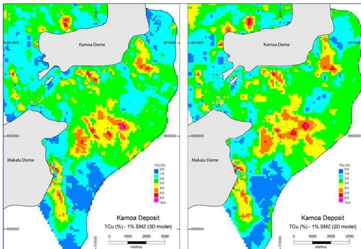
Figure 14.28 Comparison of 3D (left) and 2D (right) Models for Estimated TCu Grade (%) for a 1.0% TCU Modelling Cut-off (SMZ10)
