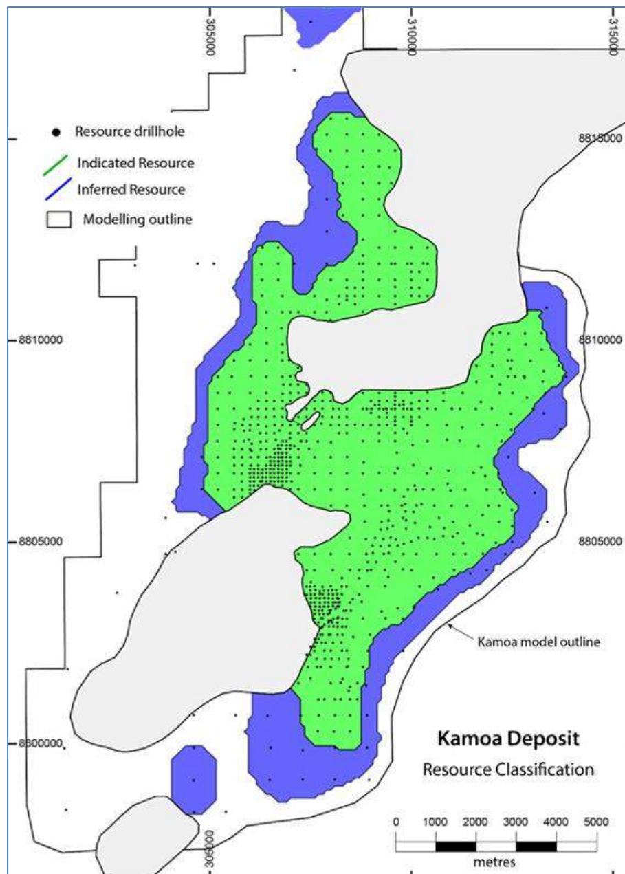
Figure 14.22 Kamoā: Mineral Resource Classification
