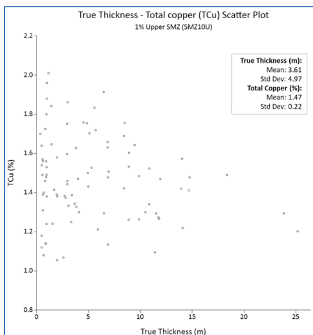
Figure 14.18 Kakula: Scatter Plot of TCu (%) Versus True Thickness (m) for the 1% Upper Grade Shell (SMZ10U)
