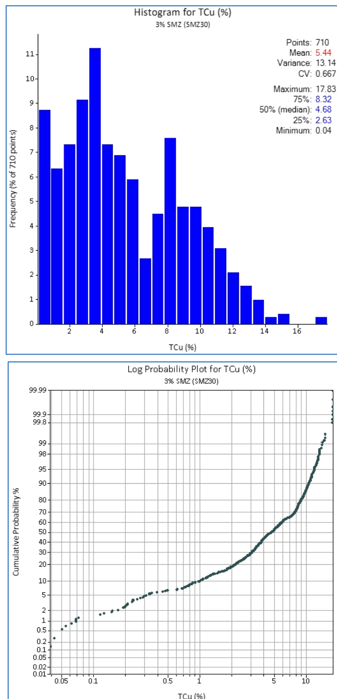
Figure 14.15 Kakula: 1 m Composite TCu (%) for 3.0% TCu Grade Shell (SMZ30). Histogram and Probability Plot
