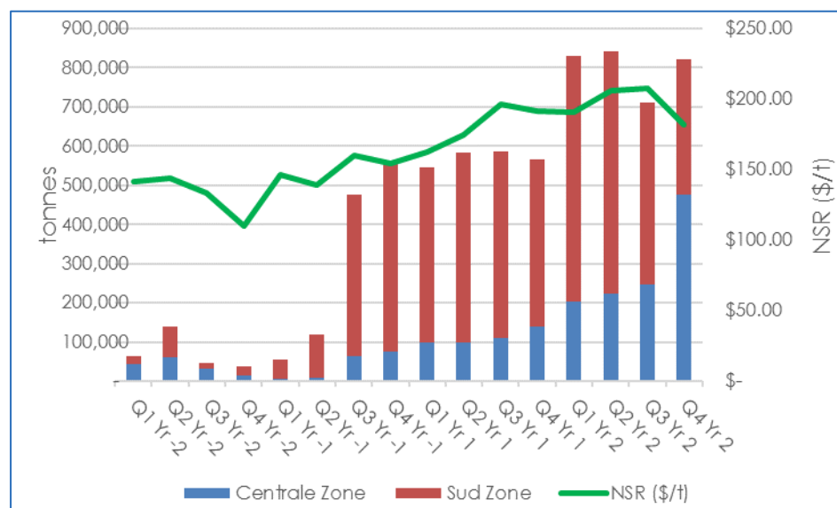
Figure 16.28 Pre-production Ramp-Up and Grades
