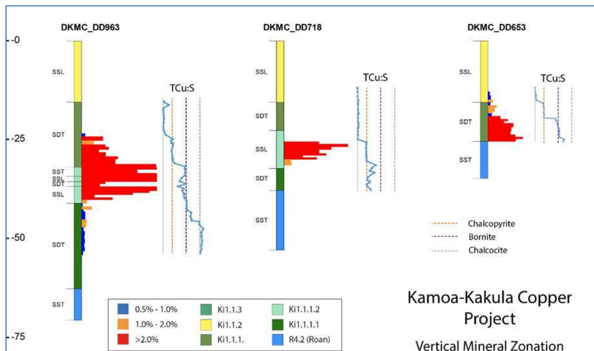
Figure 7.33 Examples from Three Drillholes from Kamoā of Vertical Mineral Zonation Evident Based on TCu: S Ratios
