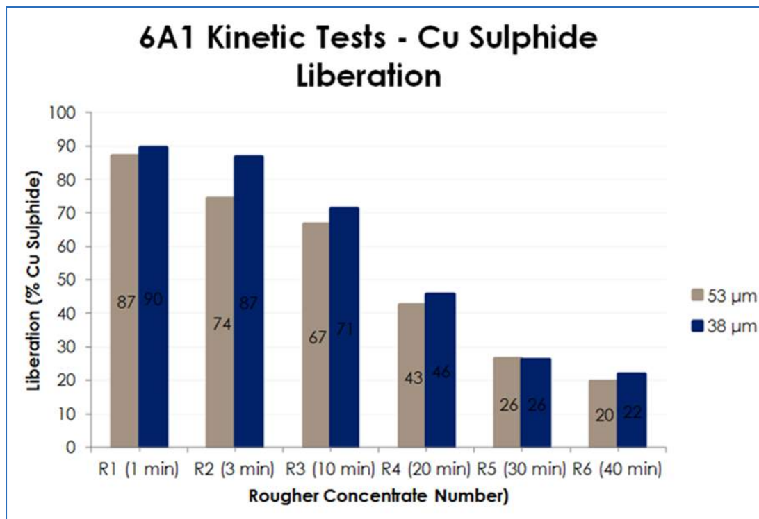
Figure 13.22 Copper Sulphide Liberation in Rougher Flotation
