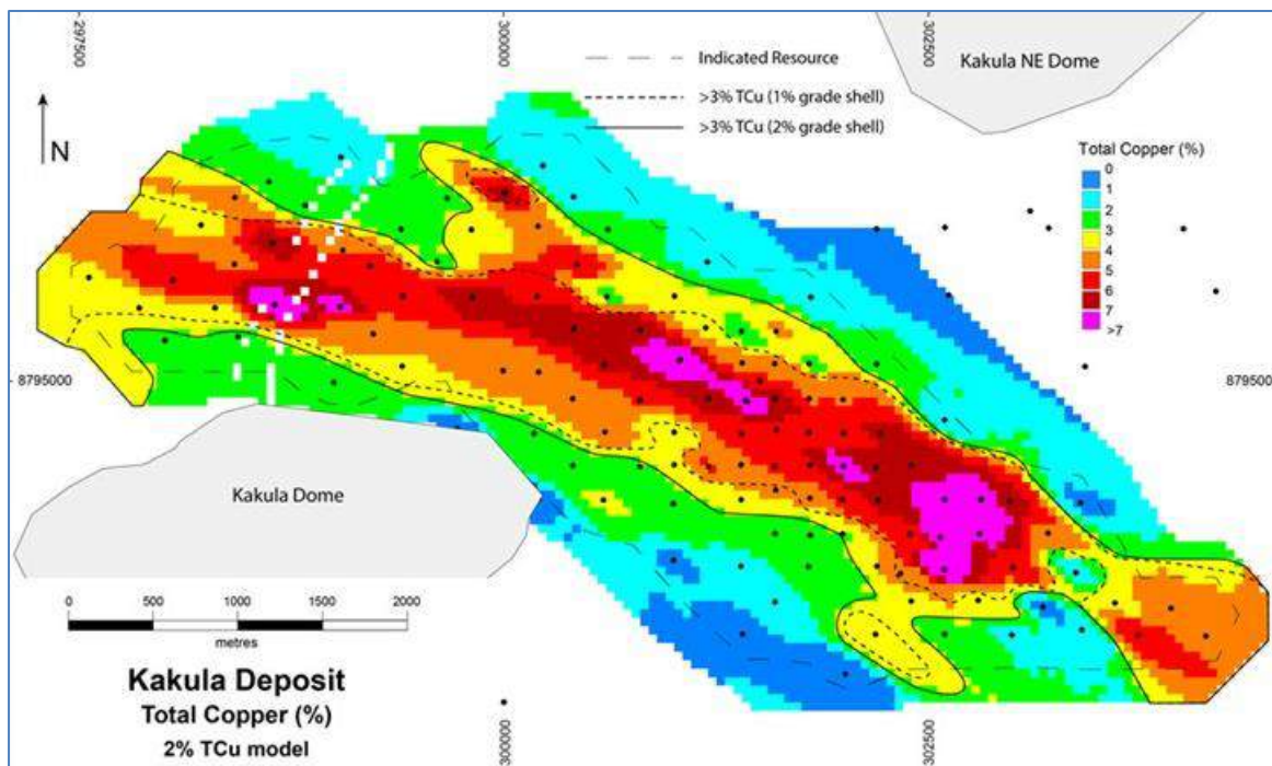
Figure 14.33 Kakula: TCu Grades for the Overall 2.0% TCu Model
