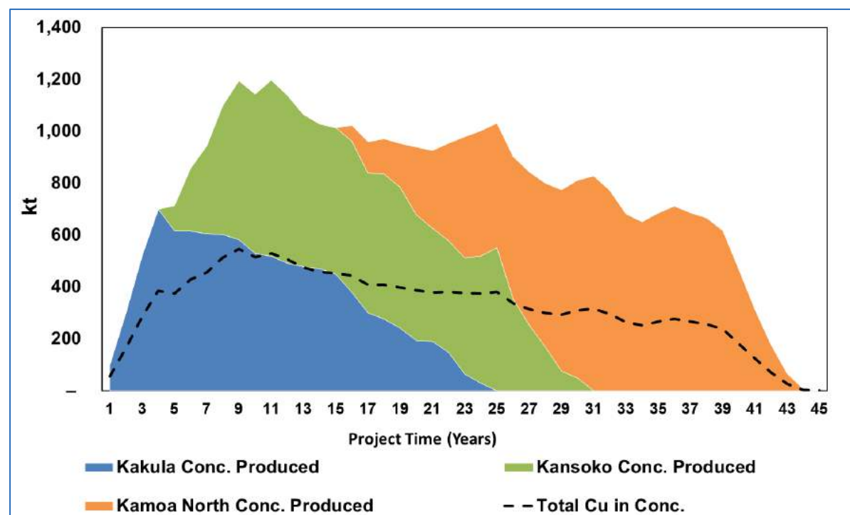
Figure 1.16 Kamoa-Kakula 12 Mtpa PEA Concentrate and Metal Production
