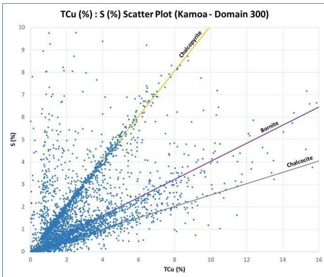
Figure 7.34 Scatter Plot Illustrating Clear Sulphide Species Within the Mineralised Zone at Kamoā. Theoretical TCu: S Ratios for Chalcopyrite (orange), Bornite (purple) and Chalcocite (grey) are Based upon Molar Mass Ratios
