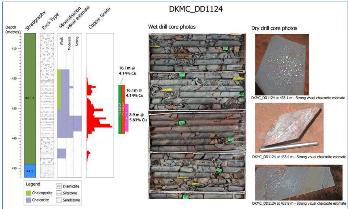
Figure 7.43 Lithological and Mineralisation Styles at Kakula West (from Drillhole DKMC_DD1124)
