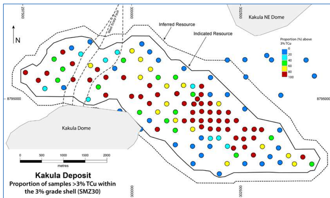
Figure 14.5 Kakula: Proportion of Samples >3% TCu Within the 3% Grade Shell
