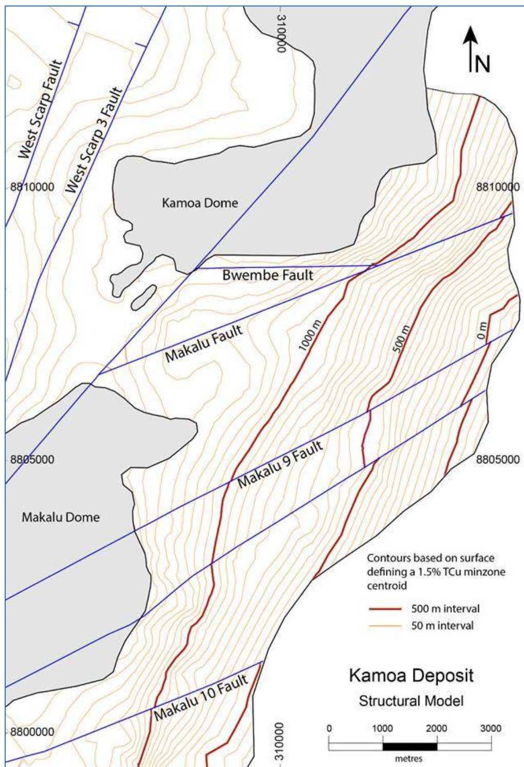
Figure 7.21 Structural Model and 1.5% Minzone Structural Contours (masl) for the Kamoā Deposit
