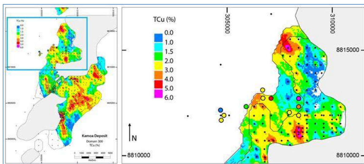
Figure 10.5 Plan View Showing Kamoa Drillholes with Assay Results Completed Since Construction of the 2014 Mineral Resource Model
