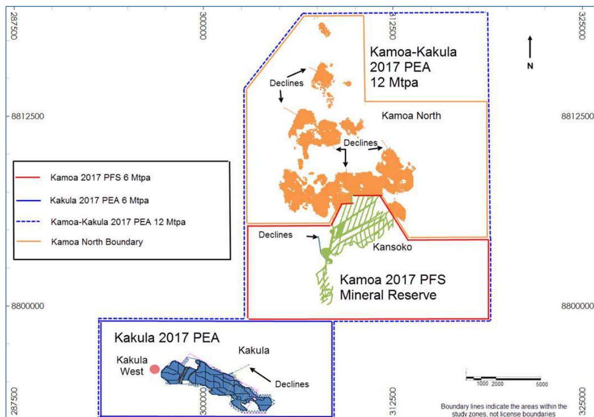
Figure 1.5 Kamoā 2017 PFS and Kamoā-Kakula 2017 PEA Mining Locations
