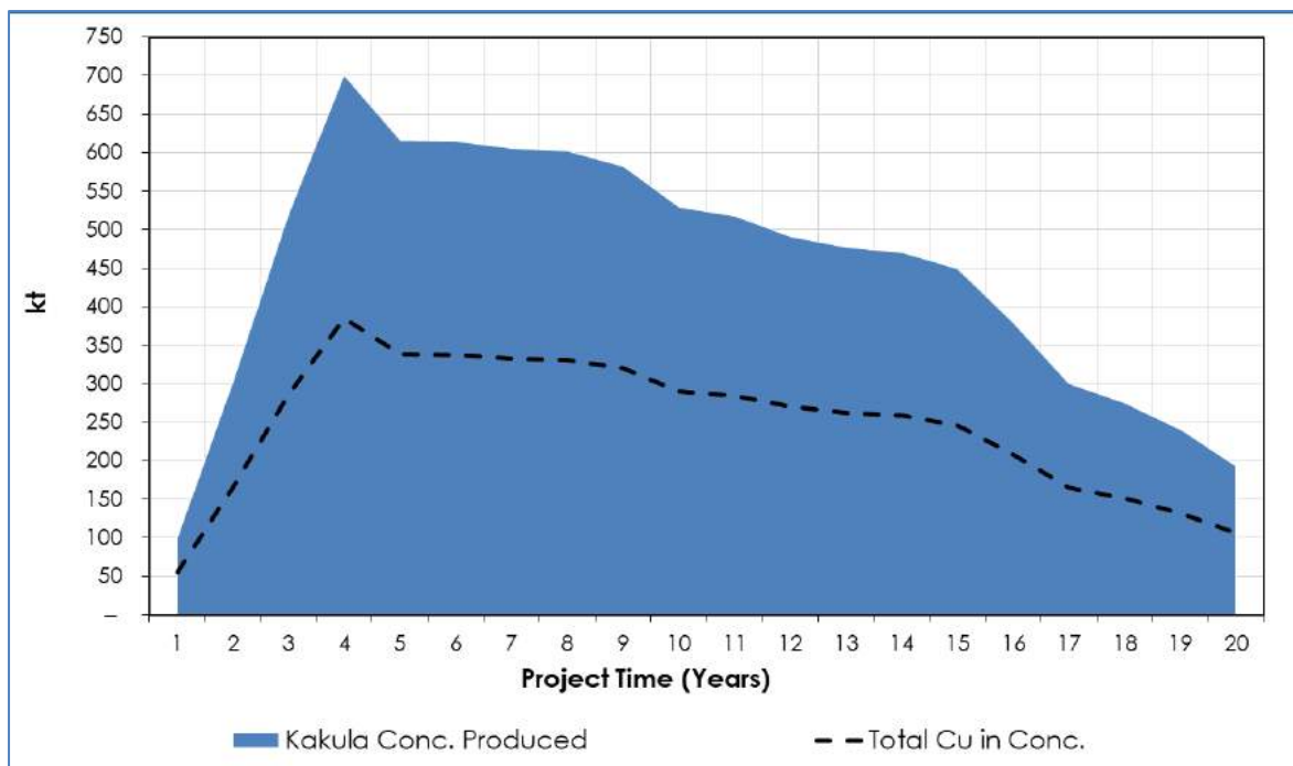
Figure 1.9 Kakula 6 Mtpa PEA Concentrate and Metal Production
