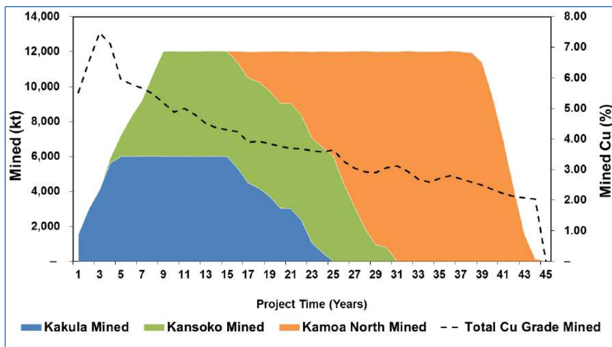
Figure 1.15 12 Mtpa PEA Scenario Mill Feed and Grade Profile
