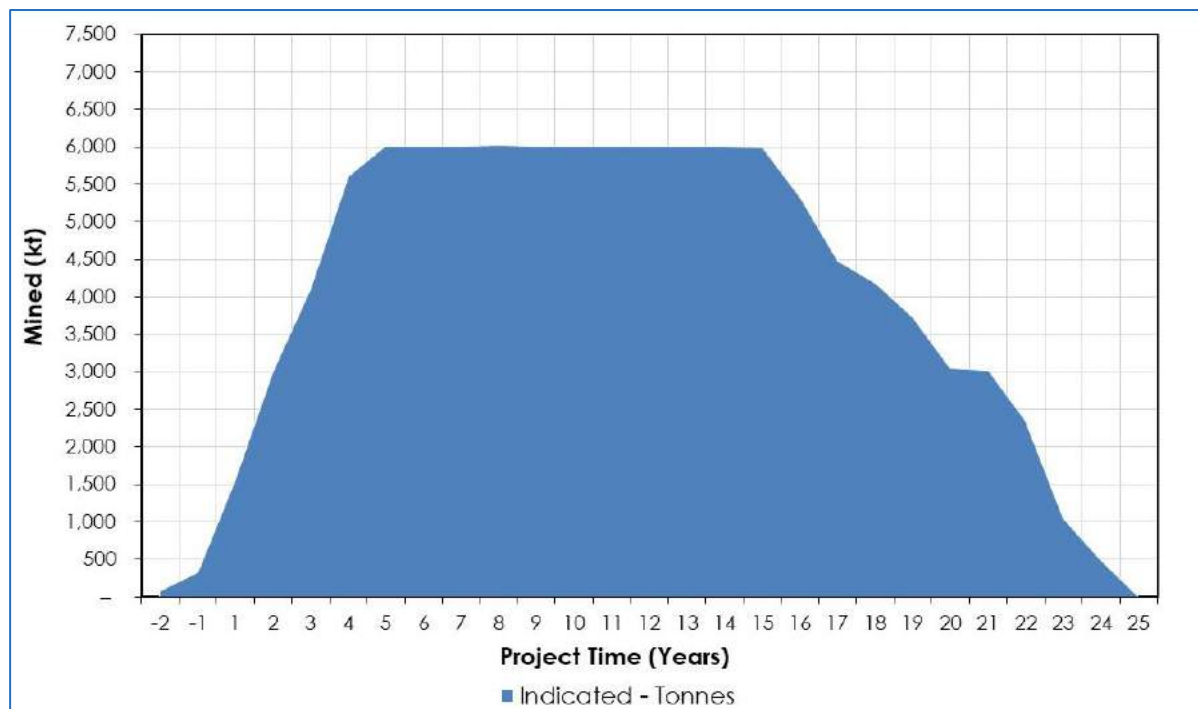
Figure 24.20 Kamoā 2017 PFS Mine Production by Resource Category
