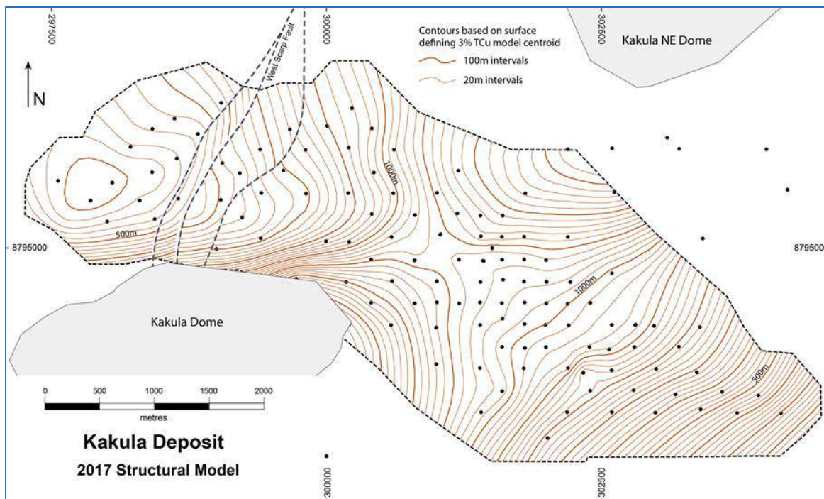
Figure 7.28 Structure Model for the Kakula Resource Area
