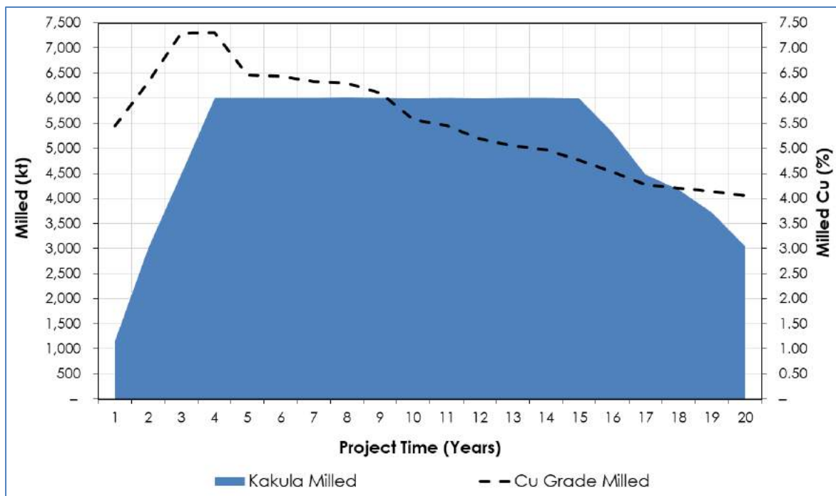
Figure 1.8 Kakula 6 Mtpa PEA Process Production
