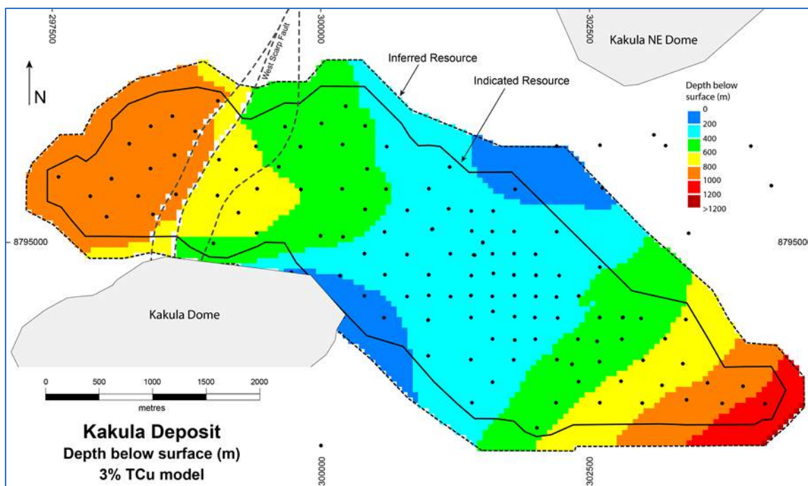
Figure 7.29 Depth Below Surface for the Kakula 3% Copper Grade Shell
