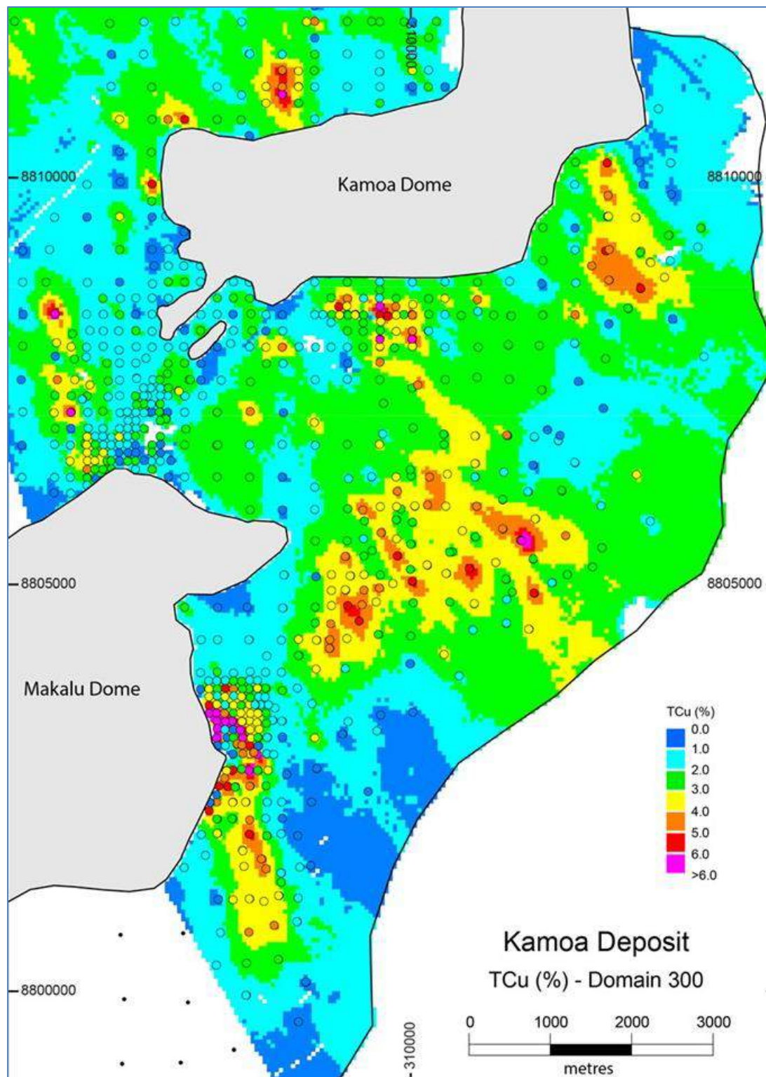
Figure 14.24 Kamoā: Estimated TCu Grade (%) for the Upper SMZ (Domain 300)
