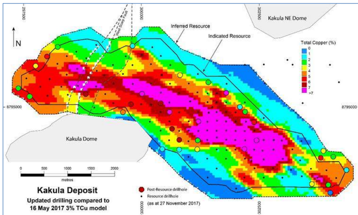
Figure 10.8 Core Drilling Completed at Kakula After 16 May 2017 (as at 27 November 2017)
