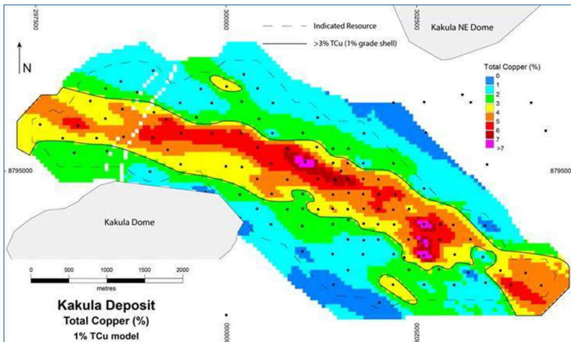
Figure 14.32 Kakula: TCu Grades for the Overall 1.0% TCu Model
