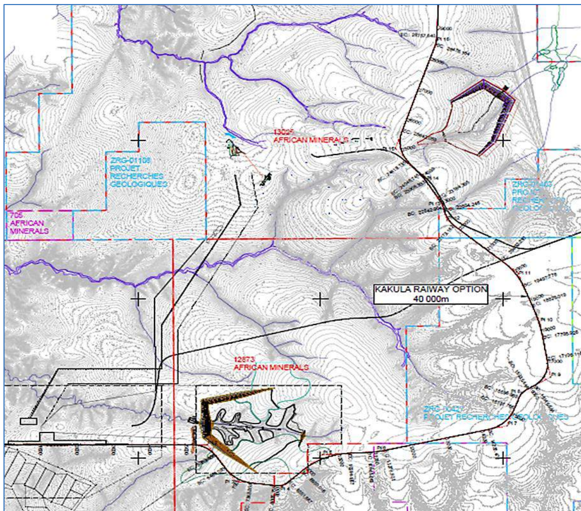
Figure 24.41 Rail from Kakula and Kansoko to Existing Lobito Infrastructure
