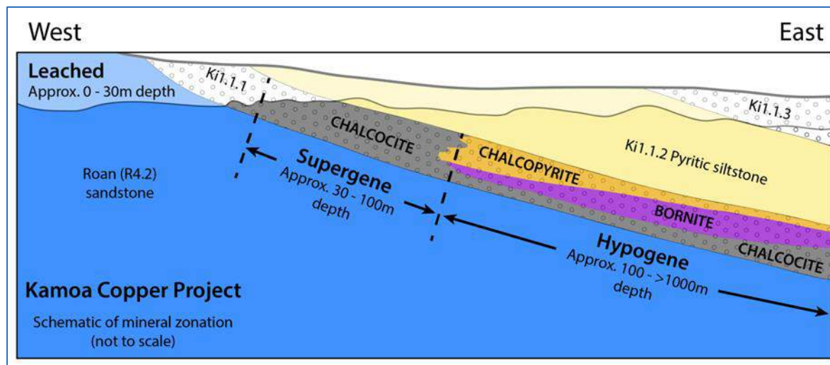
Figure 7.30 Schematic of Mineral Zonation at Kamoā
