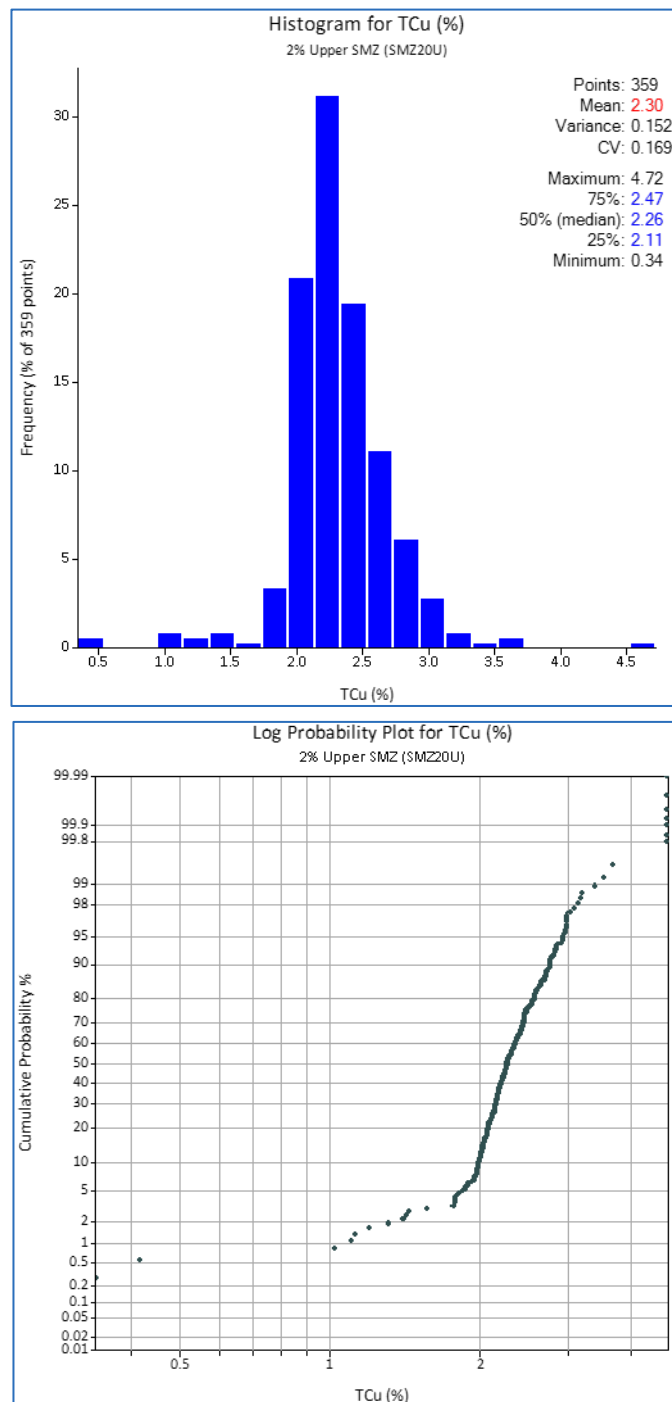
Figure 14.14 Kakula: 1 m Composite TCu (%) for 2.0% TCu Upper Grade Shell (SMZ20U). Histogram and Probability Plot
