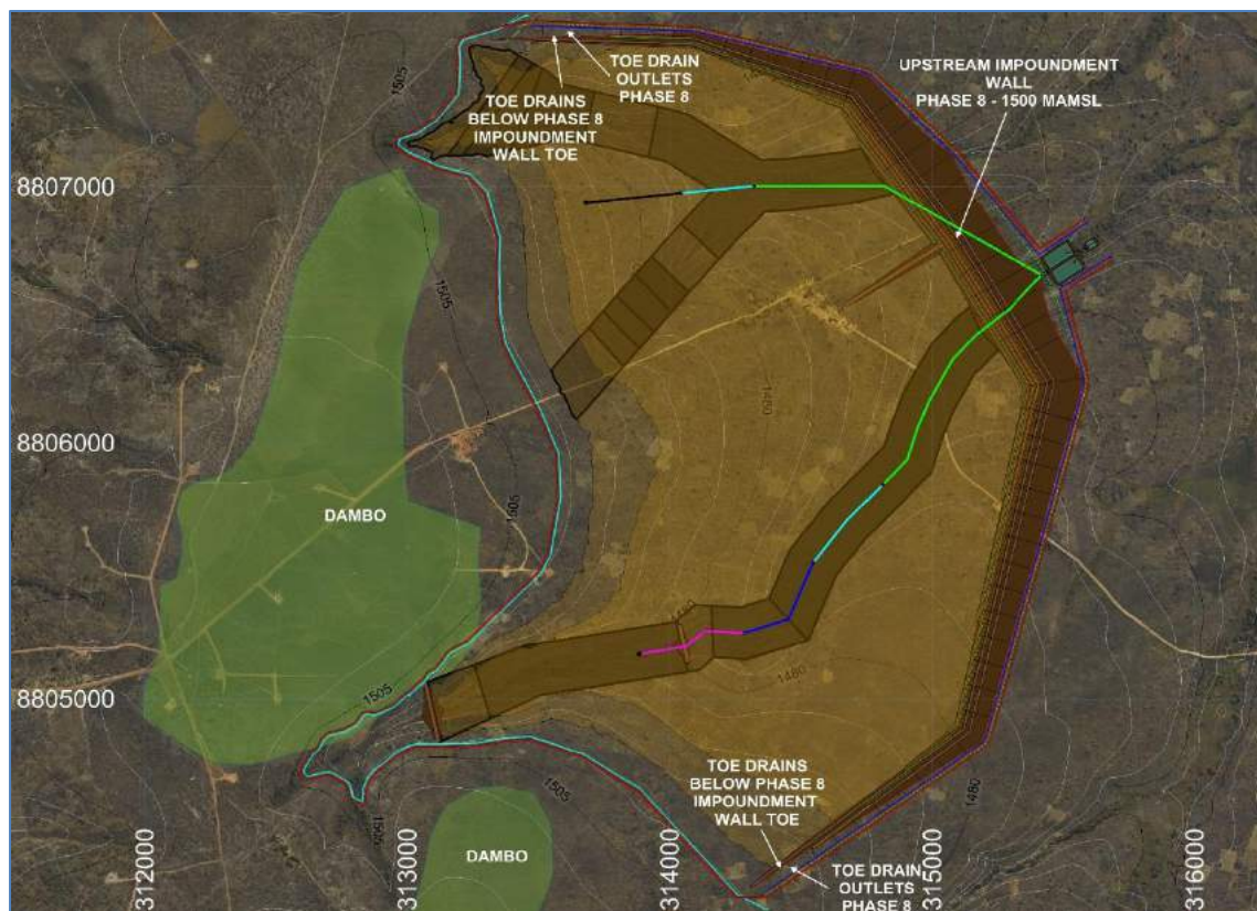
Figure 18.7 General Topography of the Preferred Kamoia TSF Area
