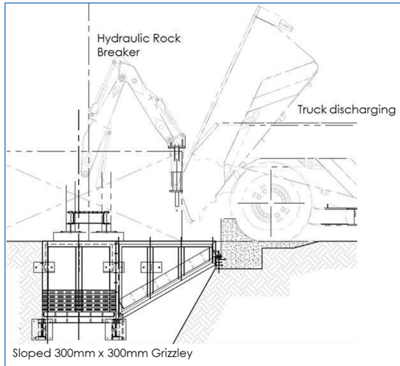
Figure 16.33 Grizzly Layout
