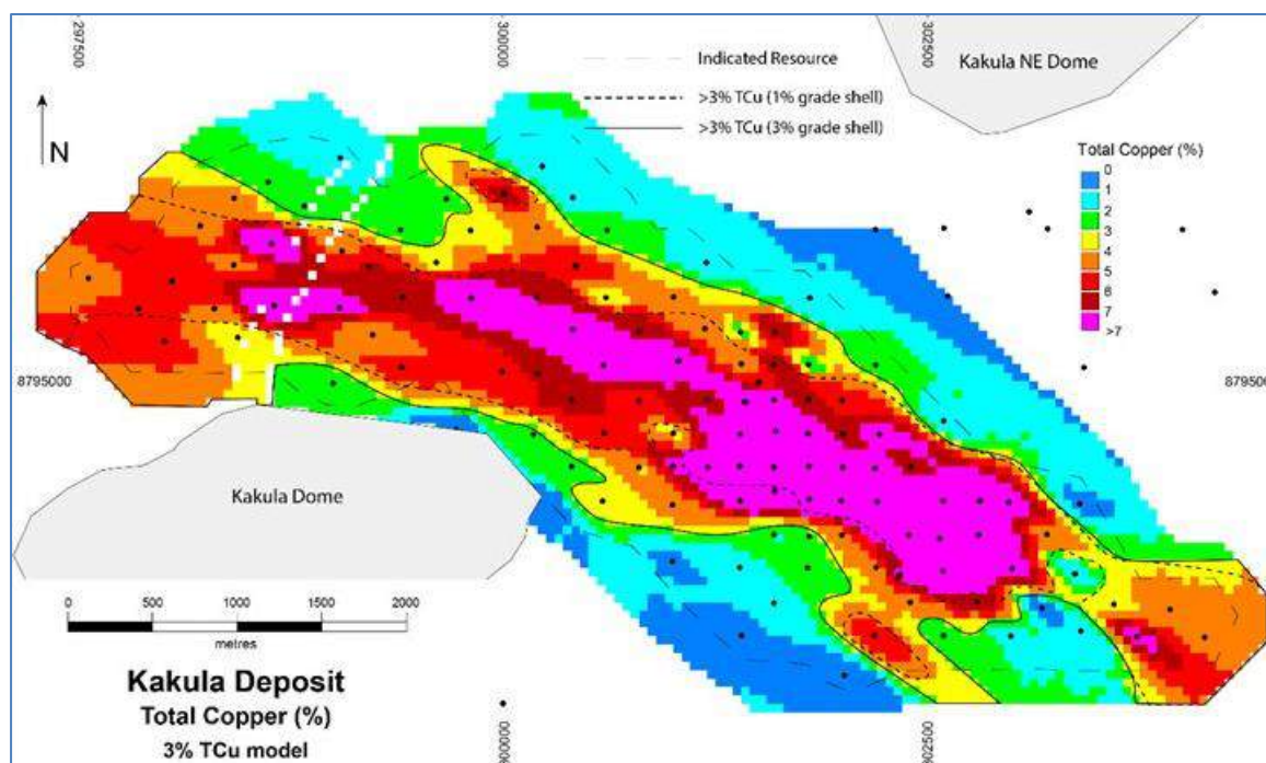
Figure 14.34 Kakula: TCu Grades for the 3.0% TCu Model
