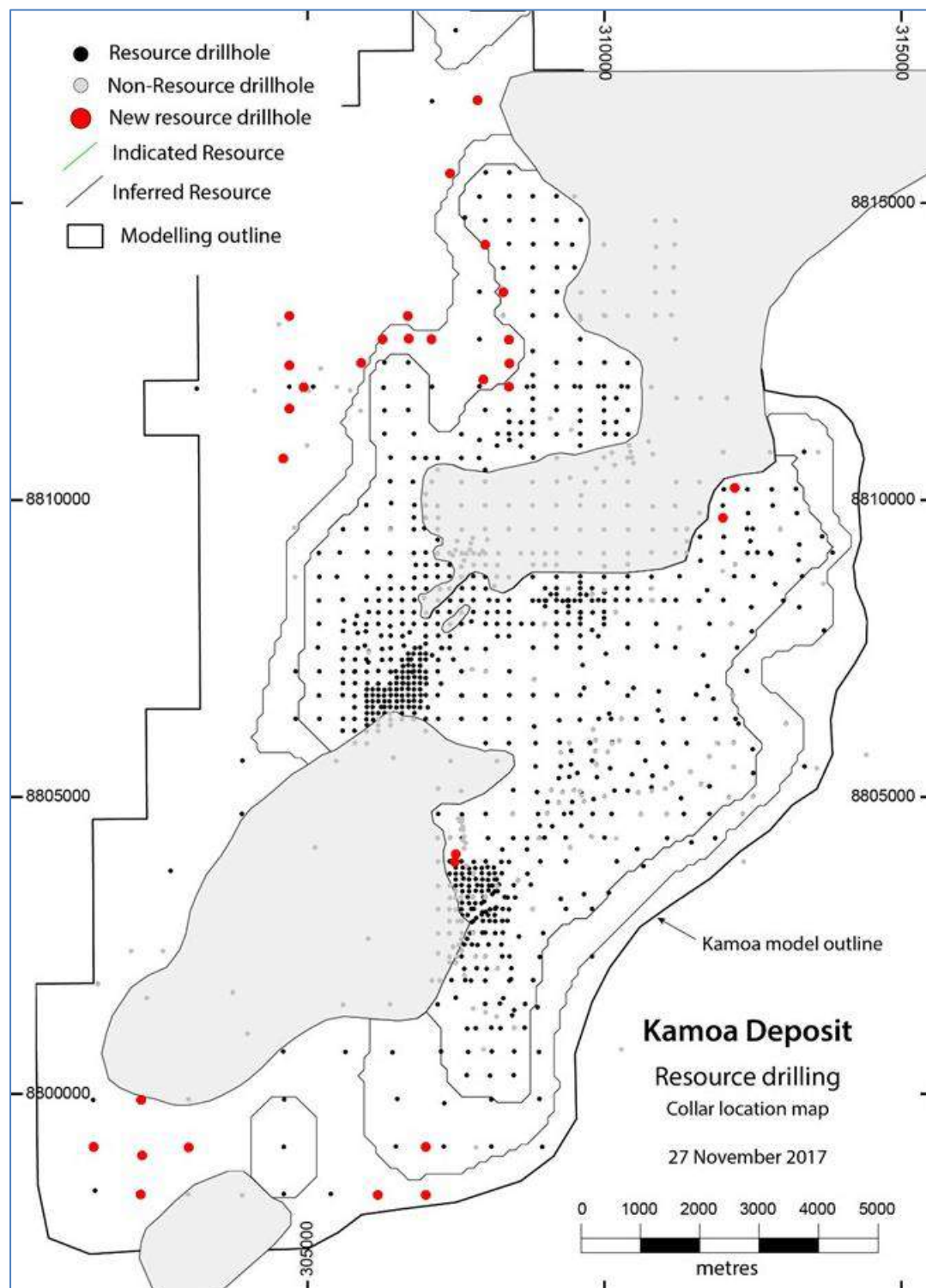
Figure 10.6 Plan View Showing Kamoa Drillholes Completed Since Construction of the 2017 Mineral Resource Model
