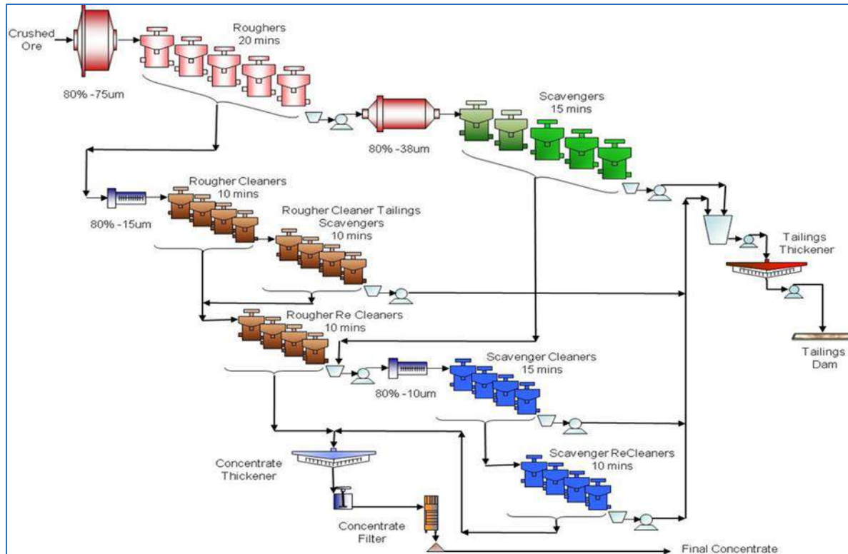
Figure 13.4 XPS Frozen Flowsheet
