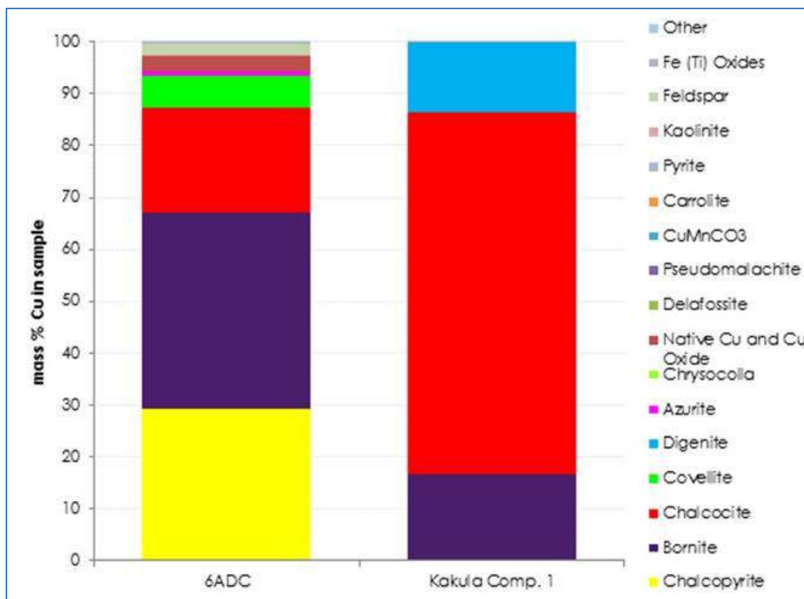
Figure 13.27 Cu Deportment Comparison Between Kamoia 6ADC and Kakula Composite 1
