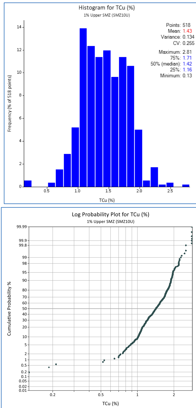
Figure 14.13 Kakula: 1 m Composite TCu (%) for 1.0% TCu Upper Grade Shell (SMZ10U). Histogram and Probability Plot
