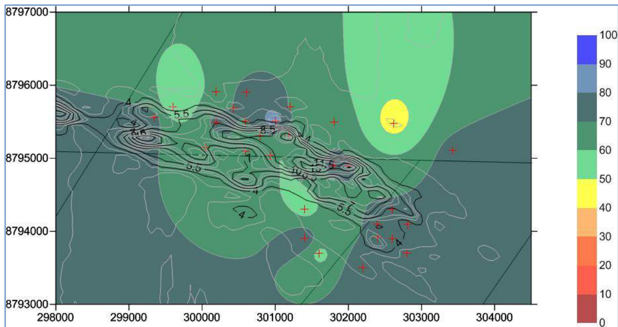
Figure 16.8 RMR B89 Contour Map for the Hanging (based on IRS from field estimates)
