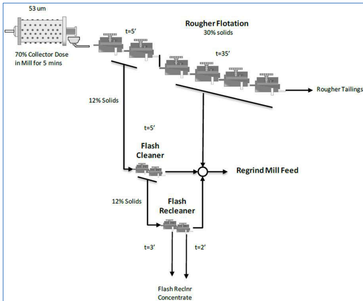
Figure 13.16 Truncated XPS IFS4α Circuit
