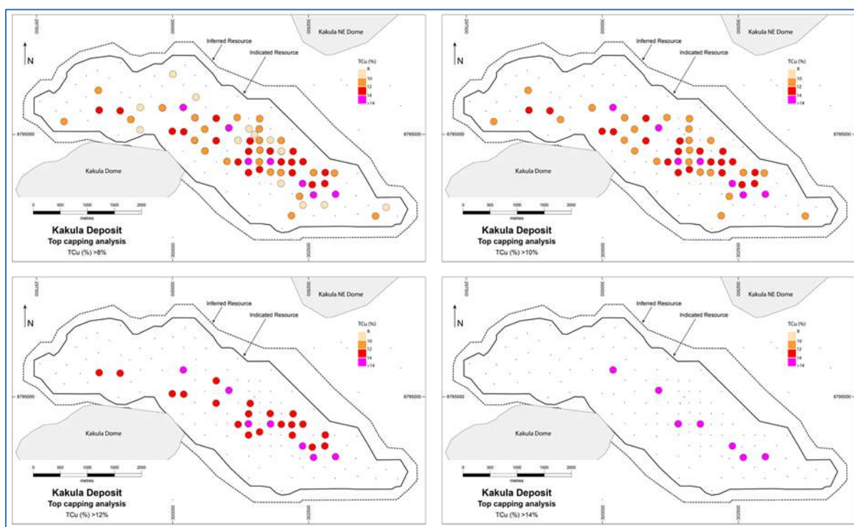
Figure 14.7 Kakula: Visual Top Capping Analyses with TCu grades >8%, >10%, 12%, and >14%
