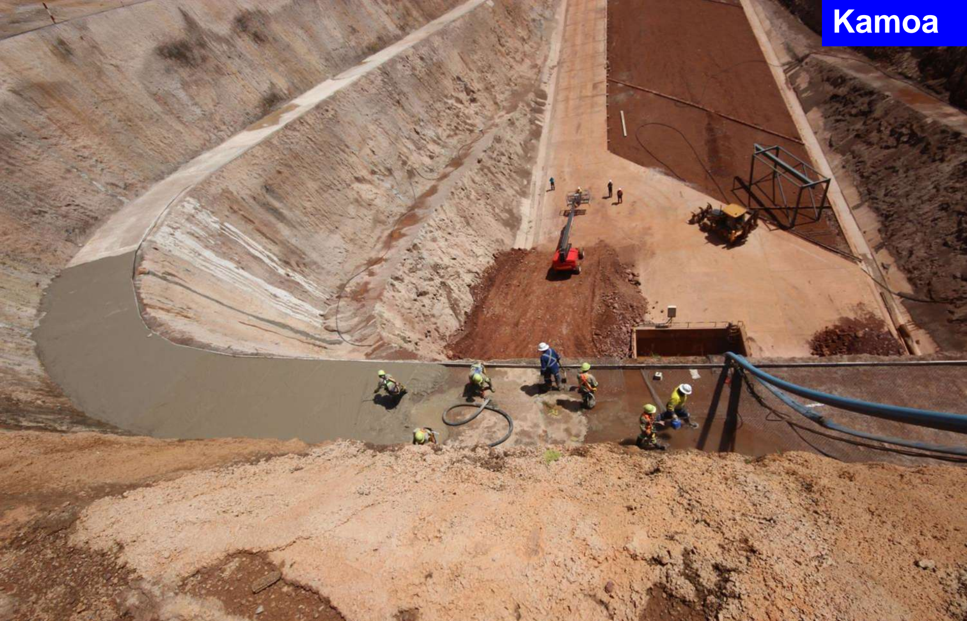
Pouring concrete on the second bench of the Kamoa box cut
