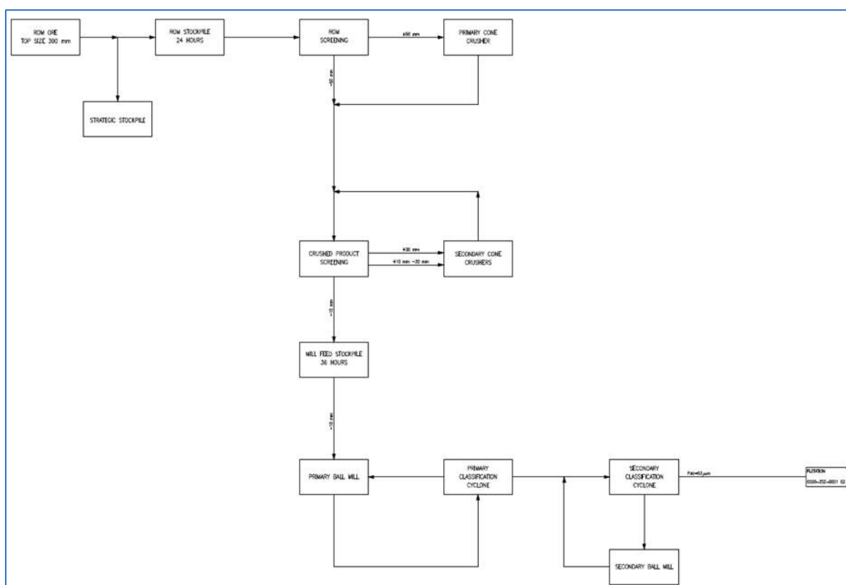
Figure 17.1 Kansoko Crushing and Milling
