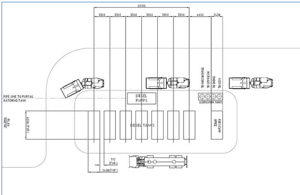
Figure 16.17 Surface Diesel and Lubrication Storage Facility
