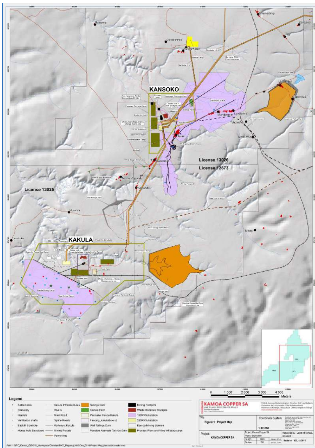
Figure 24.40 Site Plan
