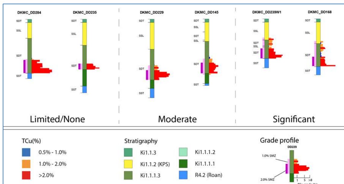
Figure 14.32 Kamoā: Impact of the Adjustments in SMZ Coding for Different Grade Profiles
