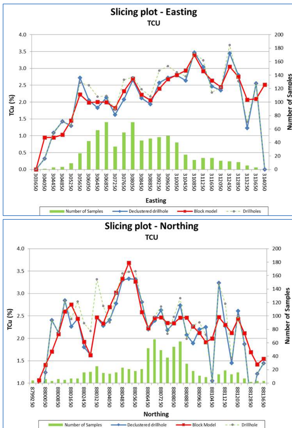
Figure 14.29 Kamoā: Swath Plots for TCu (%) for the 1.0% TCu Cut-off Model (SMZ10)
