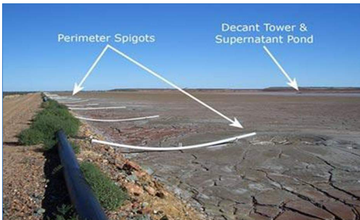
Figure 18.11 Multiple Spigot Discharge
