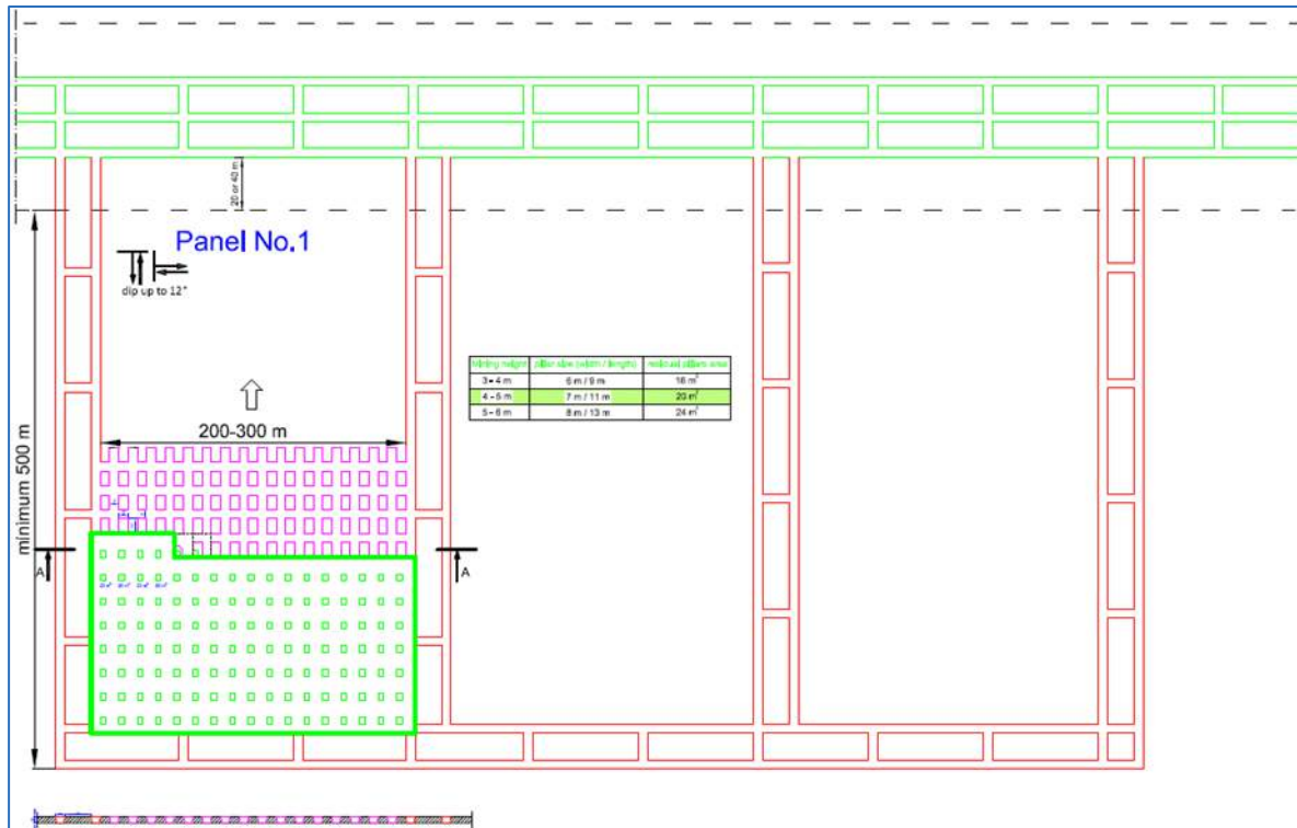
Figure 24.28 Controlled Convergence Panel Design (0° to 12° Dip)
