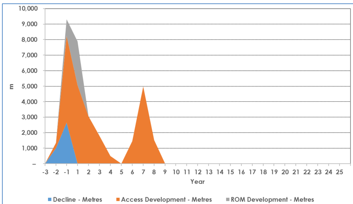
Figure 24.16 Kakula Mine Development
