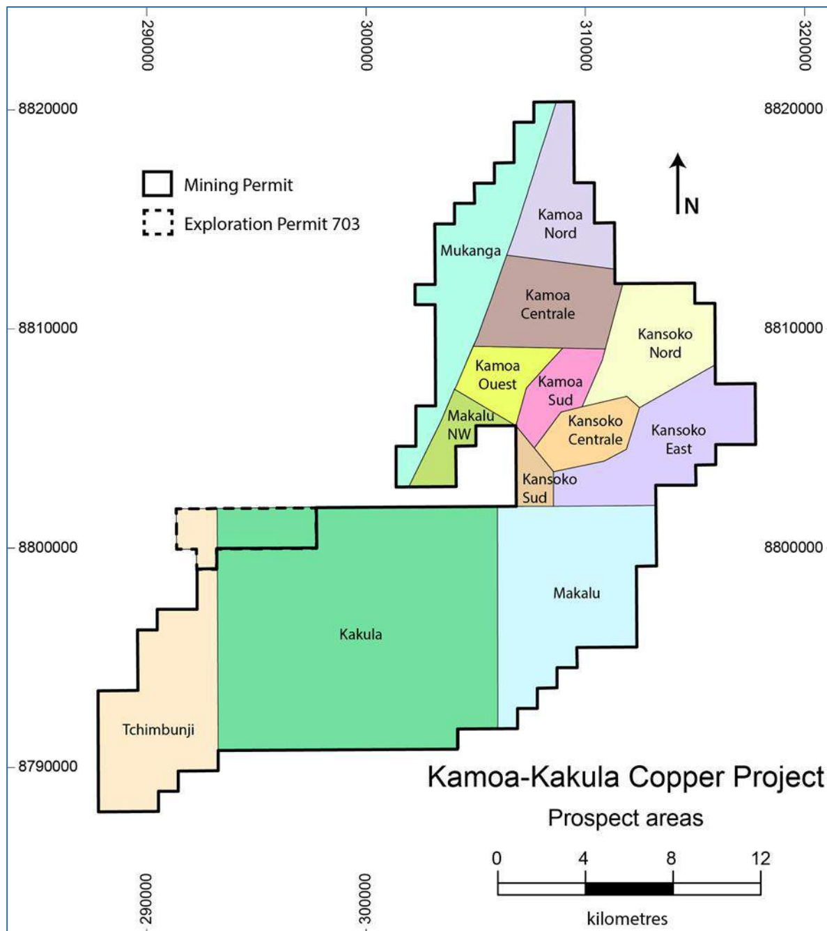
Figure 7.4 Prospect Areas within the Combined Exploitation Permits
