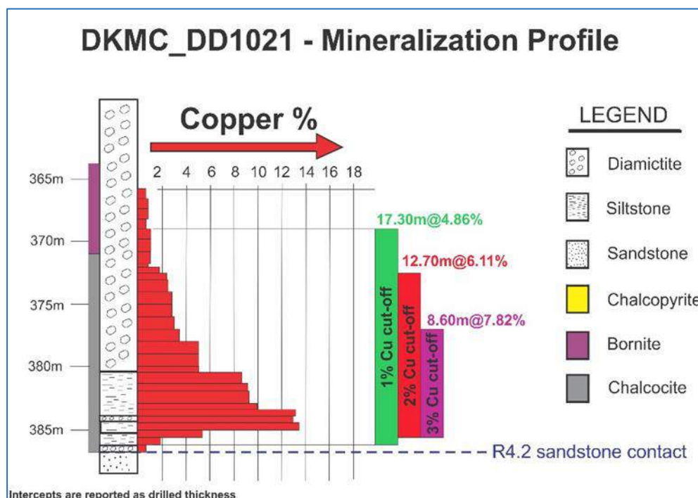
Figure 7.36 The Impact of Lithology on the Characteristics of the Grade Profile
