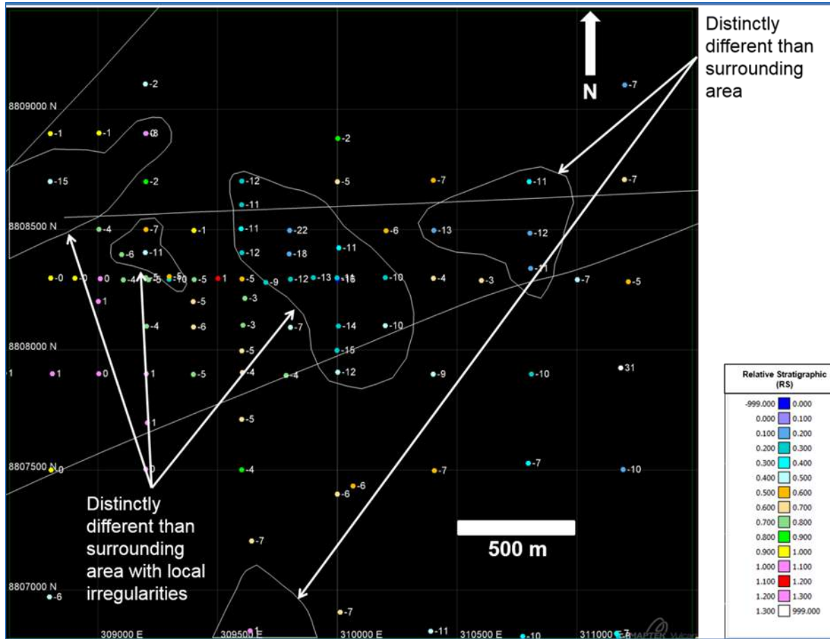
Figure 7.44 Stratigraphic Position of SMZ10 with Respect to the base of the KPS
