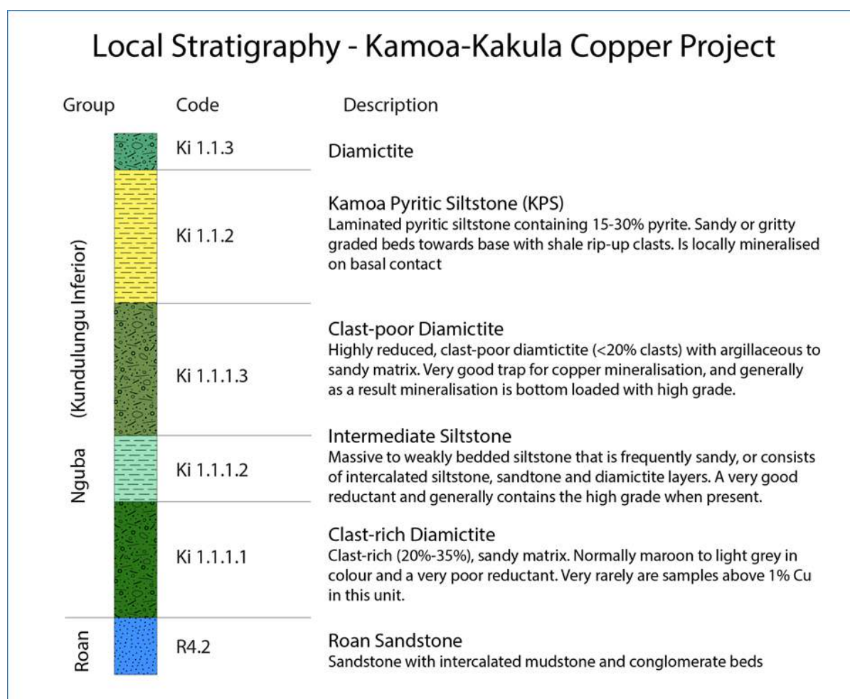
Figure 7.5 Local Stratigraphy for the Kamoa-Kakula Project
