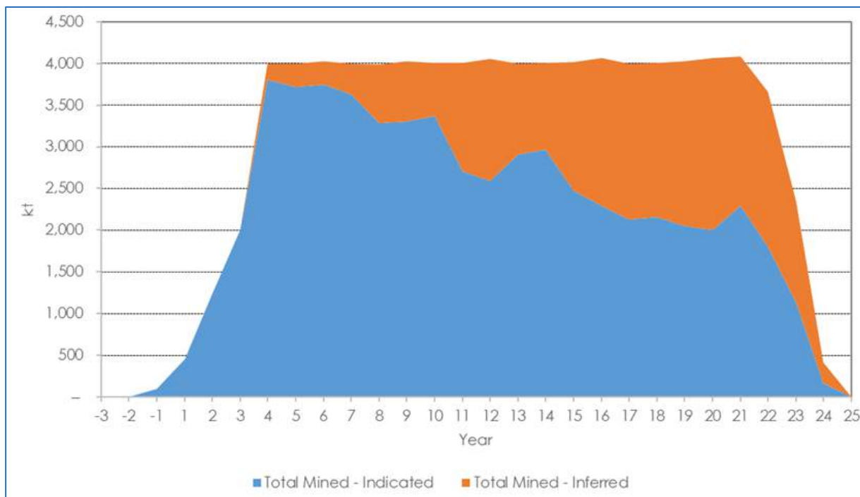
Figure 24.17 Kakula Mined by Resource Category
