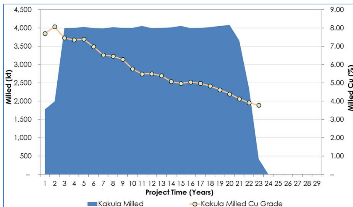
Figure 24.20 Kakula 4 Mtpa Processing
