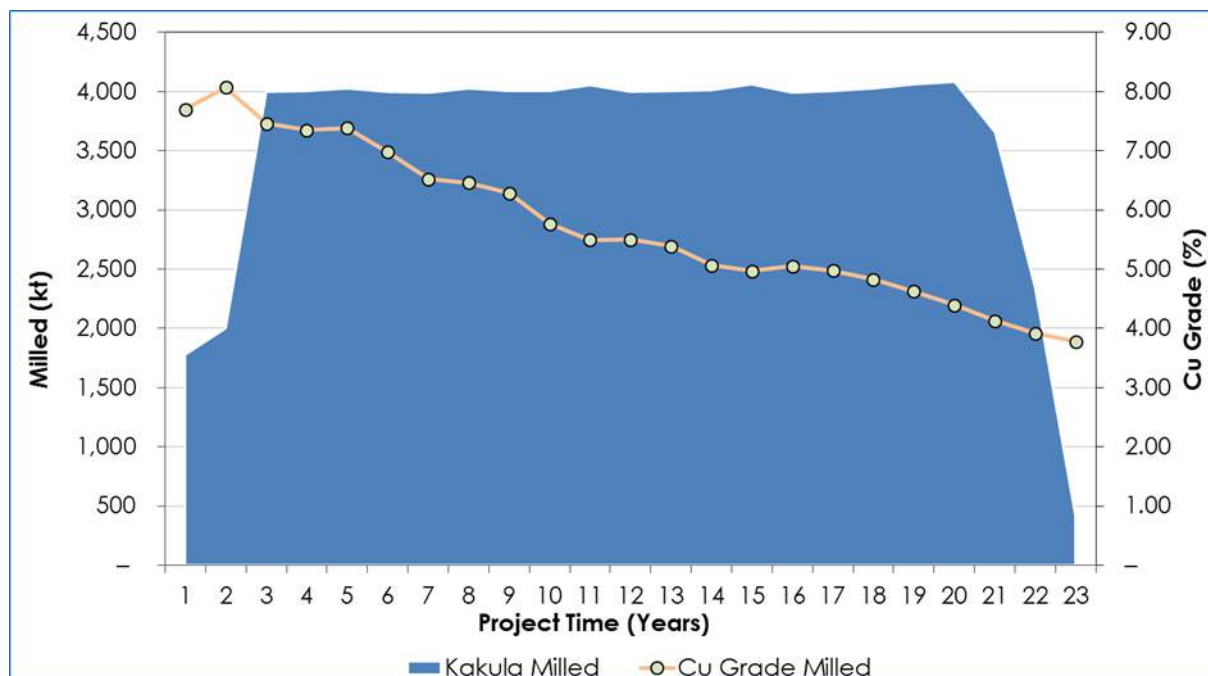
Figure 1.5 Processing – 4 Mtpa Production Scenario
