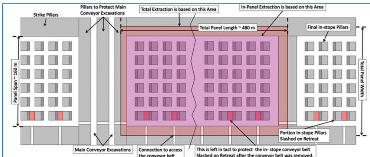
Figure 16.4 Typical Room and Pillar Layout
