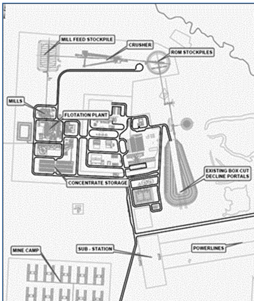
Figure 24.35 Kansoko Site Conceptual Concentrator
