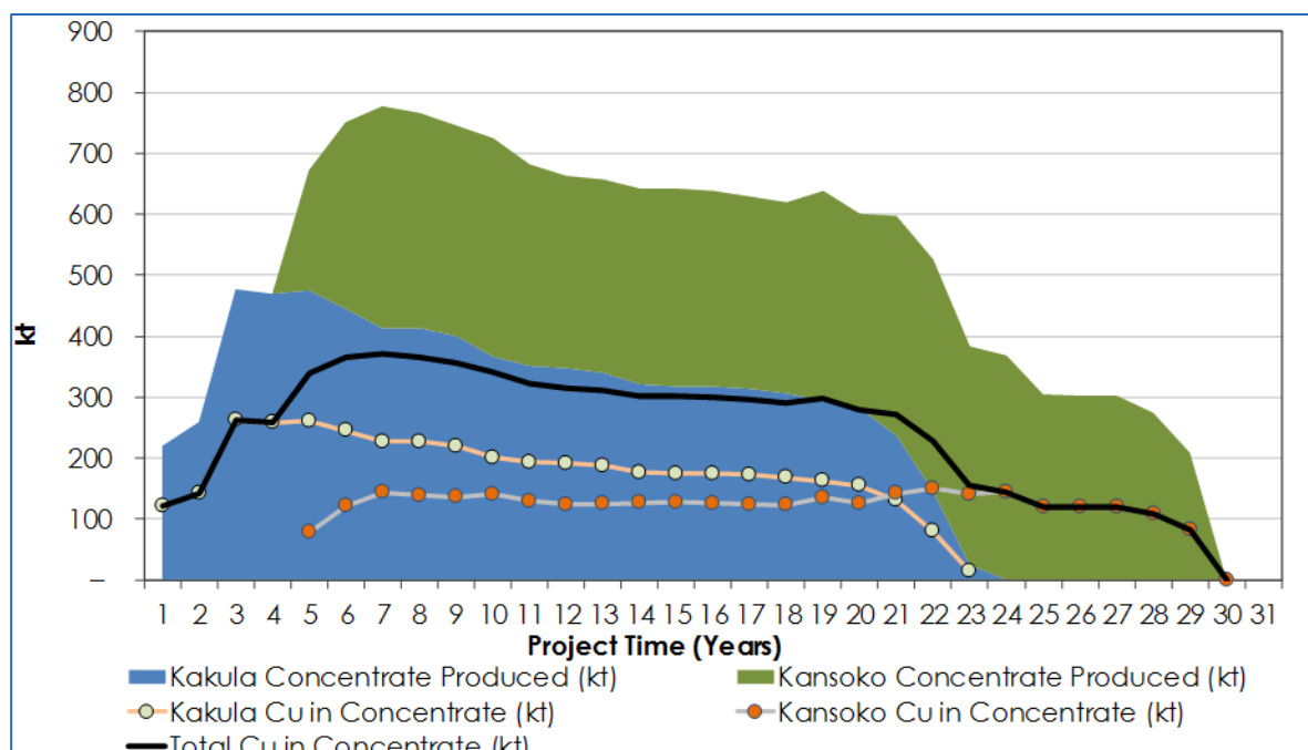
Figure 24.13 Concentrate and Metal Production – 8 Mtpa Production Scenario
