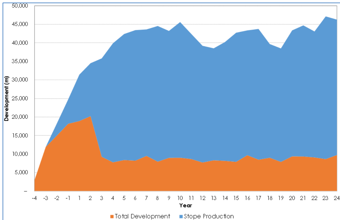
Figure 16.20 Kamoā 2016 PFS Development
