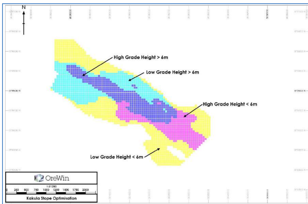
Figure 24.26 Stope Optimisation Blocks by Height
