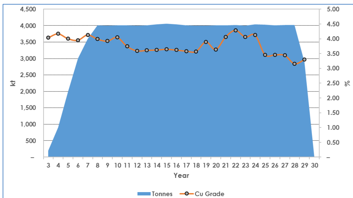
Figure 24.18 Kansoko Mine Production
