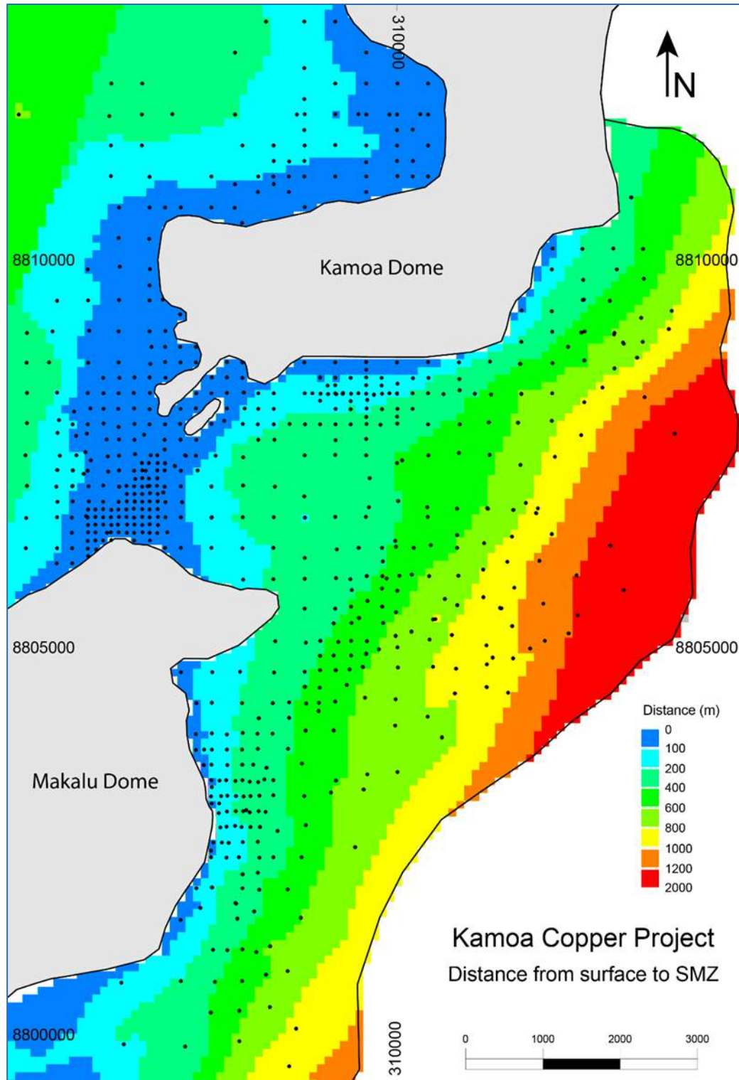
Figure 14.19 Kamoā: Depth of SMZ (Metres below Surface)
