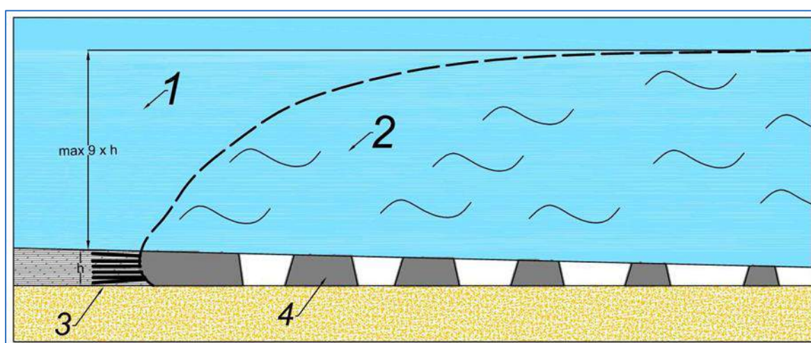
Figure 16.24 Controlled Convergence Rock Mass Impact
