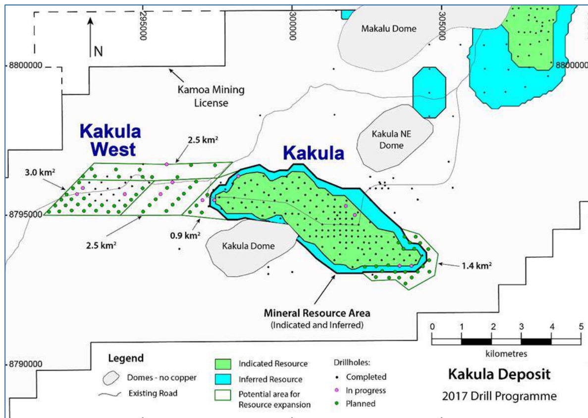
Figure 26.1 Kakula Provisional Drill Programme
