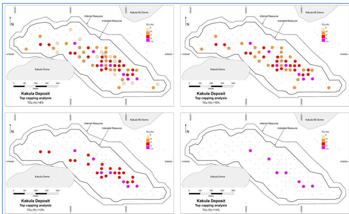
Figure 14.4 Kakula: Visual Top Capping Analyses with TCu grades >8%, >10%, 12% and >14%
