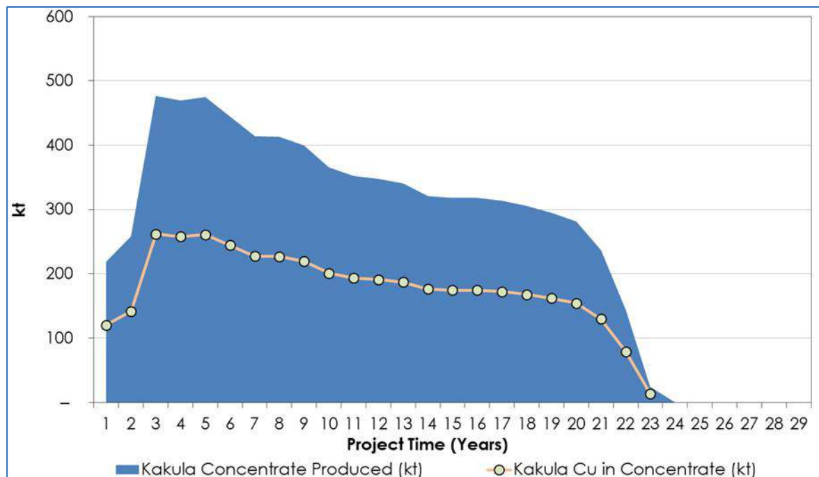
Figure 24.21 Kakula Concentrate Produced
