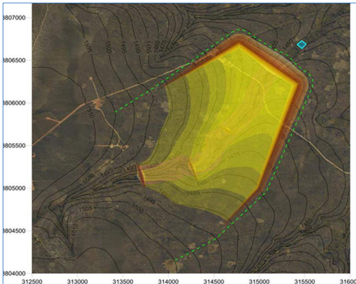
Figure 18.8 Development of the Kamoia Copper TSF at Final Elevation
