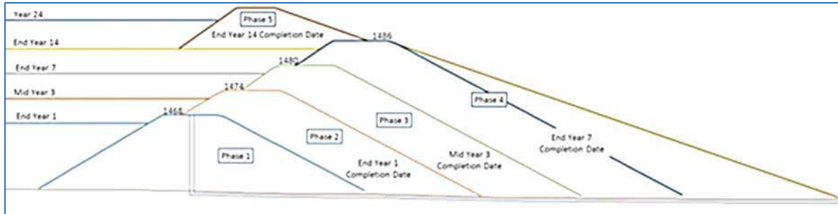
Figure 18.6 Converting to Upstream Facility in Phase 5
