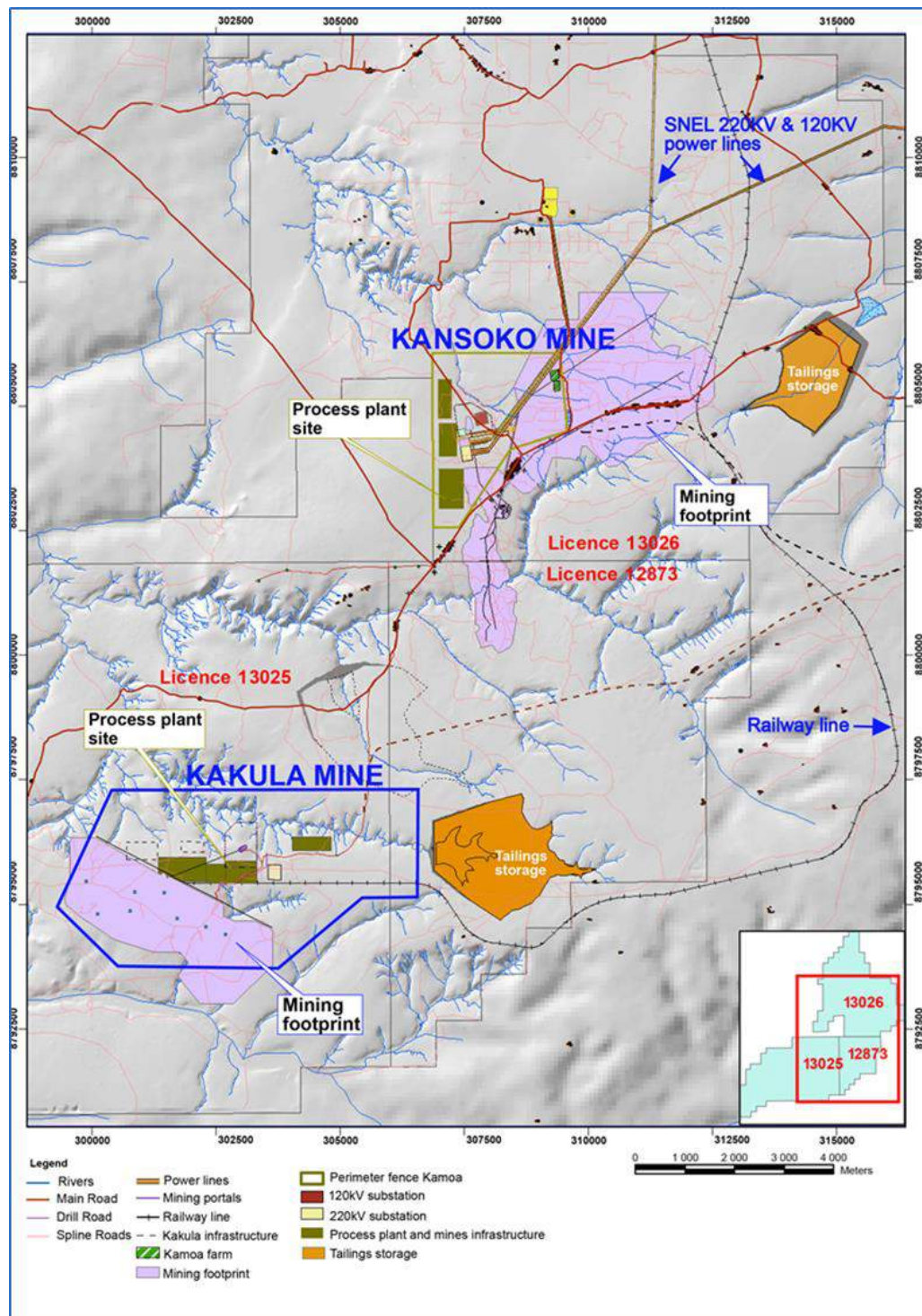
Figure 1.3 Planned Kakula 2016 PEA Development and Infrastructure for Kakula and Kansoko Mines
