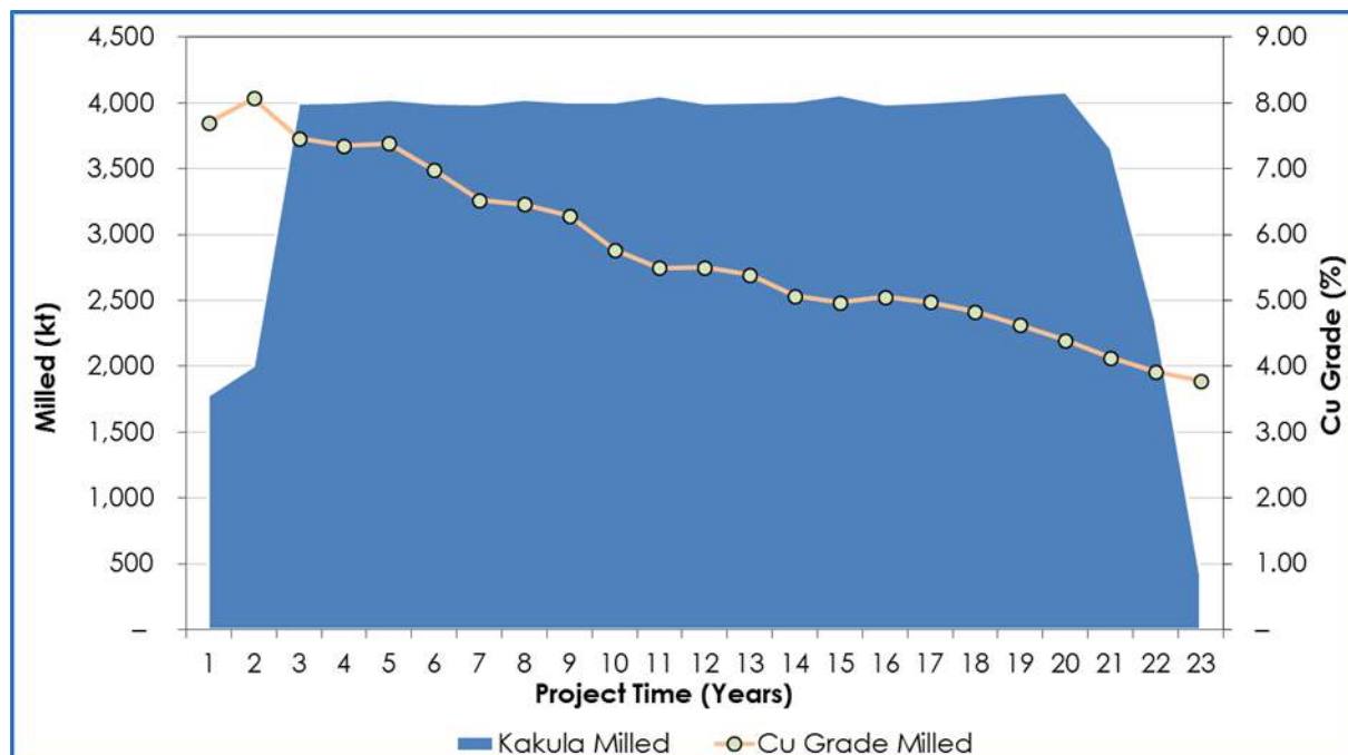
Figure 24.4 Processing – 4 Mtpa Production Scenario
