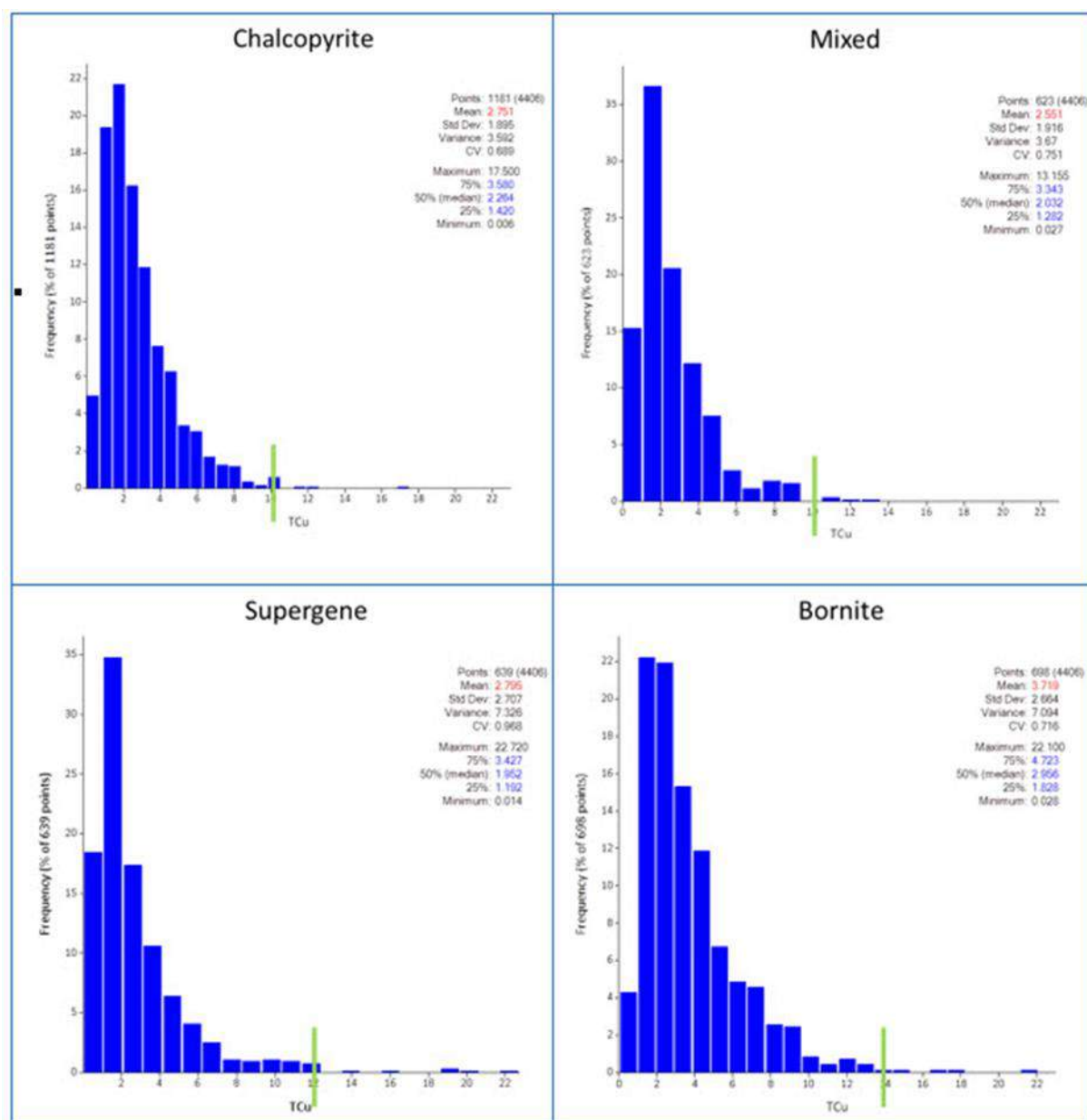
Figure 14.3 Kamoā: Example Histograms of Top Capping Selection for the Mineral Zones
