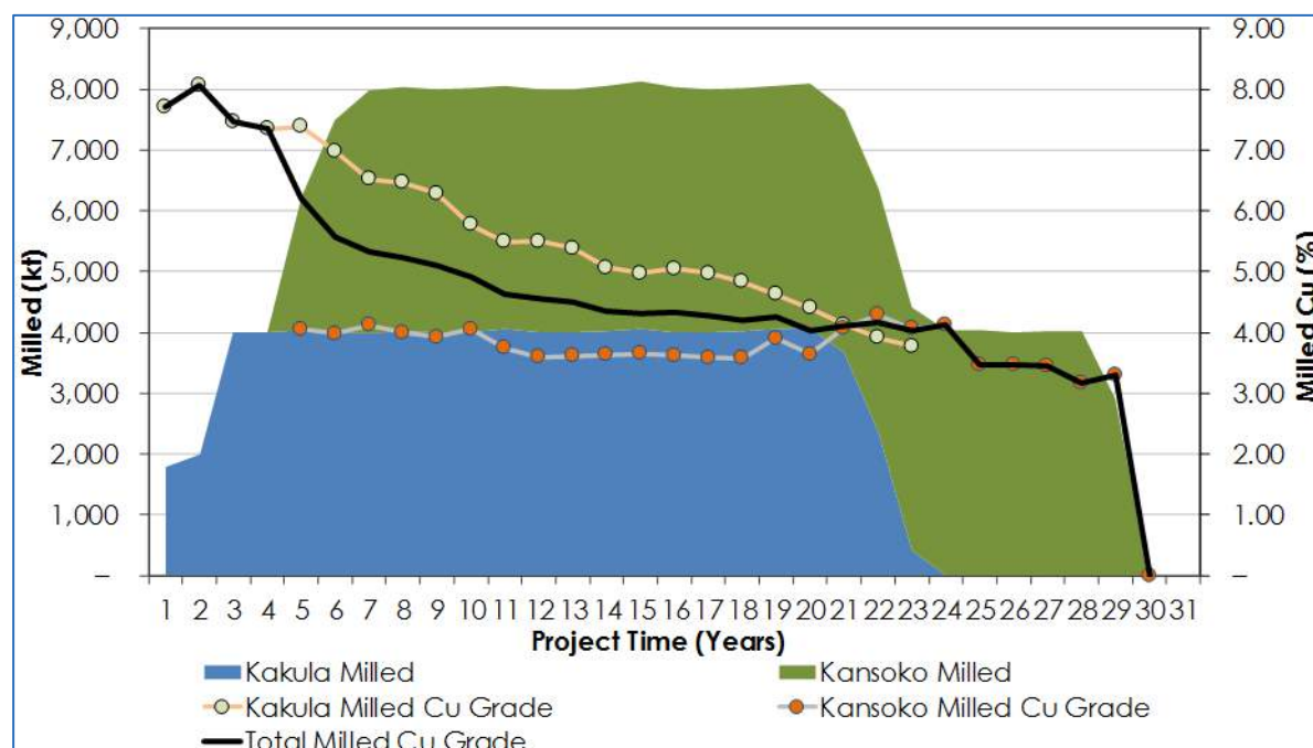
Figure 24.12 Processing – 8 Mtpa Production Scenario
