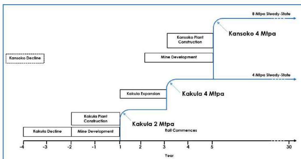
Figure 1.12 Kakula and Kansoko 8 Mtpa PEA Development Scenario
