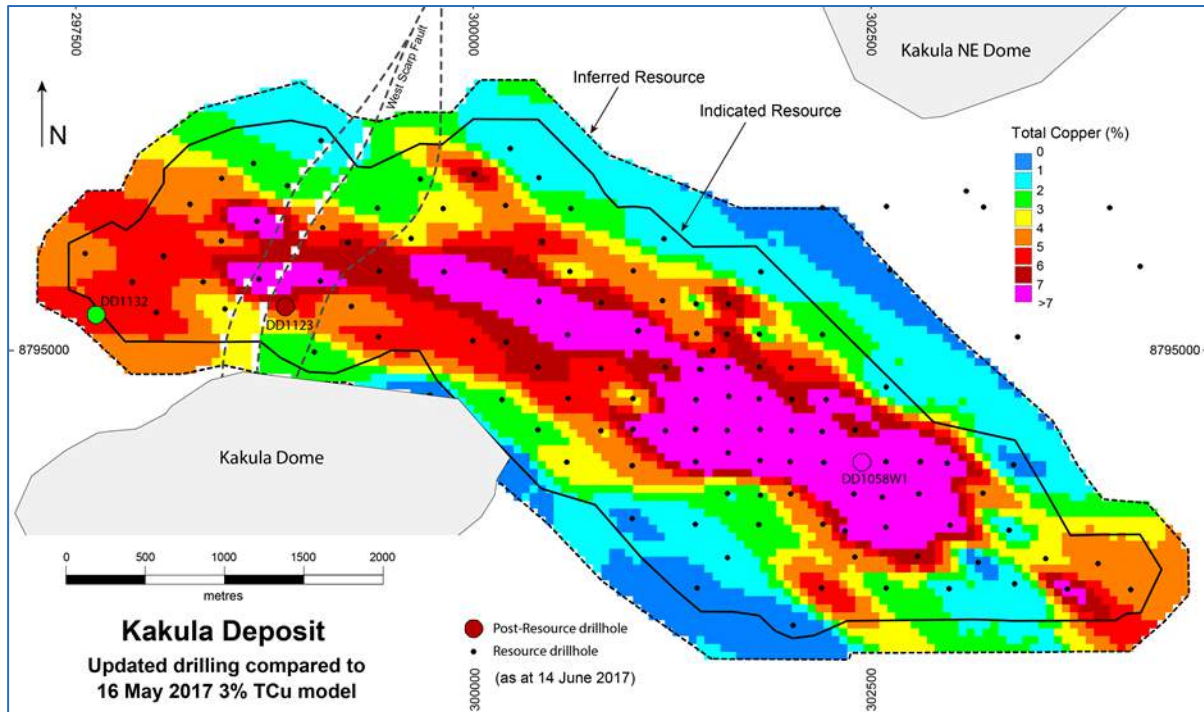
Figure 10.8 Core Drilling Completed at Kakula After 16 May 2017 (as at 14 June 2017)
