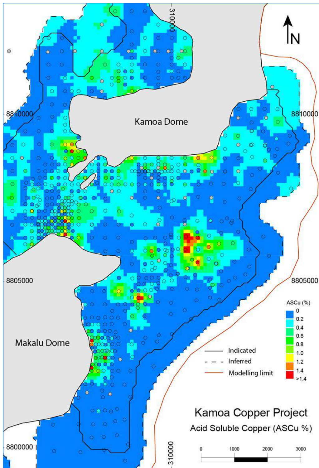
Figure 14.23 Kamoa: Estimated ASCu Grade (%) for a 1.0% TCu Modelling Cut-off (SMZ10)
