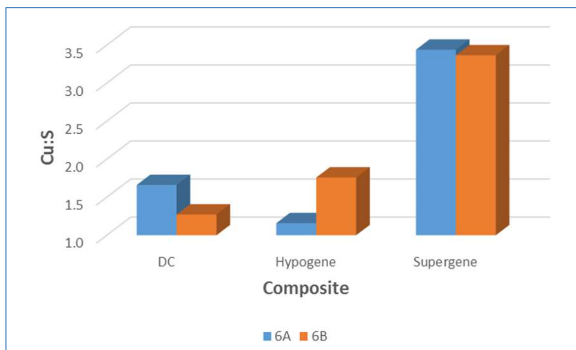
Figure 13.8 Copper to Sulphur Ratios in Phase 6 Composites
