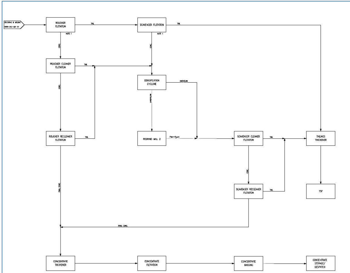
Figure 24.32 Kakula Flotation Circuit
