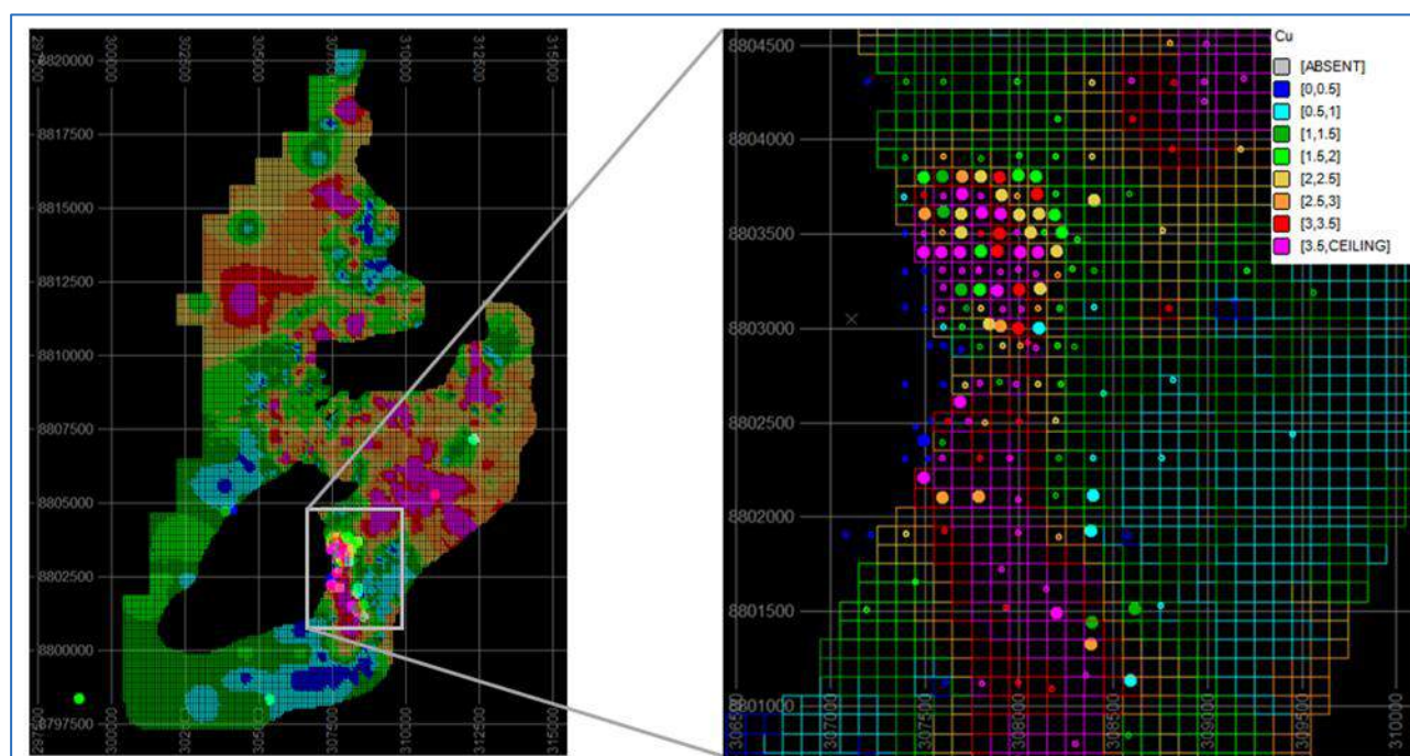
Figure 10.5 Plan View Showing Kamoa Drillholes with Assay Results Completed Since Construction of the 2014 Mineral Resource Model
