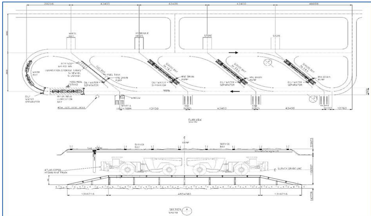
Figure 16.15 Underground Satellite Workshop
