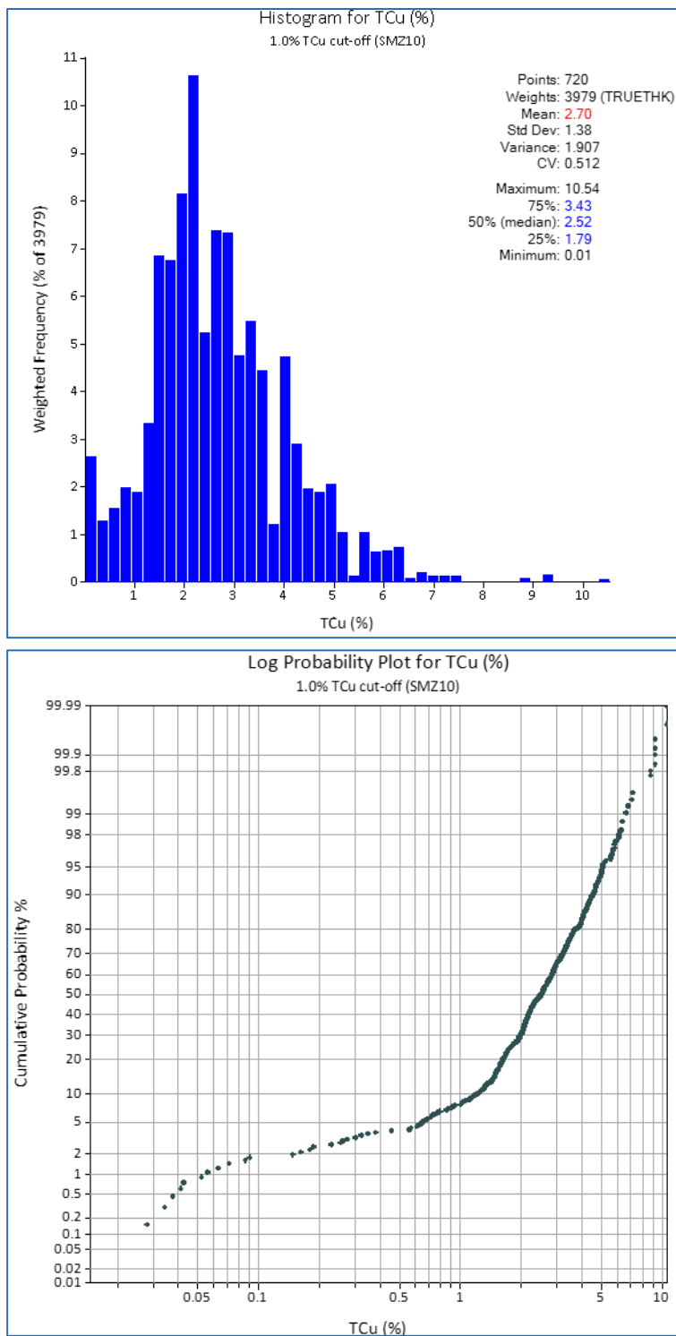
Figure 14.5 Kamoa: Capped Composite TCu (%) for SMZ10 (1.0% TCu Cut-off)
