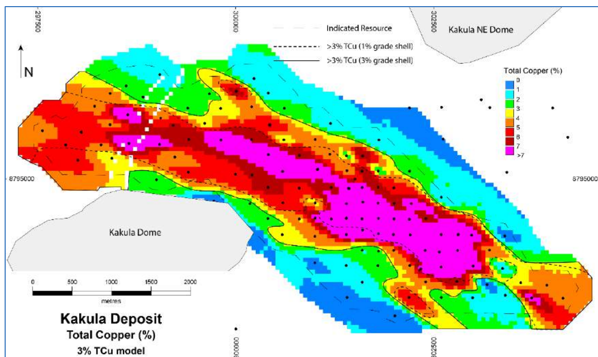
Figure 14.39 Kakula: TCu Grades for the 3.0% TCu Model
