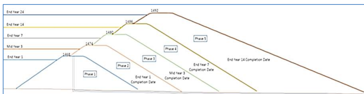
Figure 18.9 Impoundment Wall Phasing
