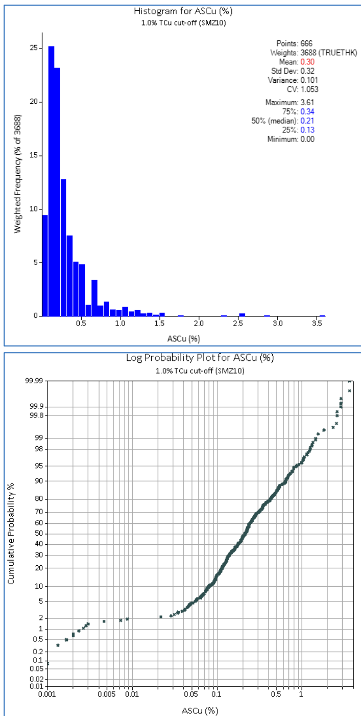
Figure 14.6 Kamoa: Capped Composite ASCu (%) for SMZ10 (1.0% TCu Cut-off)
