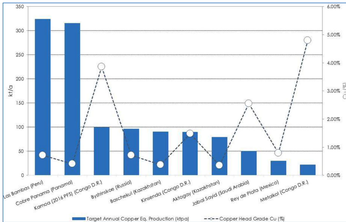
Figure 22.4 Copper Projects Under Construction Concentrate Equivalent Production
