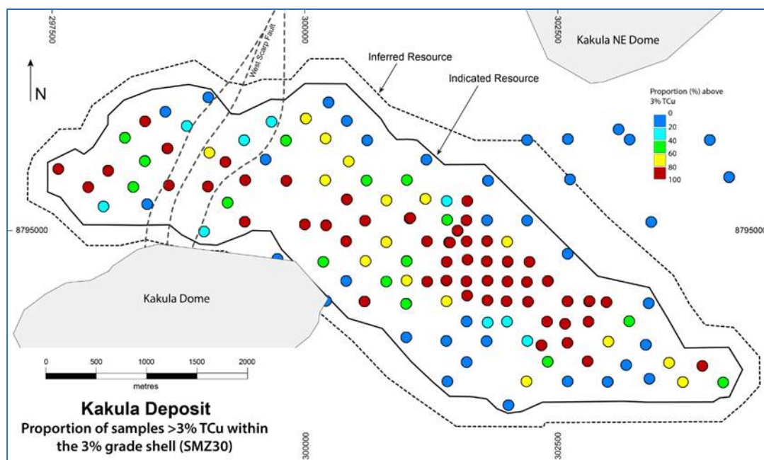
Figure 14.2 Kakula: Proportion of Samples >3% TCu Within the 3% Grade Shell
