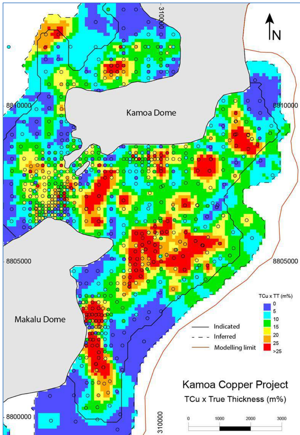
Figure 14.26 Kamoā: Estimated TCu Multiplied by True Thickness (TCu \times TT, m%) for a 1.0% TCu Modelling Cut-off (SMZ10)
