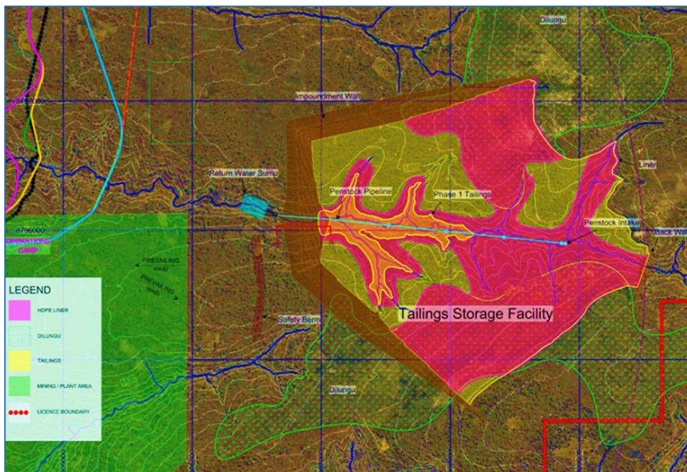
Figure 24.37 Kakula TSF Layout
