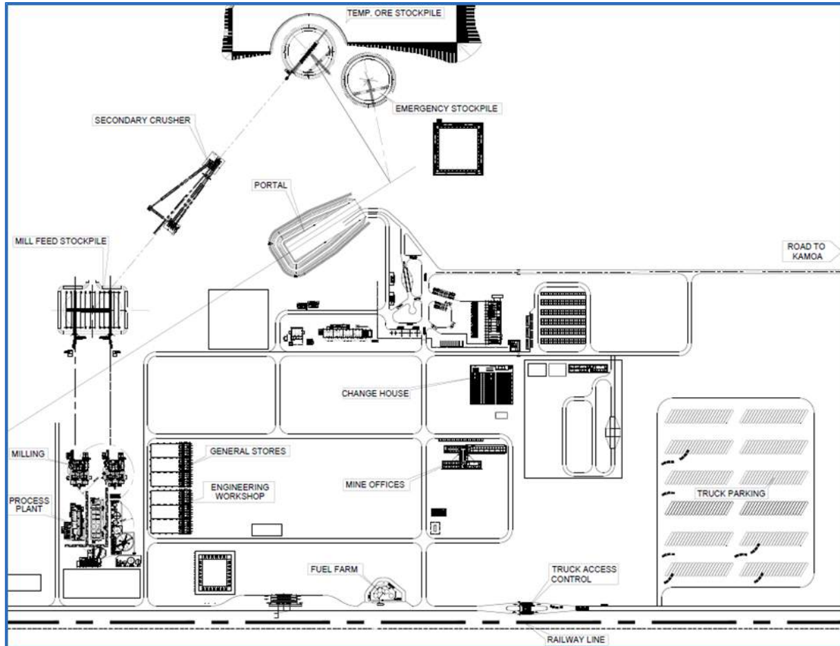
Figure 24.34 Kakula Site Conceptual Concentrator
