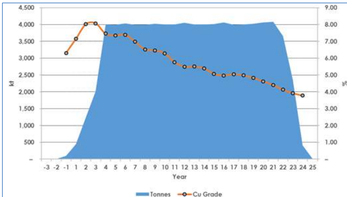
Figure 24.15 Kakula Mine Production
