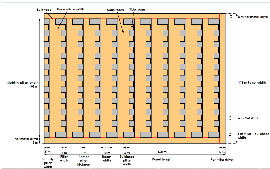
Figure 24.29 Room and Pillar with Hydraulic Fill Panel Layout
