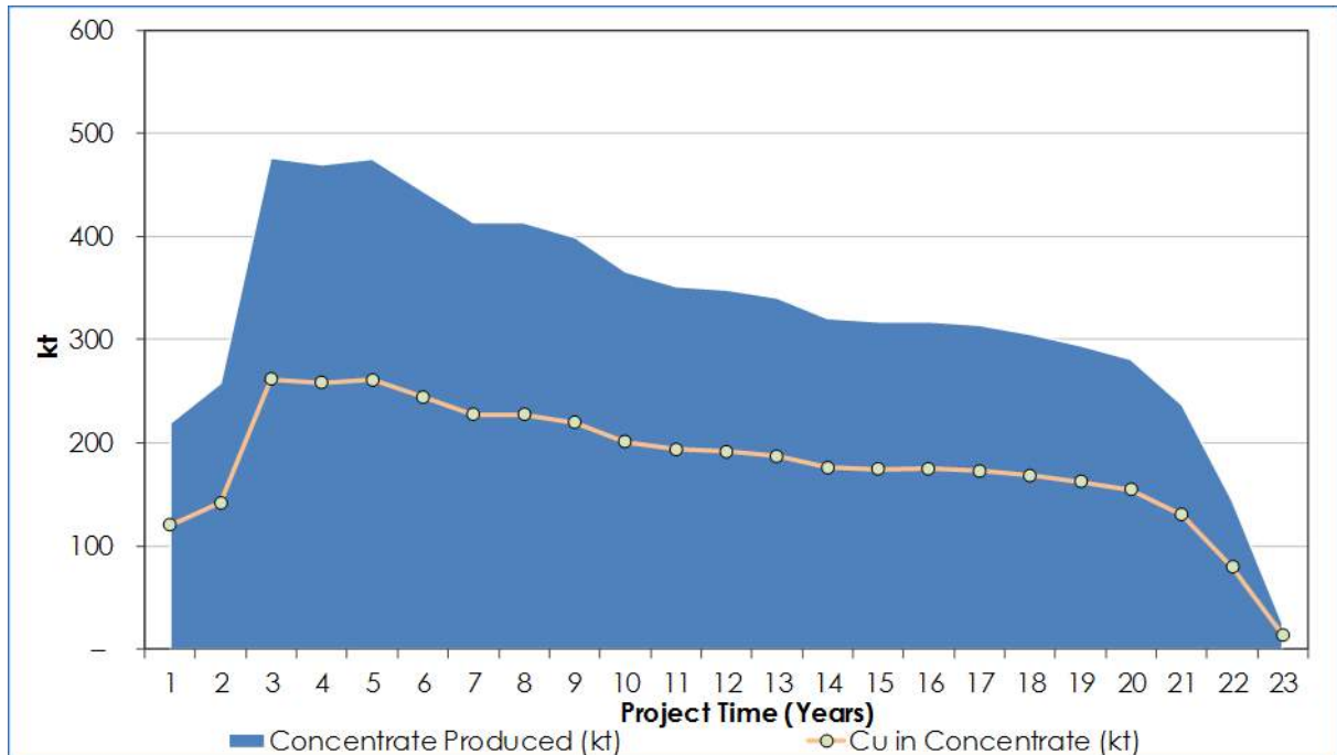
Figure 1.6 Concentrate and Metal Production – 4 Mtpa Production Scenario
