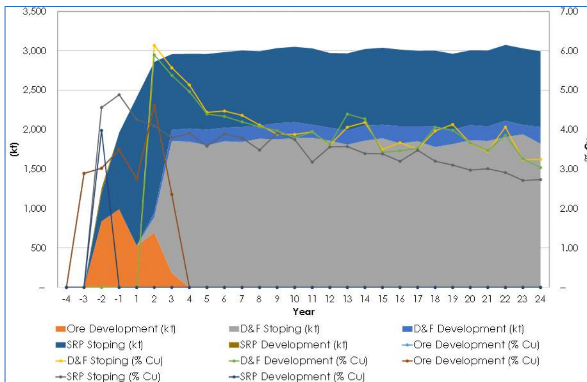
Figure 16.21 Kamoā 2016 PFS Mining Production by Source
