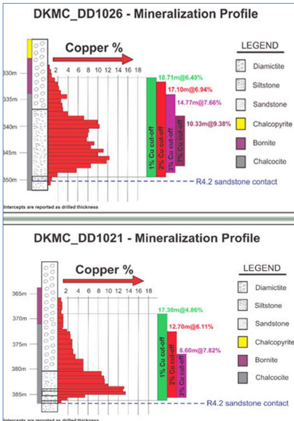
Figure 13.29 Kakula Mineralisation Profiles
