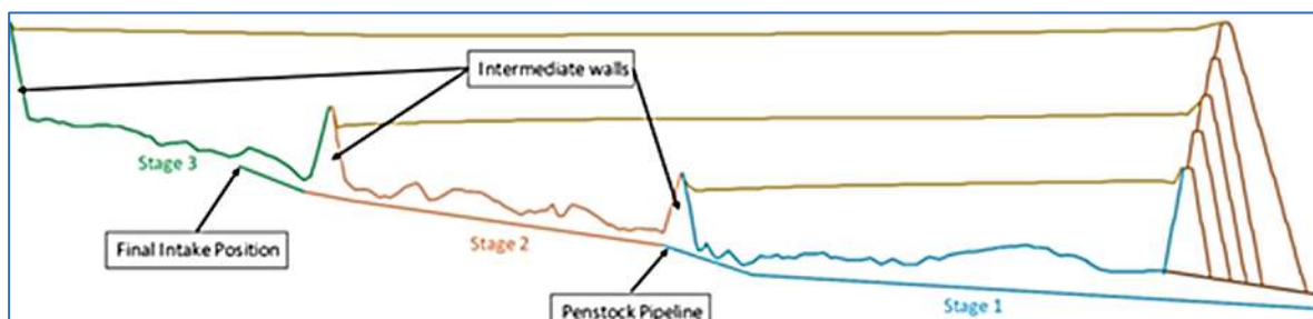
Figure 18.12 Cross-Section through Penstock Pipeline Indicating the Penstock and Liner Staging
