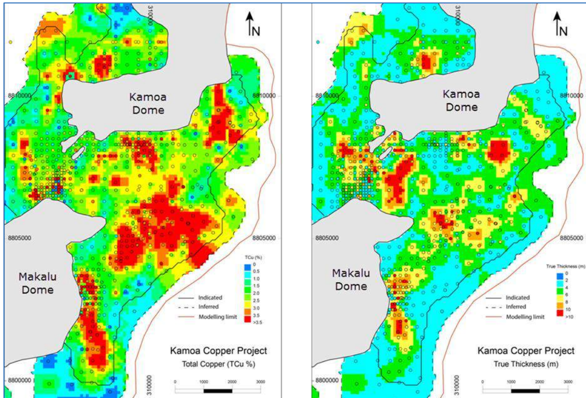
Figure 7.43 2014 Mineral Resource Model for TCu Grade and True Thickness
