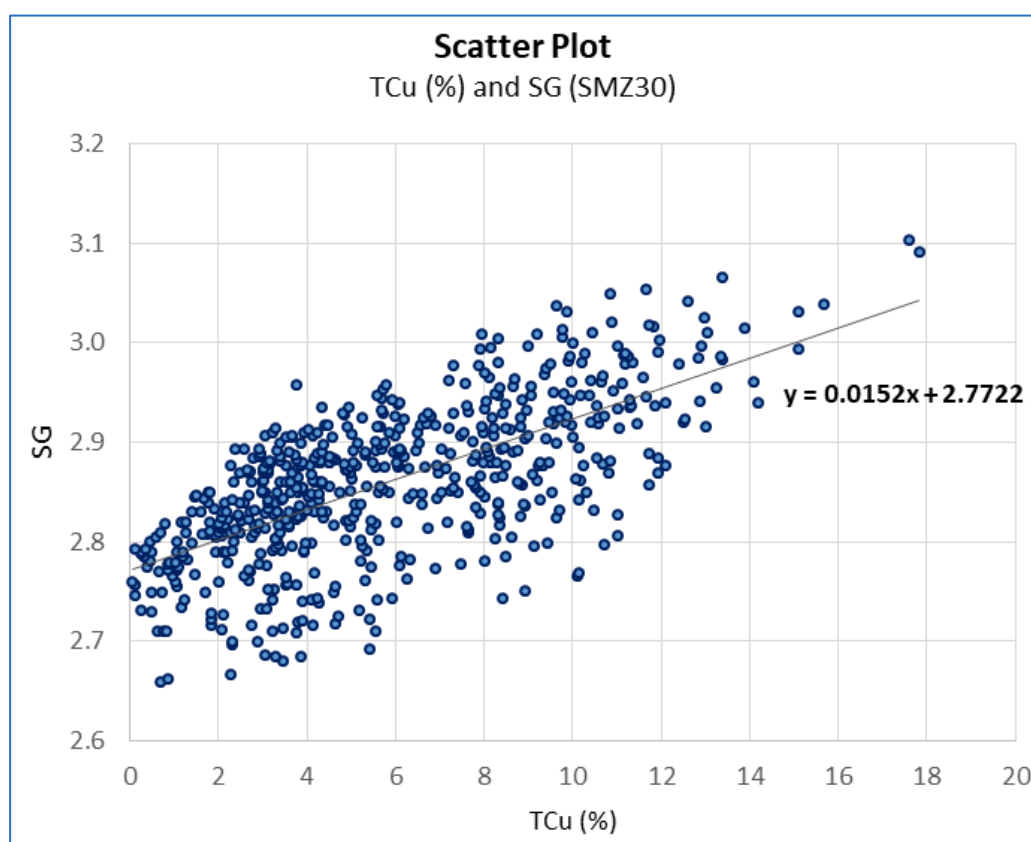
Figure 14.17 Kakula Scatter Plot of Total Copper (%) and SG Values for the 3% TCu Grade Shell (SMZ30), with Outliers Removed
