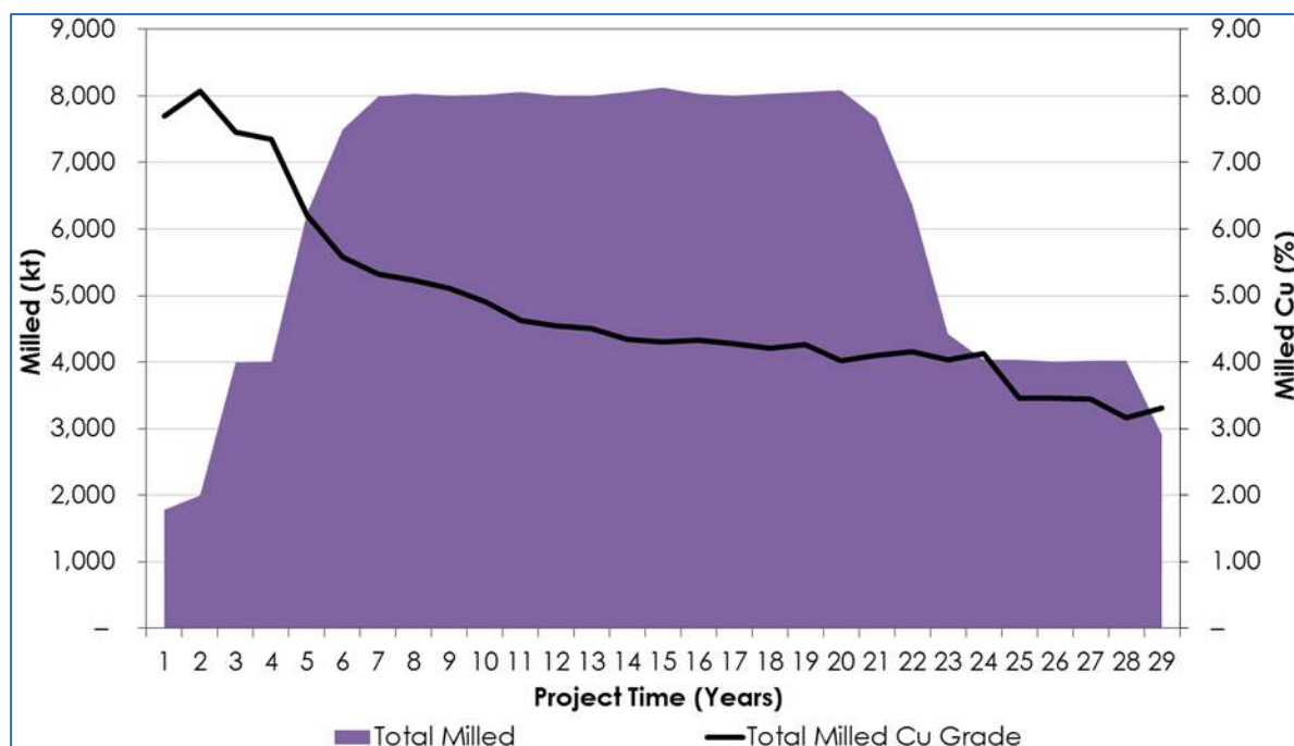
Figure 24.24 Kakula 2016 PEA – Total 8 Mtpa Processing
