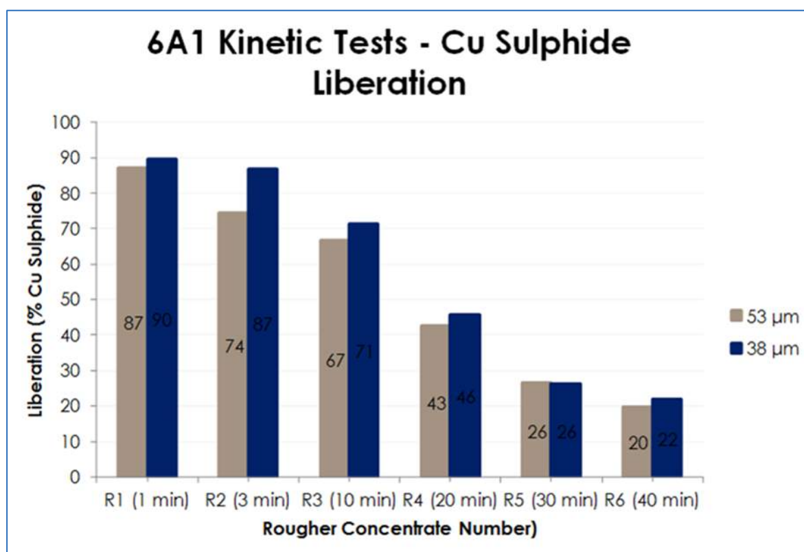
Figure 13.22 Copper Sulphide Liberation in Rougher Flotation
