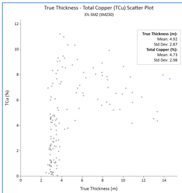
Figure 14.15 Kakula: Scatter Plot of TCu (%) Versus True Thickness (m) for the 3% TCu Grade Shell
