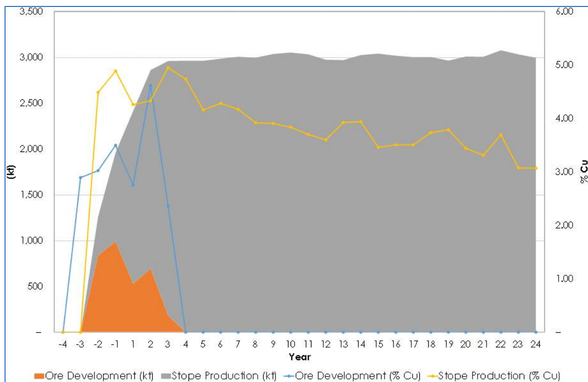
Figure 16.22 Kamoā 2016 PFS Mining Production
