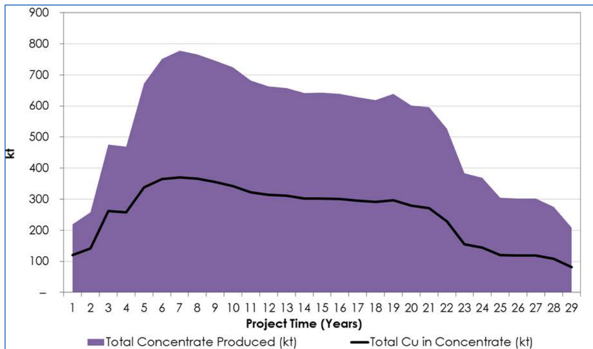
Figure 24.25 Kakula 2016 PEA – Total Concentrate Produced
