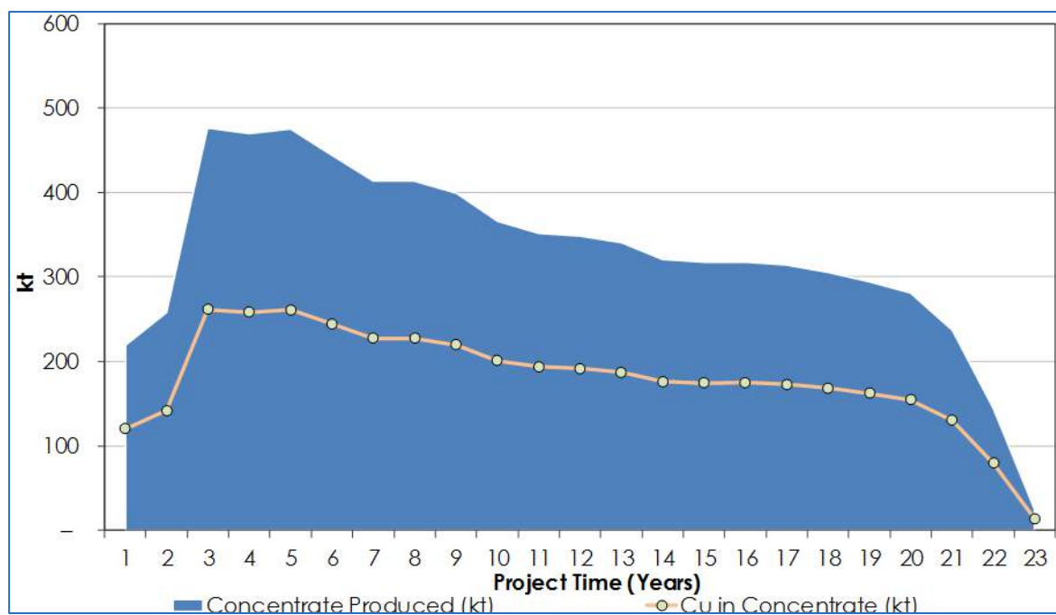
Figure 24.5 Concentrate and Metal Production – 4 Mtpa Production Scenario
