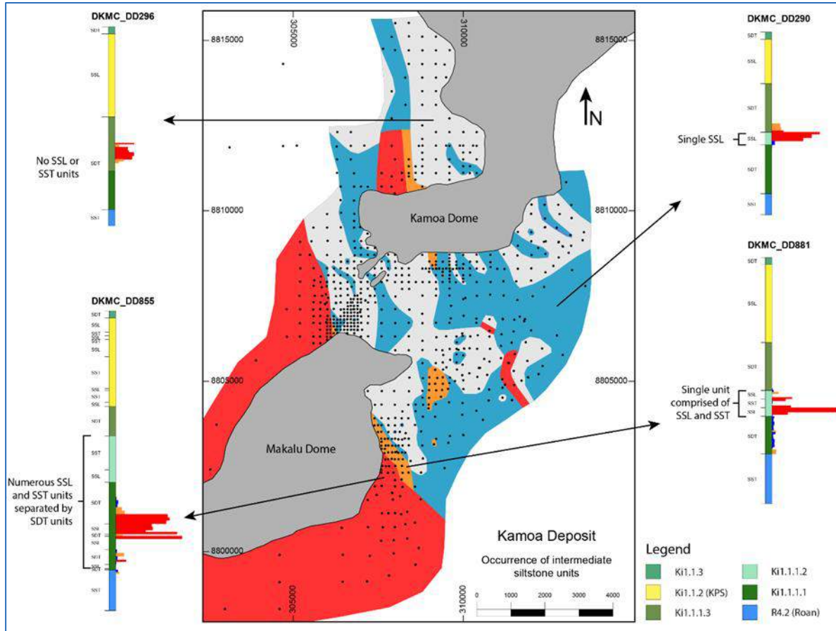
Figure 7.14 Occurrence of Ki 1.1.2 Intermediate Siltstone Units within the Ki 1.1.1
