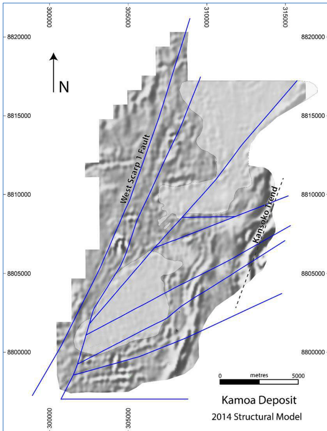
Figure 7.18 Structural Model Overlaid on Second Vertical Derivative Magnetic Image
