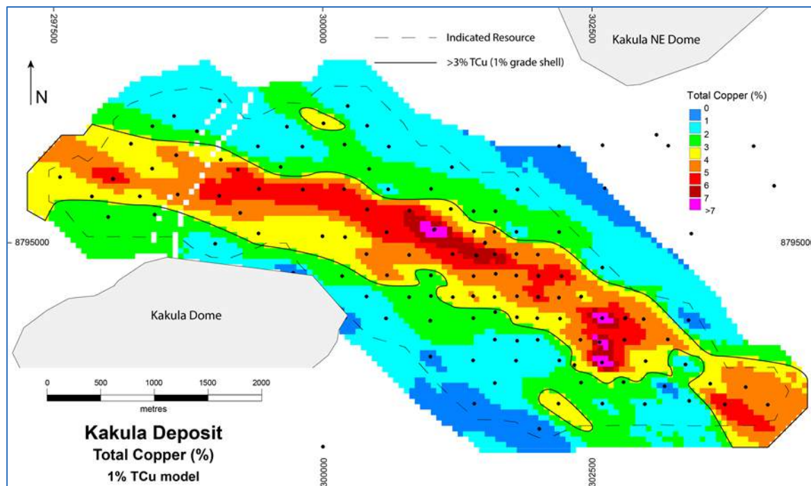
Figure 14.37 Kakula: TCu Grades for the Overall 1.0% TCu Model
