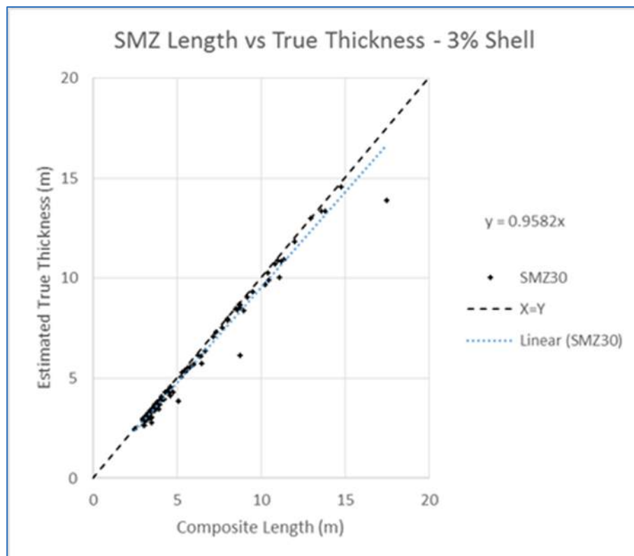
Figure 10.4 Kakula Drillhole Intercept Length versus Estimated True Thickness
