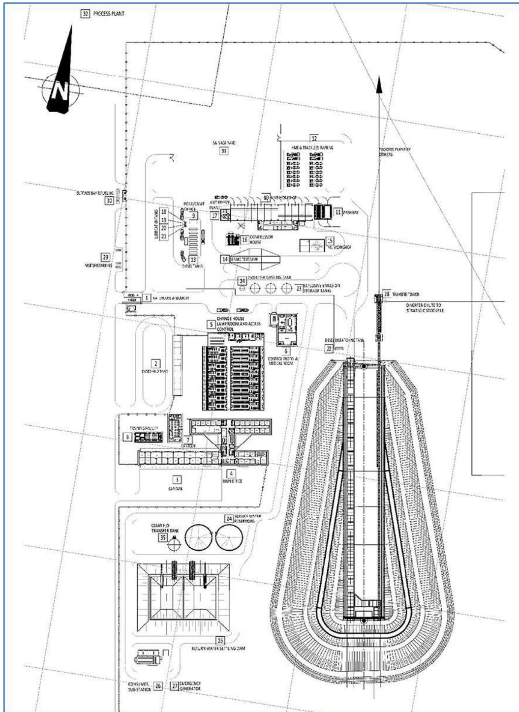
Figure 16.12 Portal Position in Relation to Surface Infrastructure
