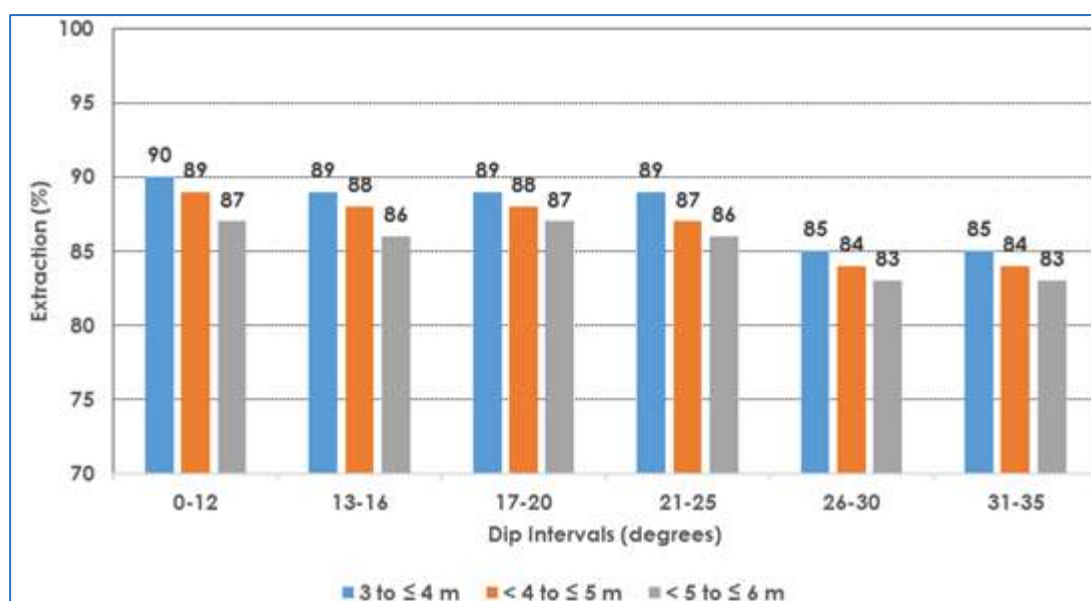
Figure 24.27 Controlled Convergence in Panel Extraction
