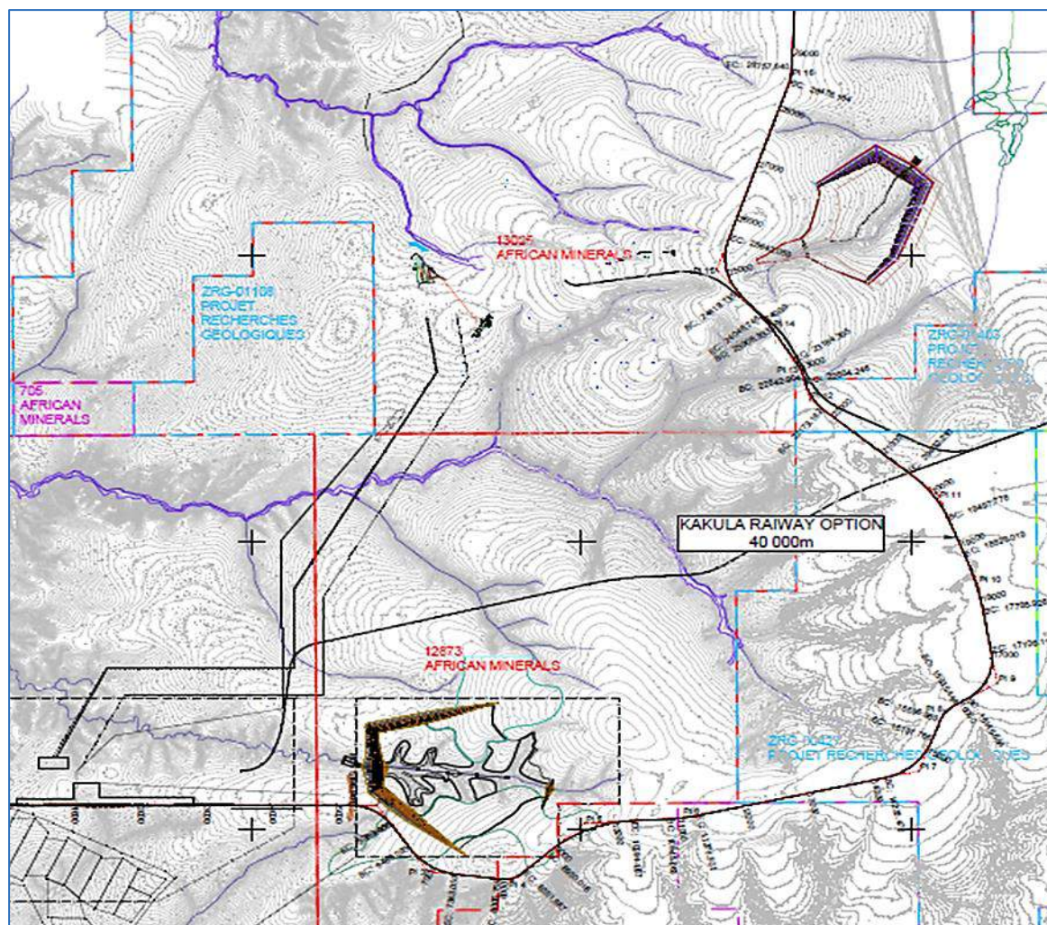
Figure 24.39 Rail from Kakula and Kansoko to existing Lobito infrastructure
