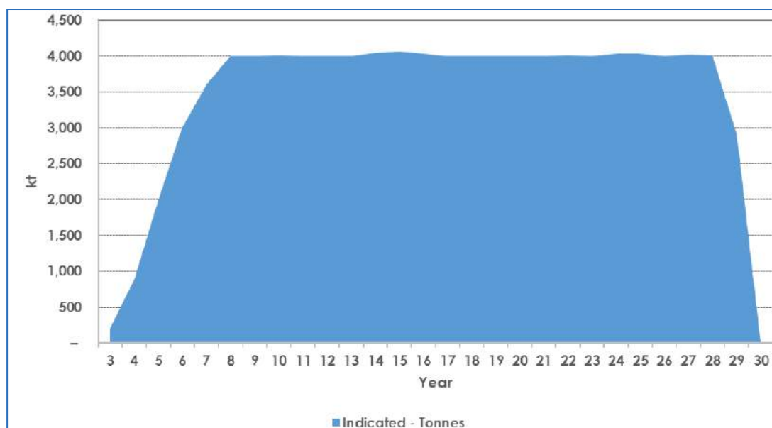
Figure 24.19 Kansoko Mine Production by Resource Category
