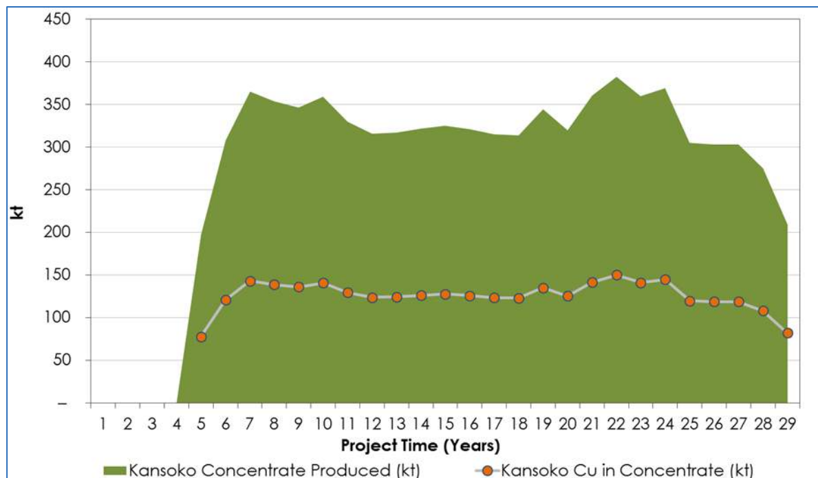
Figure 24.23 Kansoko Concentrate Produced
